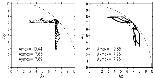
Figure 2: Secondary halo images in the amplitude plane before (left) and after (right) minimization for the lattice of IR3 in [1]
