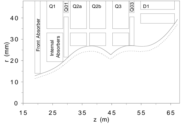
Figure 1: The LHC low- \beta insertion including absorbers which reach the 10\sigma limit (injection/collision optics: solid/dashed line) for d_{coil}=70 mm quadrupoles.
