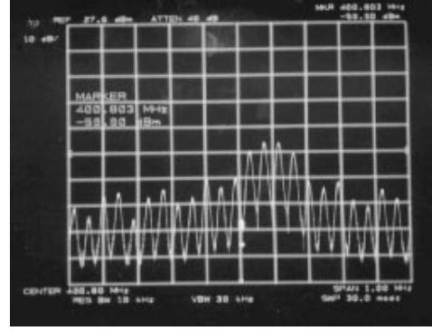
Figure 5: Spectrum at beginning of 450GeV flat top, the cavity resonance is at the centre of the screen.
