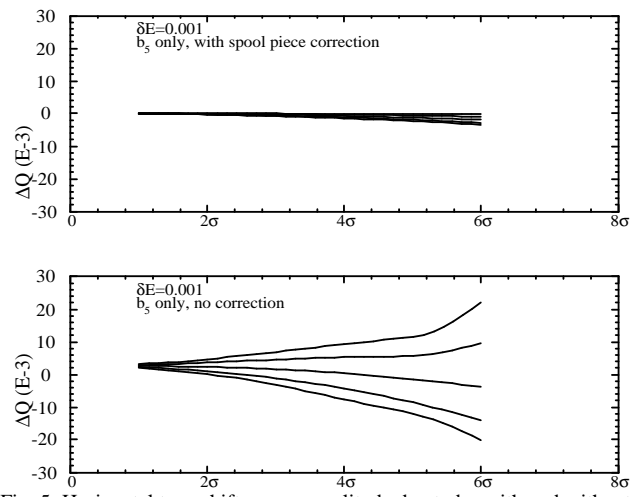
Fig. 5: Horizontal tune shift versus amplitude due to b_5 , with and without correction by spool pieces in magnet ends. Each line corresponds to a different ratio of horizontal to vertical amplitude
