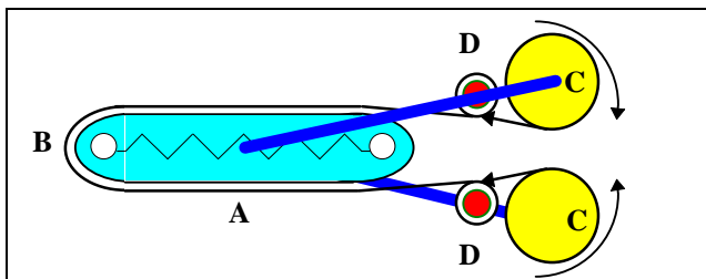
Figure 2. Winding A: Pre-compressed central island B: Layer jump C: Wire reels D: Counter bending pulleys
