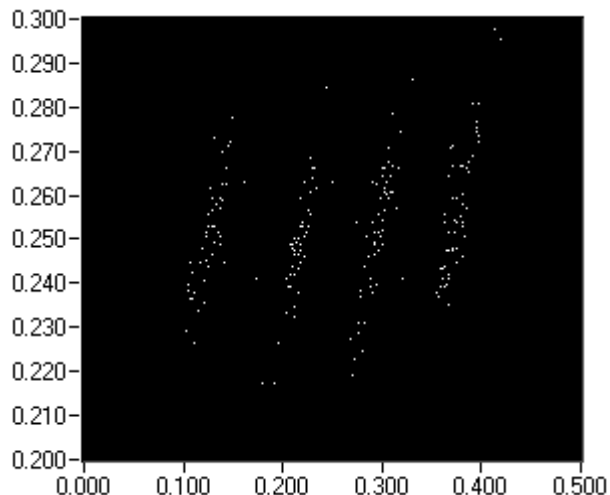
Figure 6: Correlated output with three 50 \mu\text{m} steps.
