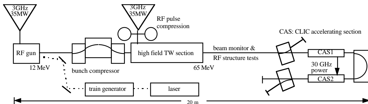
Figure 1. Schematic layout of CTF as it was in 1995
