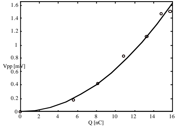
Figure 3. Bolometer output signal as a function of the total charge in the train.
