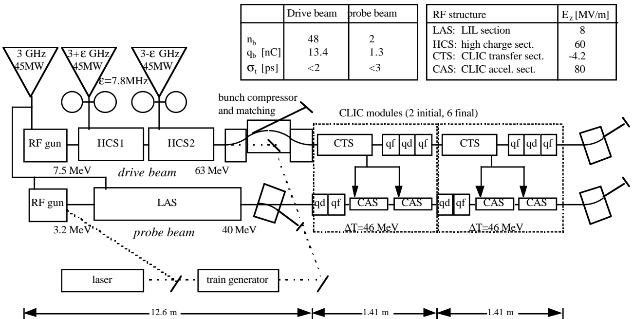
Figure 4. Sketch of CTF2. BPM's and focusing is omitted, except of the quadrupoles in the CLIC modules. the phase change from bunch to bunch compensates for the field reduction due to beam loading. This scheme for
