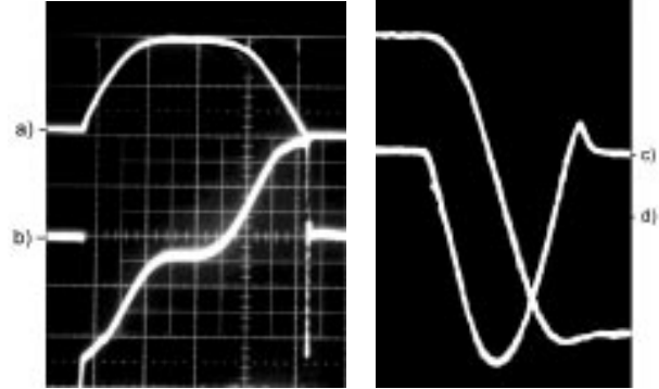
Fig 4: Wave shapes recorded during tests: S1-S2 at 9 kA: a) Magnet current (5 kA/d-0.5 ms/d); b) Transformer primary voltage (0.8 kV/d). S3 at 8 kA: c) Magnet current (2 kA/d-20 \mu\text{s} /d); d) Capacitor voltage (0.5 kV/d)
