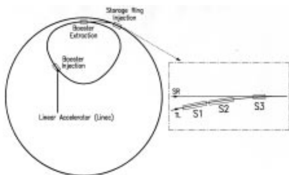
Fig.1: ESRF complex and SR injection layout.
