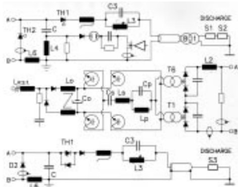
Fig.3: Electrical diagram of power converters
