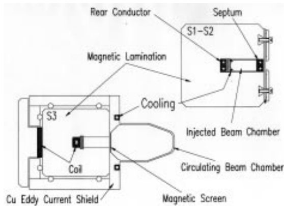
Fig.2: Cross-section of S1-S2 and S3 magnets
