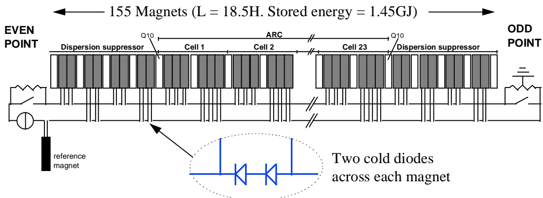
Figure 2 Main Dipole Circuit for One Sector (1/8) of LHC
