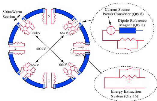
Figure 1 Segmentation of Main Dipoles
