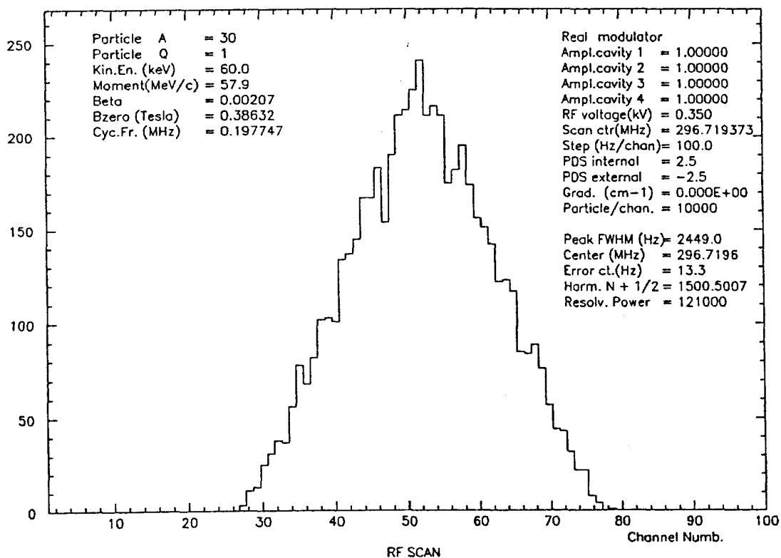
Figure 3. Multi-particle simulation for A = 30 : the resonance peak exhibits a resolving power of 1.2 \cdot 10^5 and a transmission for the central frequency of 2 \cdot 10^{-2} , in the discussion, in order to be conservative, a resolving power of 10^5 and a transmission of 10^{-2} have been considered.
