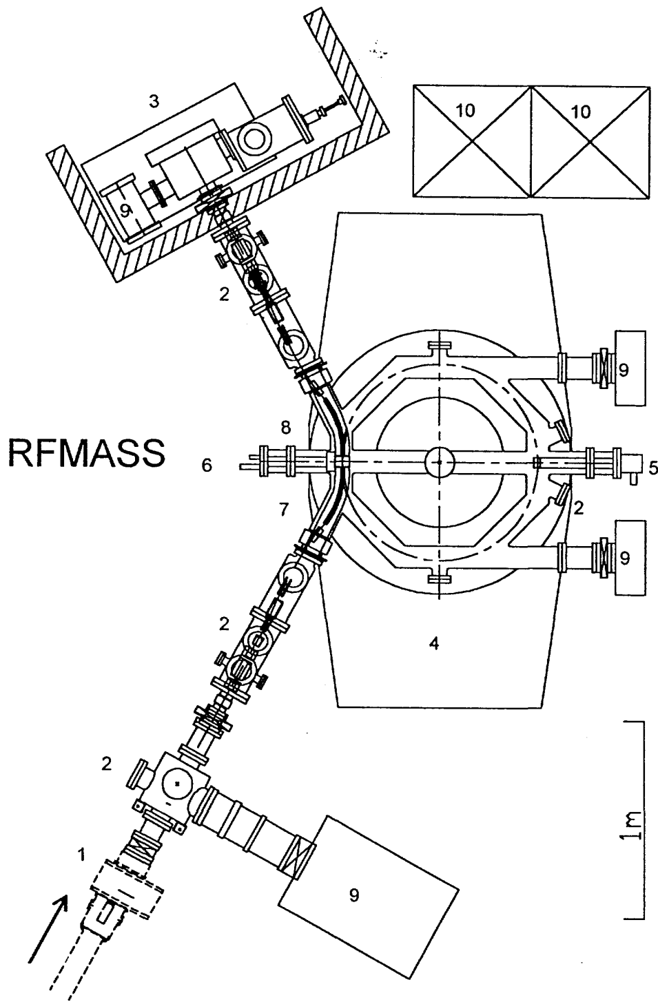
Figure 4. Layout of the RFMS:
