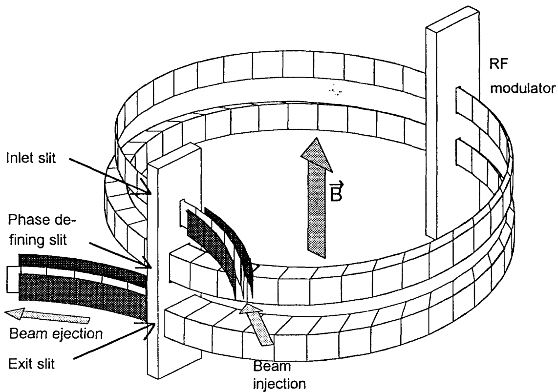
Figure 2. Principle of the RFMS. \vec{B} indicates the very homogeneous magnetic field.
