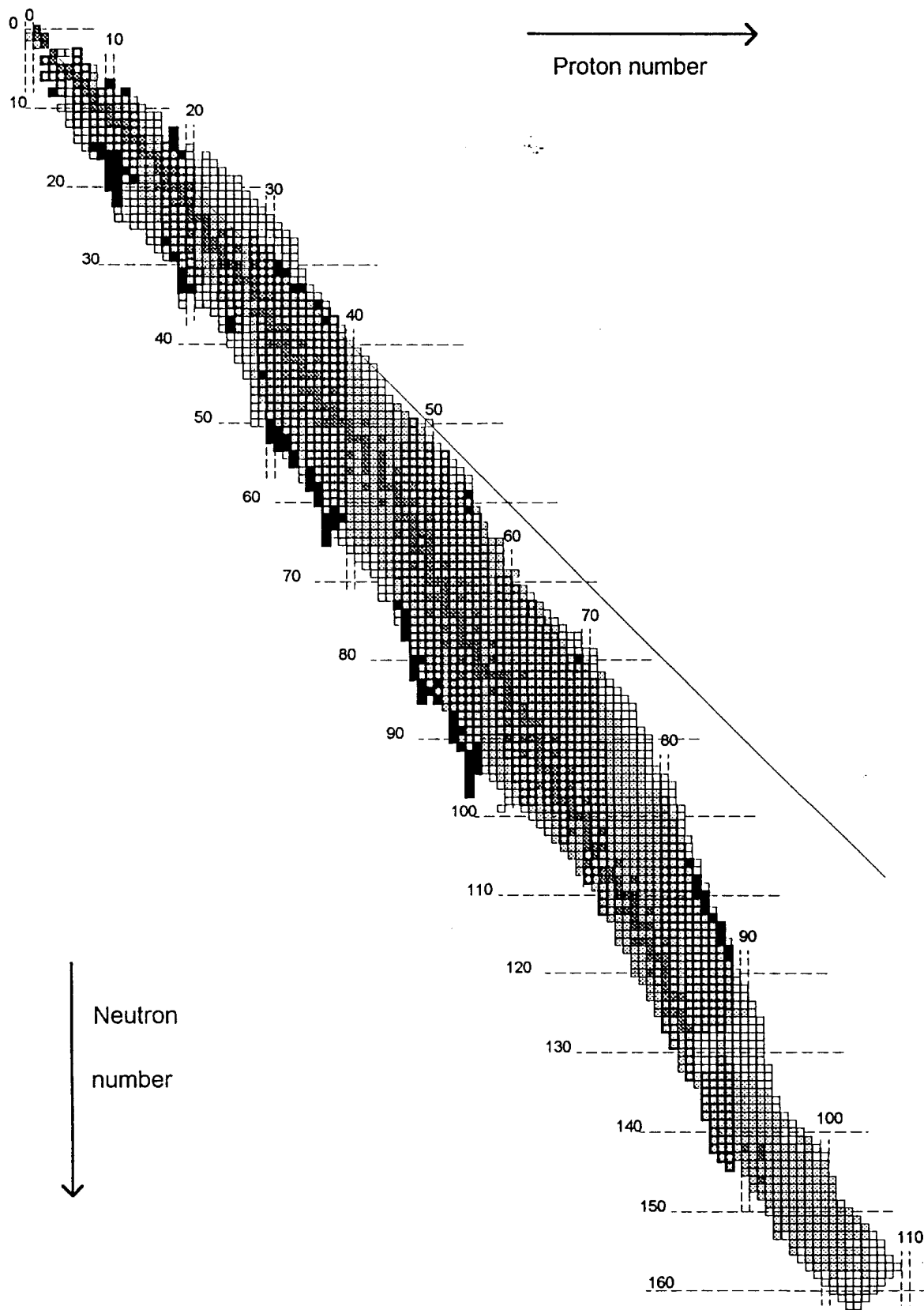
Figure 1. Chart of the nuclides displaying:
