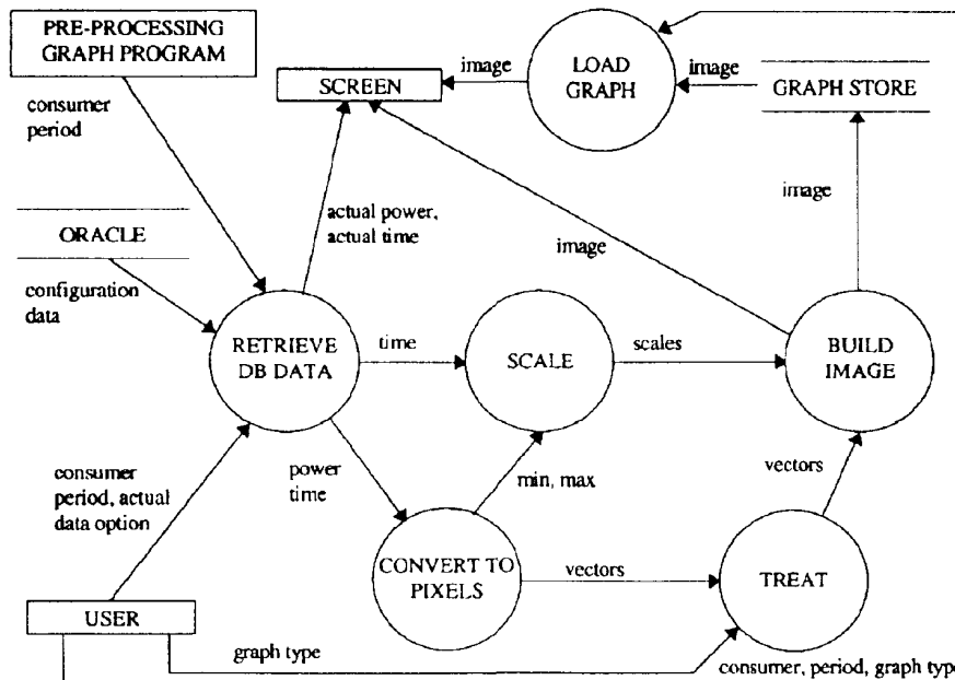
FIGURE 1: Data flow diagram for graph selection, production and display
