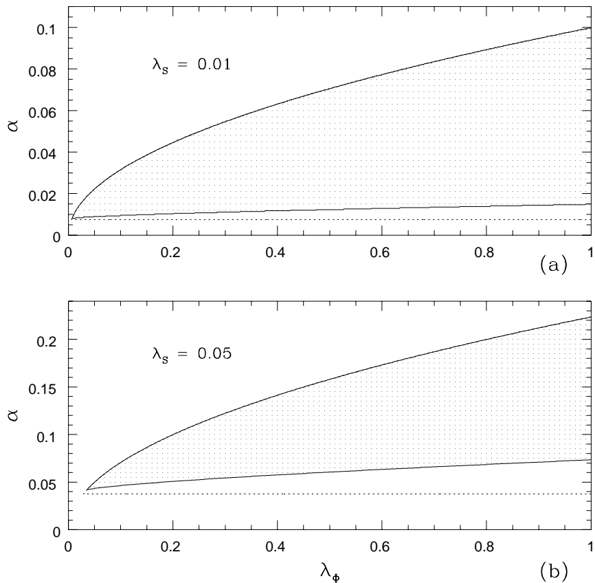
FIG. 2. The region of symmetry nonrestoration for the model of \mathcal{CP} with a real, CP odd singlet, for two values of the singlet's self coupling constant \lambda_s as indicated. When only leading order effects are taken into account, the region extends up to the dotted line
