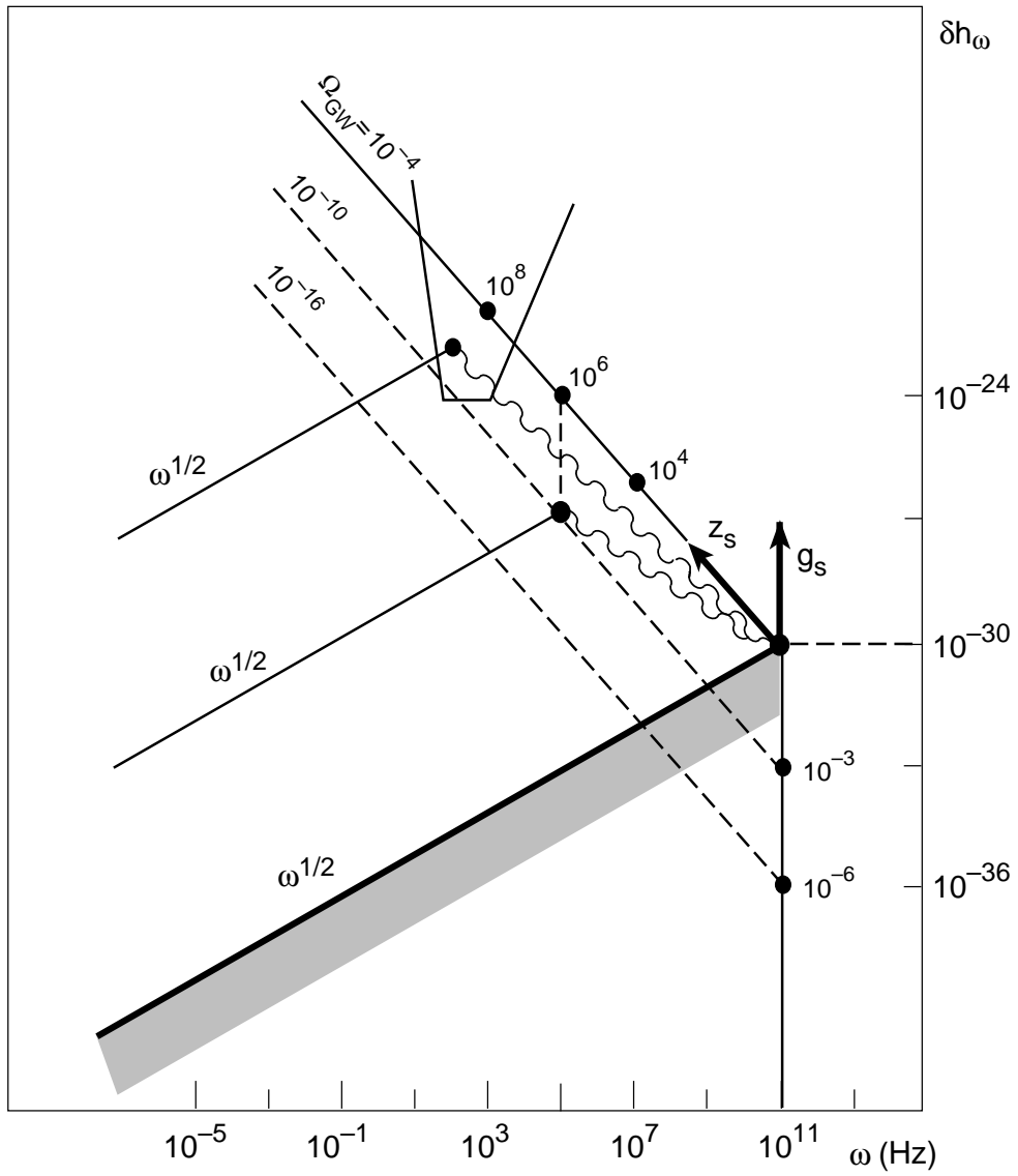
Figure 3: GW spectra from string cosmology against interferometric sensitivity.
