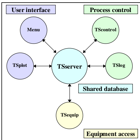
Fig 2. Software layout.
