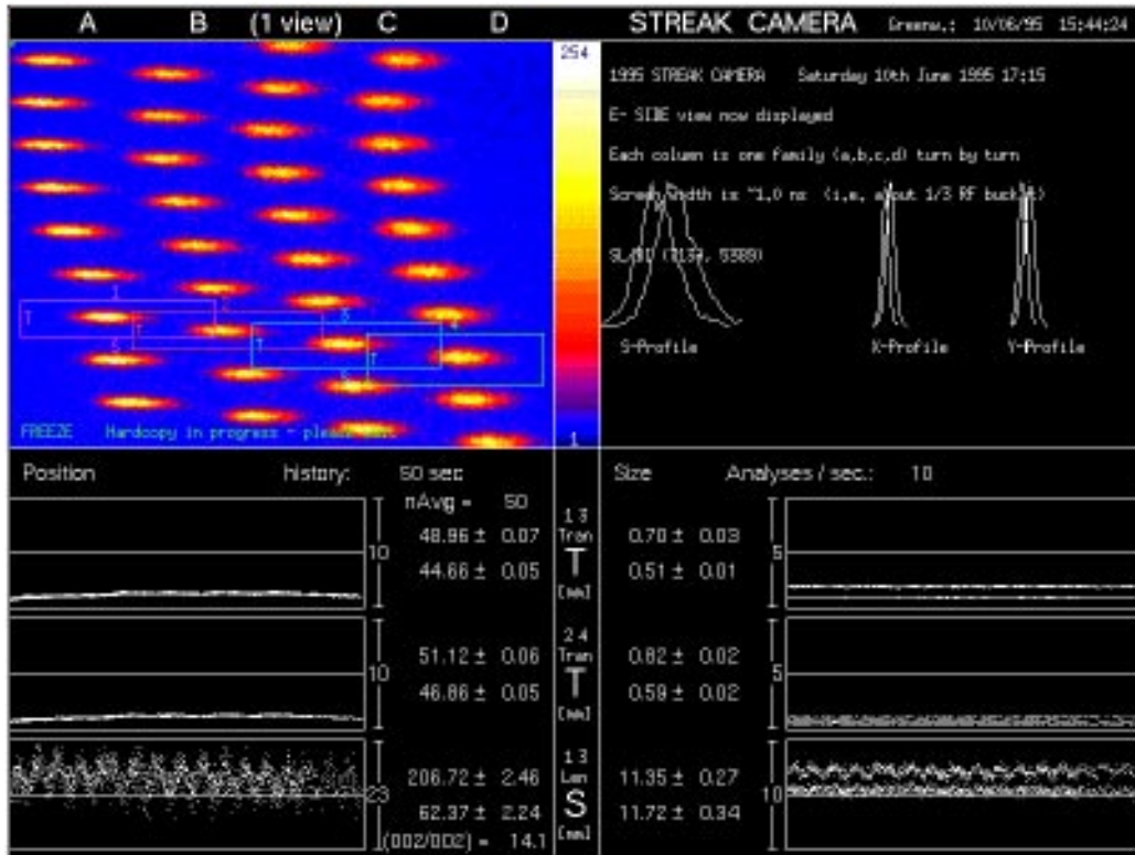
Figure 7 : High resolution video display transmitted to LEP control room
