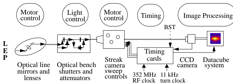
Figure 1 : Principal streak camera subsystems
