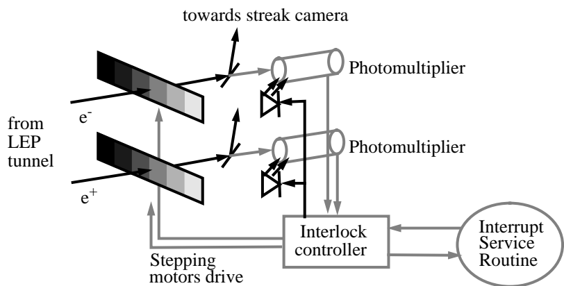
Figure 2 : Synchrotron light intensity control
