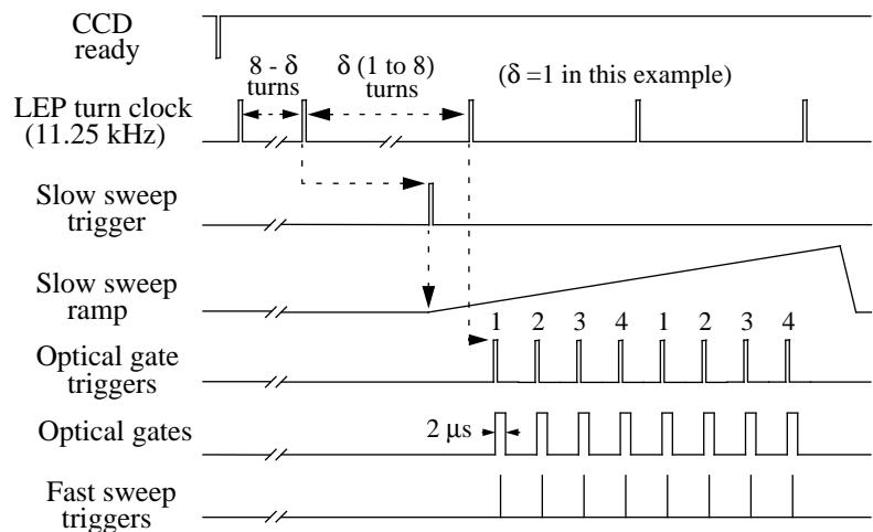
Figure 4 : Example of generation of triggers to measure 4 bunches on 2 consecutive LEP turns
