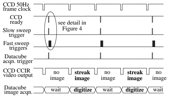
Figure 3 : Synchronisation of streak camera, CCD camera and Datacube system
