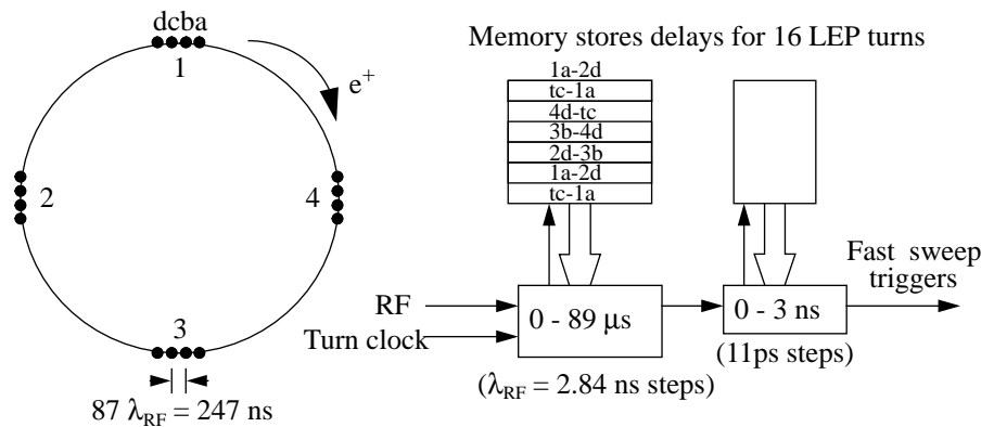
Figure 5 : Picosecond timing for bunch selection
