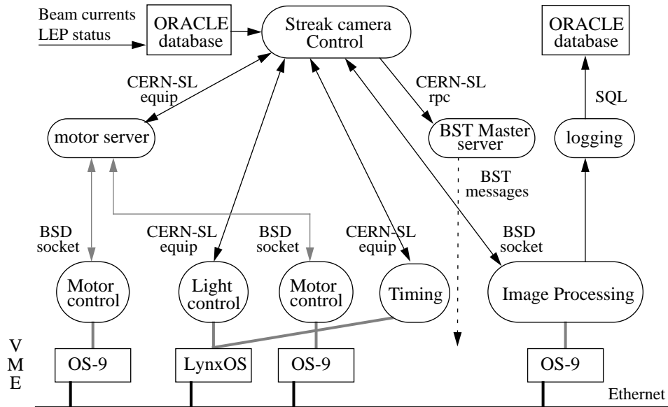
Figure 8 : Streak camera control architecture
