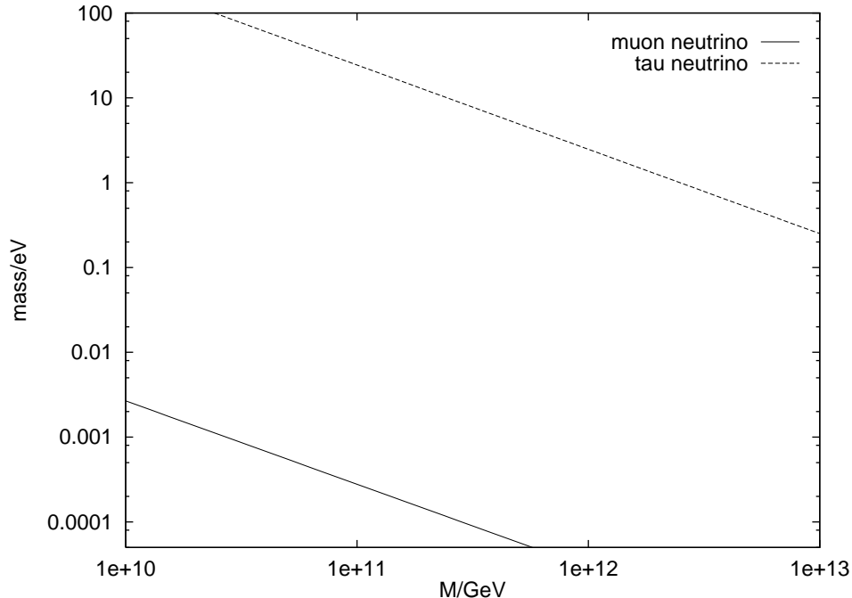
Figure 1: Dependence of m_{\nu_\tau} and m_{\nu_\mu}/l_N^2 upon M for \alpha_S(M_Z) = 0.11 , m_b = 4.25 GeV. Since the muon neutrino mass is scaled by 1/l_N^2 , the MSW bounds upon it implied by Eq.69 must also be scaled by this number. Thus, these bounds are dependent upon the choice of heavy ansatz A_i if applied to the figure.
