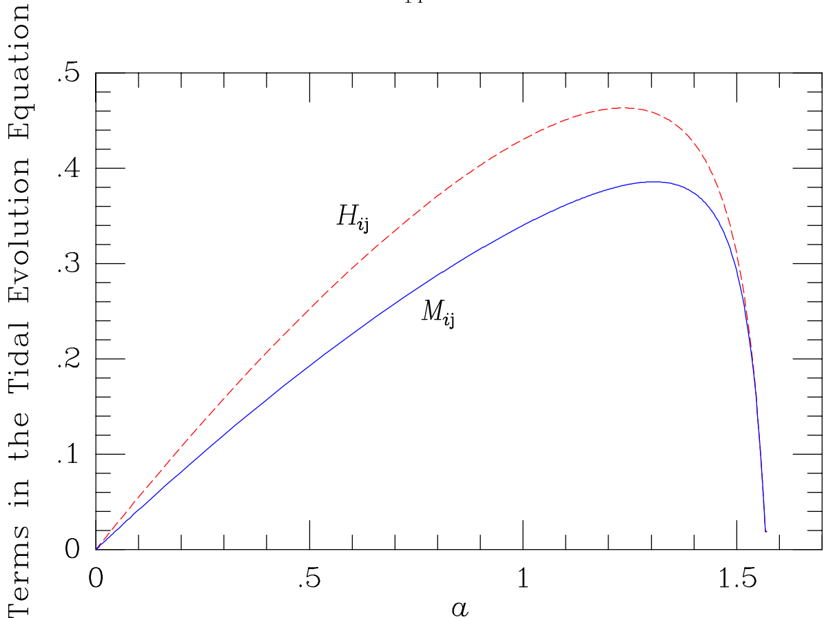
Fig. 1.— Evolution of the magnitudes of -\nabla_k \epsilon^{kl} ({}_{(i}H_{j)l} (dashed line) and M_{ij} (solid line) divided by the magnitude of 4\pi Ga^2 \rho \sigma_{ij} , evaluated for a homogeneous ellipsoid with initial axis ratios 1 : 1.25 : 1.5 embedded in an expanding universe. The magnitude of a matrix is defined here as the square root of sum of squares of eigenvalues.
