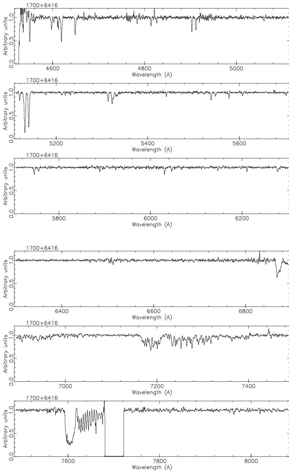
Fig. 1. Normalized spectrum of HS 1700+6416
