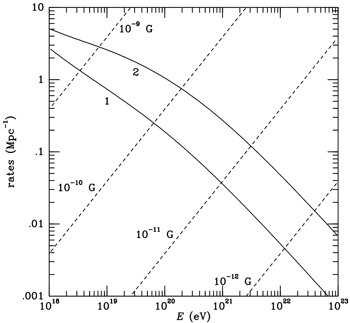
Fig. 1.— The rate of inverse Compton scattering (ICS; solid lines) and the fractional synchrotron loss rate (dashed lines) for different magnetic fields as functions of energy. 1 is for a frequency cutoff at 2 MHz in the diffuse radio background, and 2 is for 0.5 MHz, respectively.
