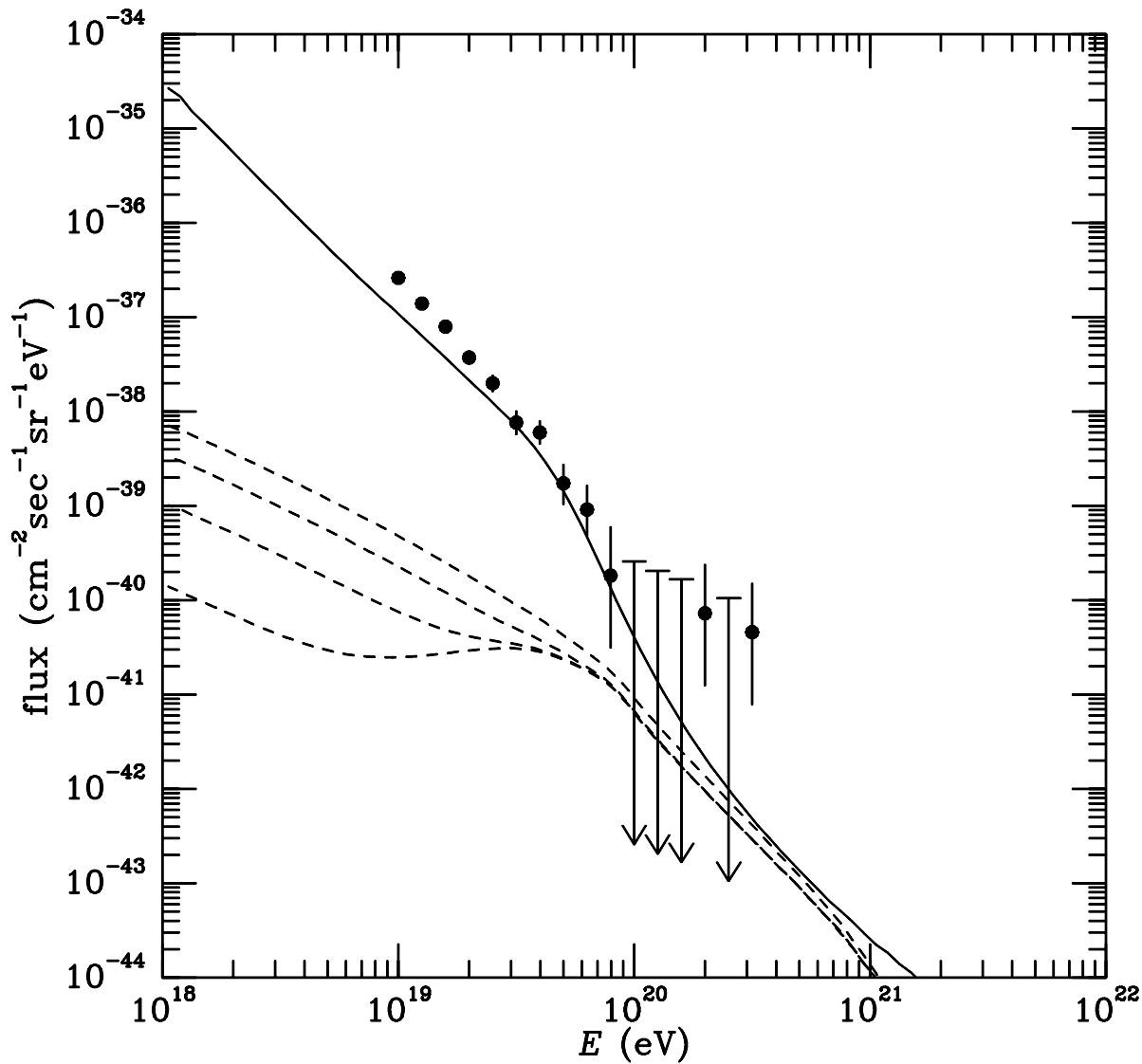
Fig. 3.— Cosmic ray nucleon spectrum (solid line), and secondary \gamma -ray spectra (dashed lines) for a continuous source distribution up to 1Gpc distance whose comoving density scales as (1+z)^2 . The sum of the nucleon and \gamma -ray flux is fitted to the combined data from the monocular Fly’s Eye (Bird et al. 1994) and the AGASA experiment (Yoshida et al. 1995). Shown are 1\sigma error bars, and 84% confidence level upper limits. The magnetic field values are the same as in fig. 2.
