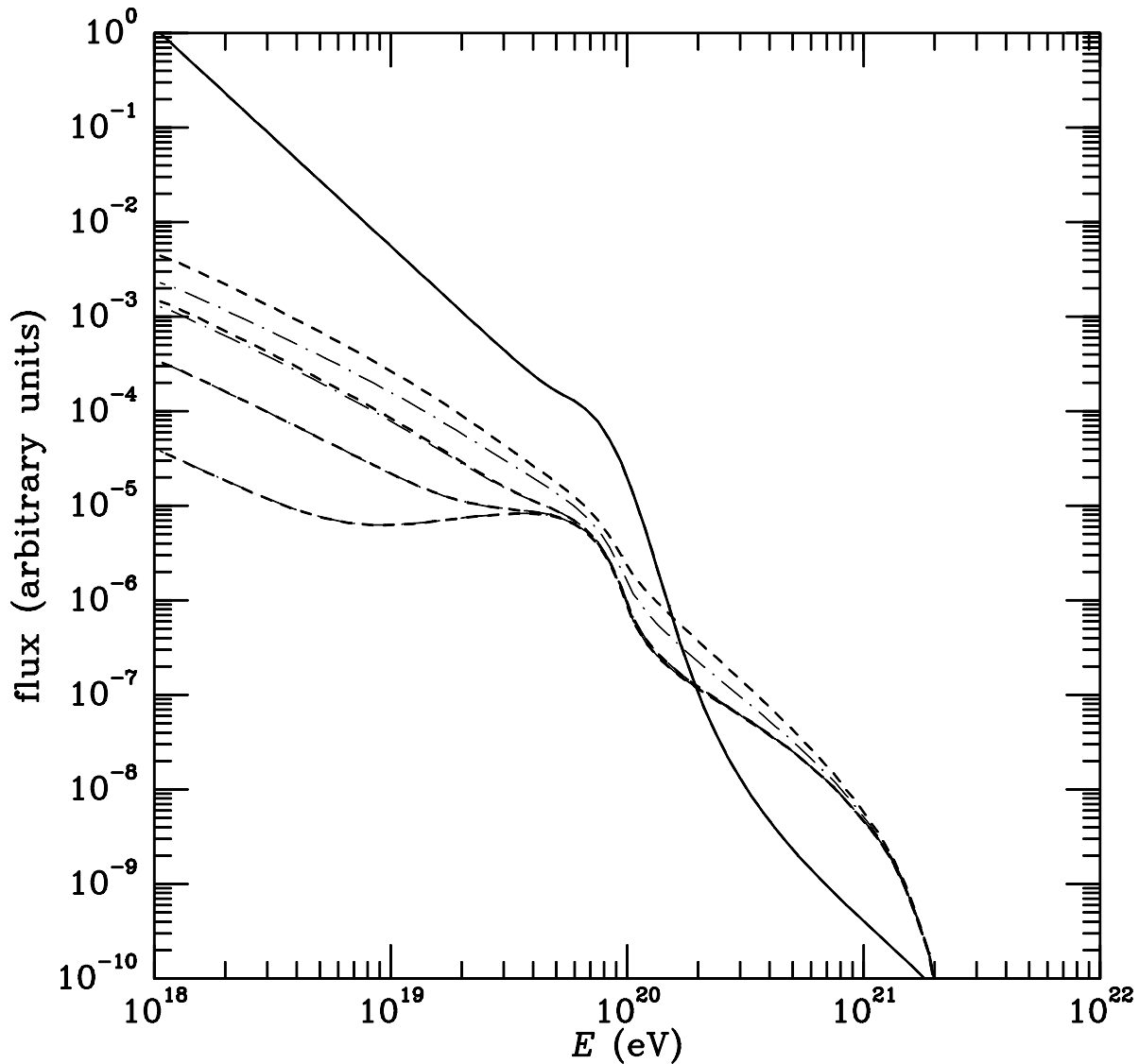
Fig. 2.— Cosmic ray nucleon spectrum (solid line) from a single source at a distance of 30 Mpc, and secondary \gamma -ray spectra for different magnetic fields. The short dashed lines are with no intervening objects, and the long dashed lines with dots are with a 5 Mpc sized object located at 12.5 Mpc from the observer. The magnetic field values are B = 0, 10^{-10}, 3 \times 10^{-10}, and 10^{-9} G, respectively from the top.
