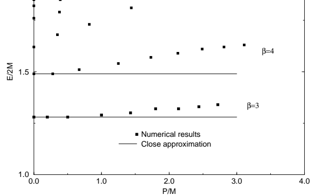
FIG. 2. The ADM energy of initial data for collisions of black holes of momenta P . The dots are the full numerical results of Cook, for different values of the initial separation \beta . We see that for small separations, the energy is approximately independent of the holes momenta, which coincides with the close approximation prediction, depicted by the solid line.
