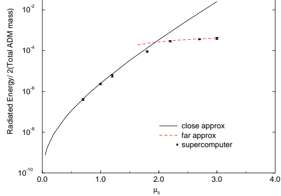
FIG. 1. Comparison of results for the radiated energy vs initial separation in a collision for the close approximation, the fully numerical results and the far approximation. Vertical scale is logarithmic.
