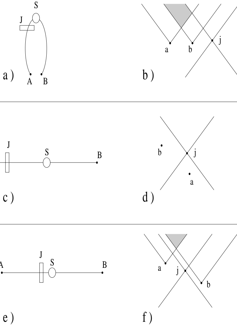
Figure 1: The geometrical configurations showing the source S of pairs of quantum systems, the jammer J , and the experimenters Alice A , and Bob B . (a) A and B are close to each other while J is far from both of them. (c) A and J are close to each other while B is far from both of them. (e) A , B and J are all far from each other; J is stationed near the source and A and B are at opposite ends of an EPR-Bohm setup. Corresponding Minkowski diagrams showing the events a , b and j . (b) The future light cones of a and b have some overlap outside the future light cone of j . (d) A possible configuration for selective jamming. (f) A configuration satisfying the binary condition. The future light cones of a and b overlap only within the future light cone of j .
