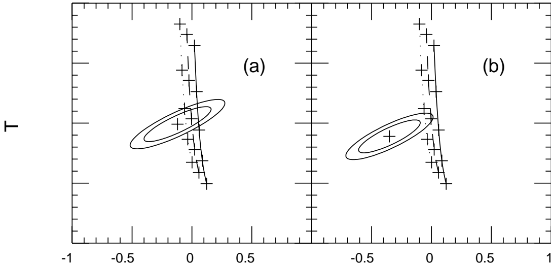
Figure 1: Allowed ranges of S and T at 68% (inner ellipses) and 90% (outer ellipses) confidence levels. Dotted, dashed, and solid lines correspond to standard model predictions for M_H = 100, 300, 1000 GeV. Tick marks, from bottom to top, denote predictions for m_t = 100, 140, 180, 220, and 260 GeV. (a) Fit including APV experiments with present errors; (b) errors on APV experiments reduced by a factor of 4, with present central values of Q_W retained.
