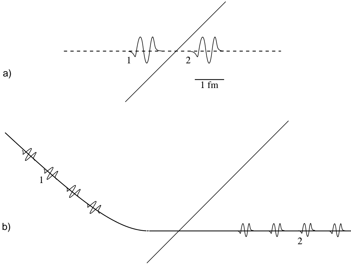
Figure 2: a) Fermi-scale wavepackets just inside and just outside the horizon. b) Subsequent state of several pairs of packets along a nice slice.
