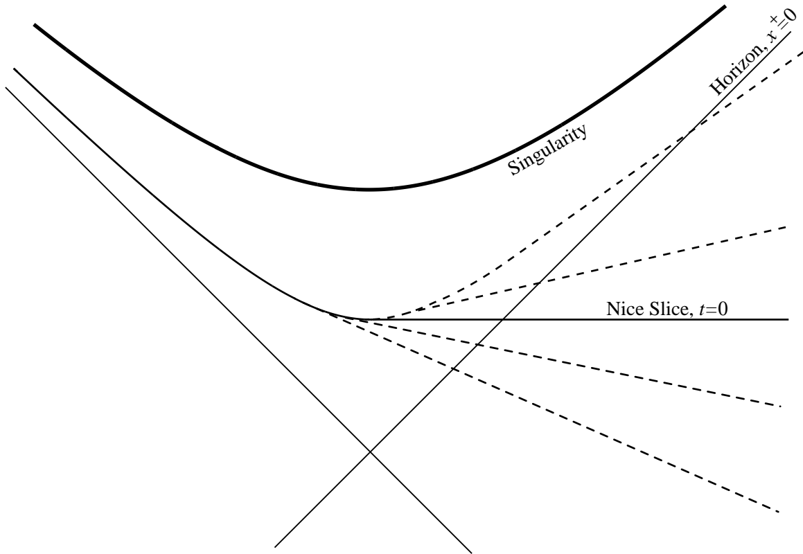
Figure 1: Nice slicing of the Kruskal x^+x^- plane. The slice which is asymptotic to the t = 0 surface is drawn as a solid line, with earlier and later slices shown dashed.
