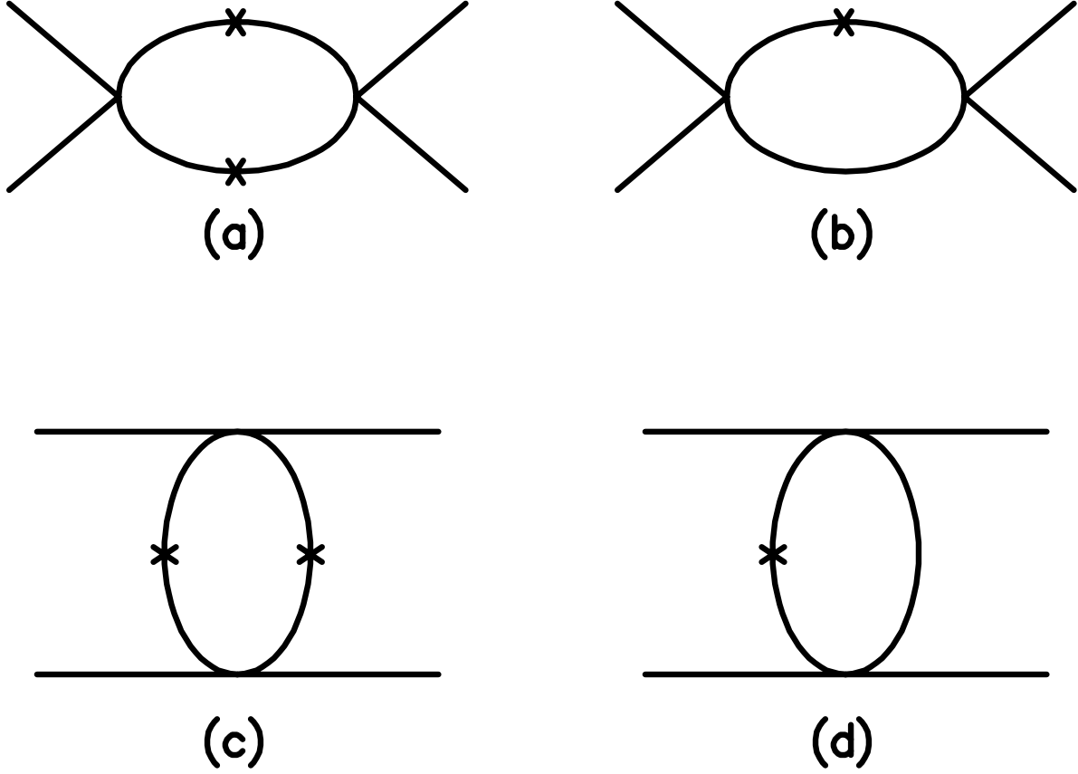
Figure 1. \mu^2 -dependent s -channel (a and b) and t -channel (c and d) contributions to pion-pion scattering. Incoming (outgoing) particles are on the left (right). An internal line with (without) a cross refers to the double (single) pole term in eq. (7).
