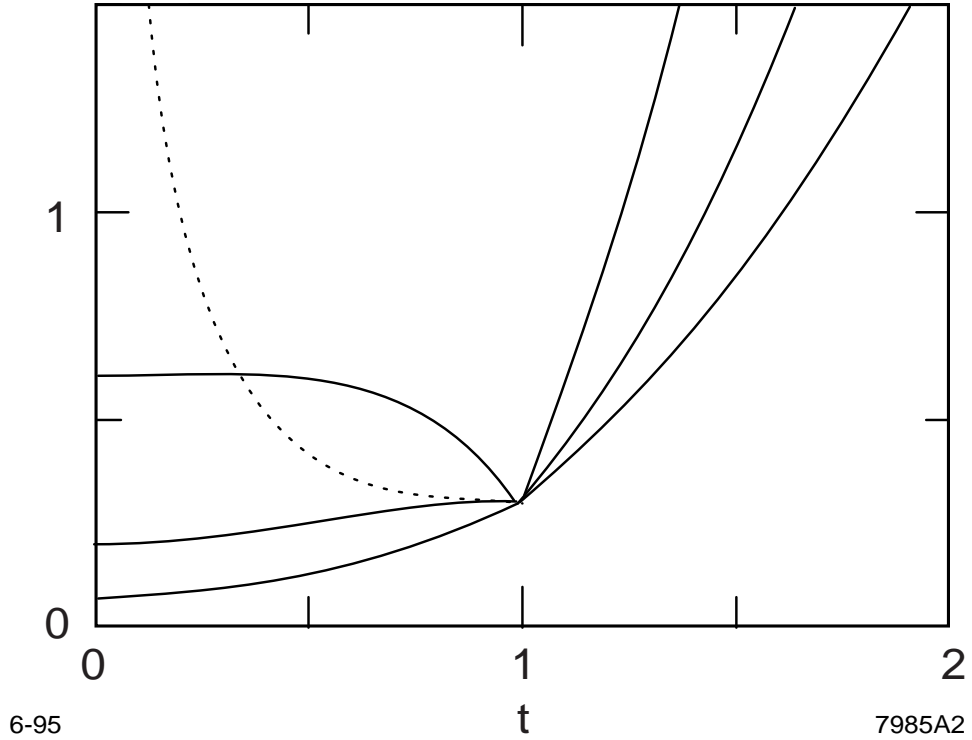
Figure 2: The potential \Delta V for softly broken supersymmetric Yang-Mills theory with N_c = 3 , N_f = 3 . The potential is shown on the subspace T = t \cdot \mathbf{1} , as a function of t . The three curves correspond to (B_B/B_T) = \frac{1}{3}, 1, 3 , from bottom to top. The dotted line shows the location of the stationary point (3) referred to in the text.
