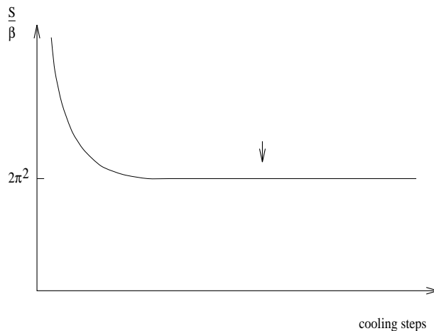
Fig. 1. Cooling history for gauge group SU(2) and a single instanton event. The action for this event is S/\beta = 2\pi^2 .
