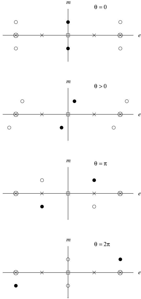
Fig. 3. The electric ( e ) and magnetic ( m ) charge lattice for various values of \theta . The solid circles represent monopoles, crosses represent quarks, crossed circles gluons, open circles monopole-gluon bound states, and the box represents the 'photon'.
