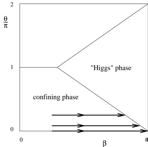
Fig. 5. The phase diagram. The line which starts at \theta = \pi in the strong coupling region and then turns towards \theta = 0 (and \theta = 2\pi , respectively) in the continuum limit is a line of first order phase transitions. The horizontal lines marked by arrows are lines of constant physics.
