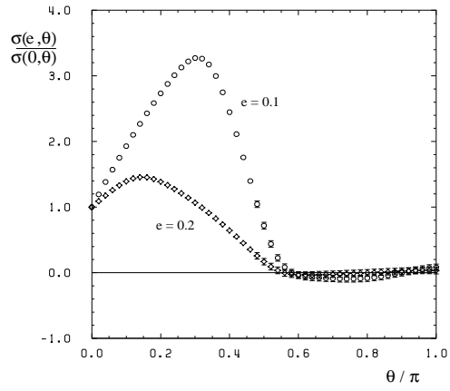
Fig. 4. The free energy F(\theta) , the topological charge density q(\theta) and the string tension \sigma(e, \theta) as a function of \theta for the \text{CP}^3 model on the 64^2 lattice at \beta = 2.7 . The solid curve in the figure at the top is the prediction of the large- N expansion. In the string tension figure at the bottom e denotes the external charge in units of the fundamental charge.
