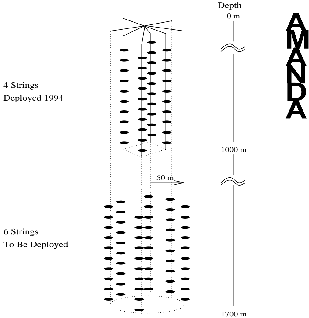
Figure 28. Diagram of the AMANDA neutrino detector [340]. The final configuration may differ slightly from that shown here.
