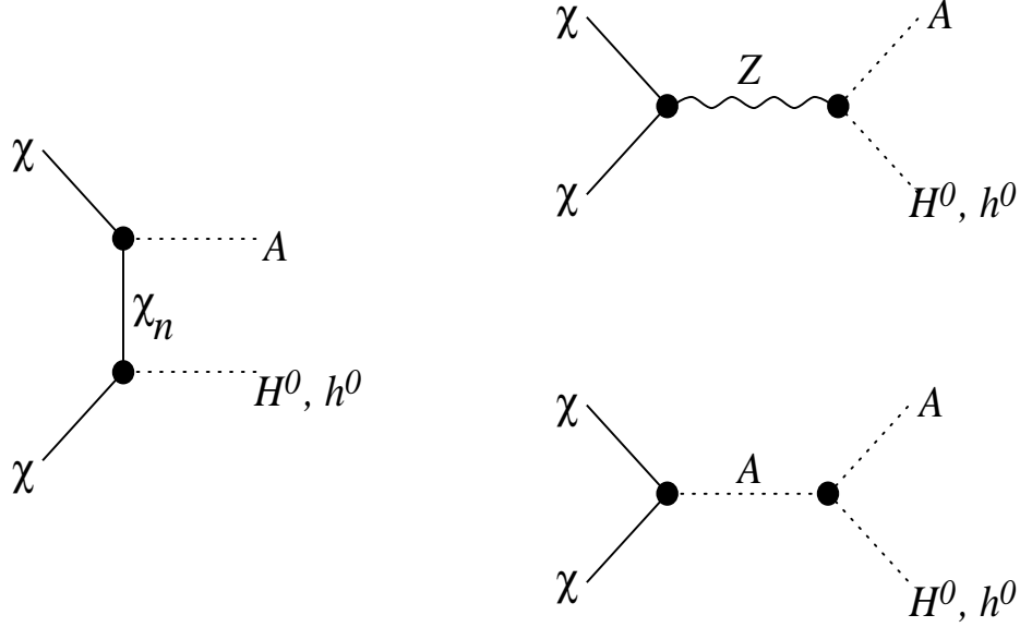
Figure 15. Diagrams for the amplitudes containing one pseudoscalar Higgs boson in the final state.
