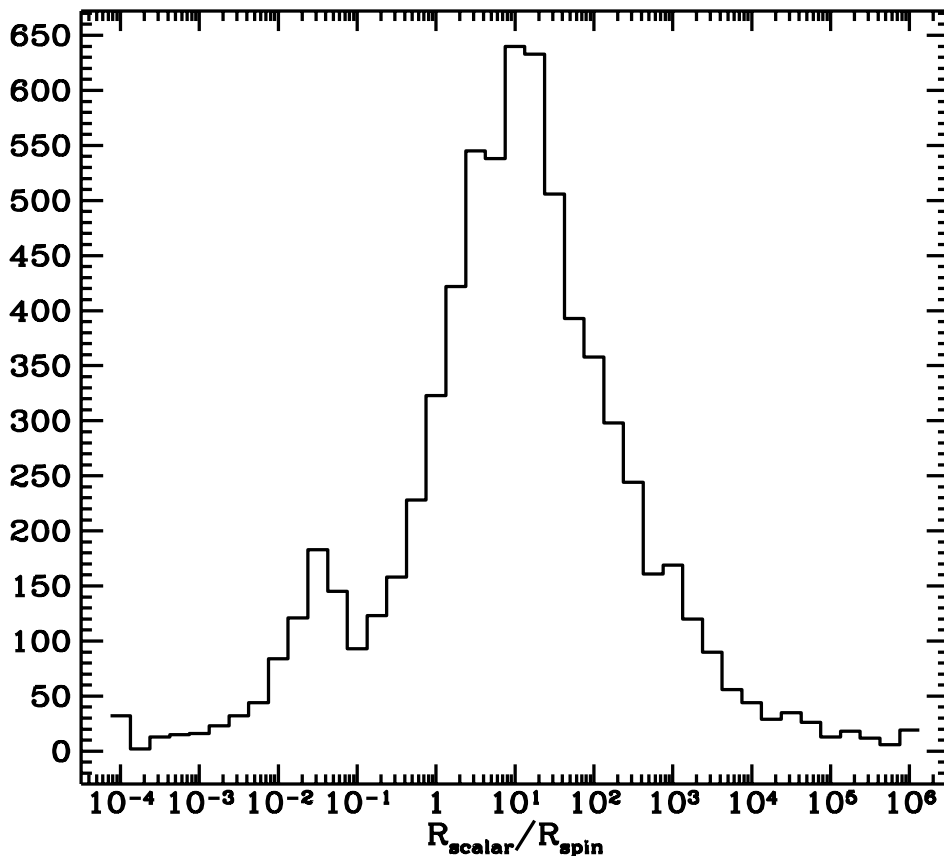
Figure 50. Histogram of the ratio of scalar rate to spin rate r = R_{\text{scalar}}/R_{\text{spin}} in a ^{73}\text{Ge} detector for the allowed dark-matter neutralinos.
