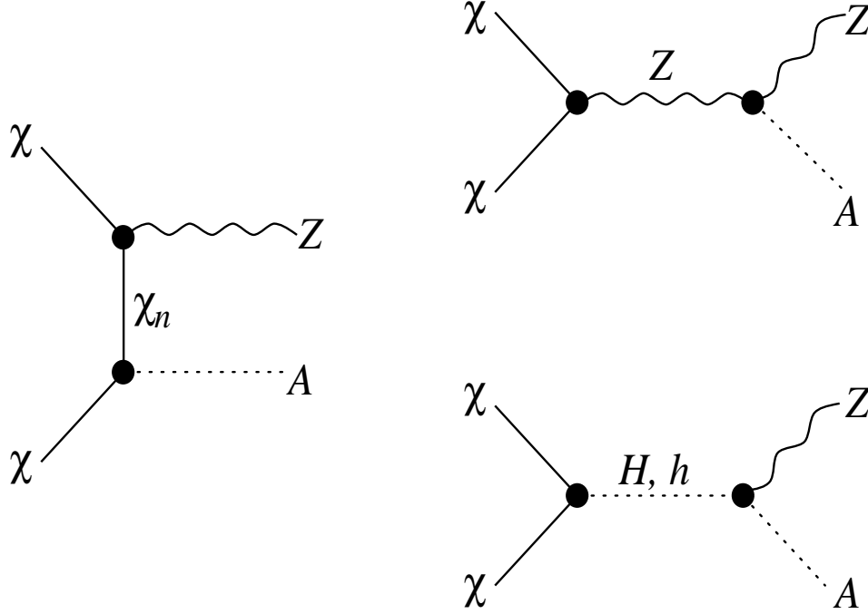
Figure 12. Diagrams for the process \chi\chi \rightarrow Z^0 A^0 .
