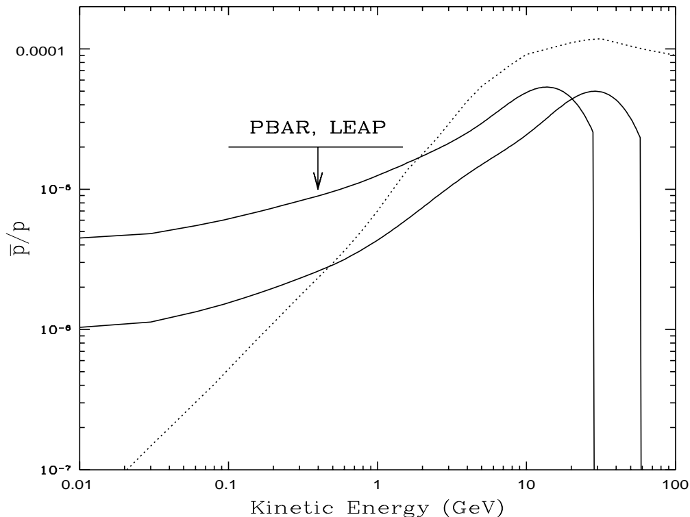
Figure 36. Observed antiproton/proton ratio as a function of kinetic energy. From Ref. [363].
