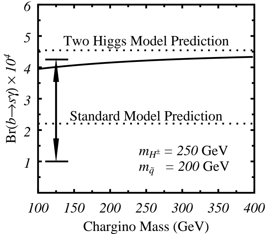
Figure 8. Example of the effect of chargino exchange on \text{Br}(b \rightarrow s\gamma) . The mixing angle appearing in the quark-squark-chargino vertex has been fixed at 0.1, and the only parameter allowed to vary is m_{\chi_{\pm}} . The solid line is the result for the branching ratio; the upper dotted line is the result ignoring the chargino contribution; the lower dotted line is the result ignoring both the chargino contribution and the charge-Higgs contribution, which is the usual standard-model result. The arrows show the CLEO 95% CL limits.
