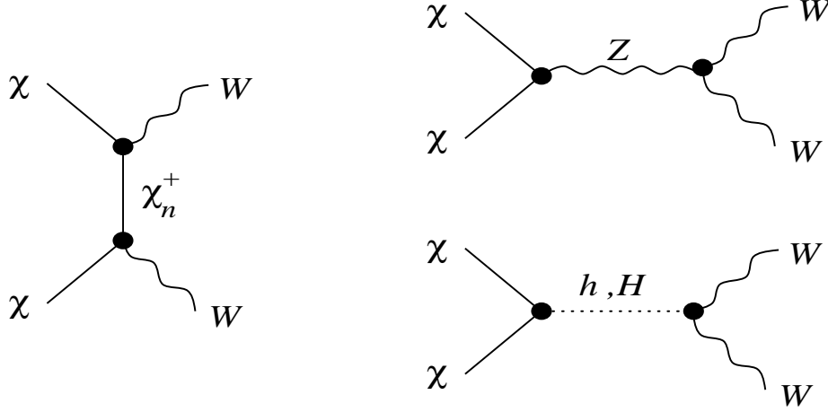
Figure 9. Diagrams contributing to neutralino annihilation to W^+W^- pairs.
