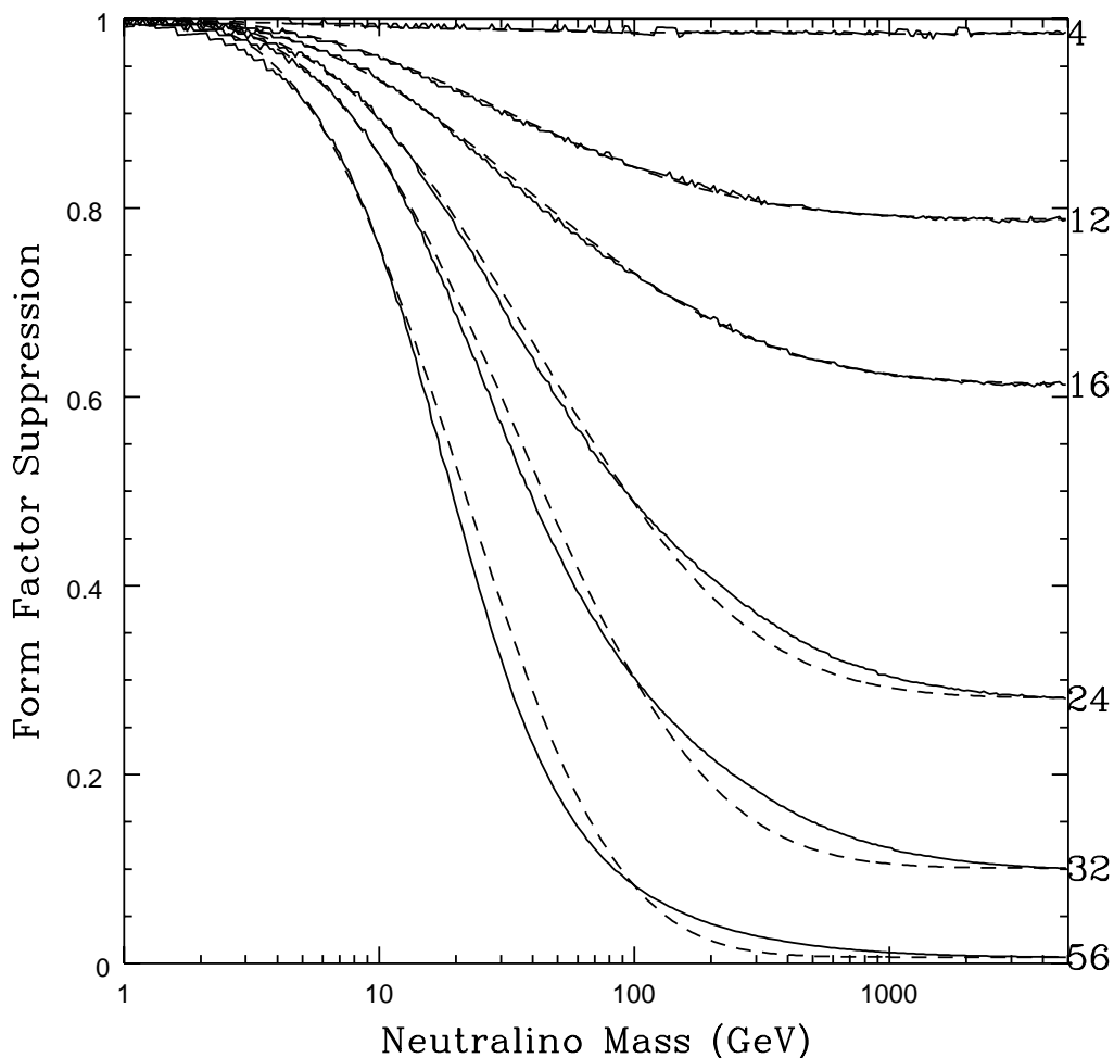
Figure 29. Form-factor suppression of capture in the Sun as a function of WIMP mass for nuclei with mass numbers 4, 12, 16, 24, 32, and 56. The solid curves are the exact results, and the dashed curves are the analytic approximation given here.
