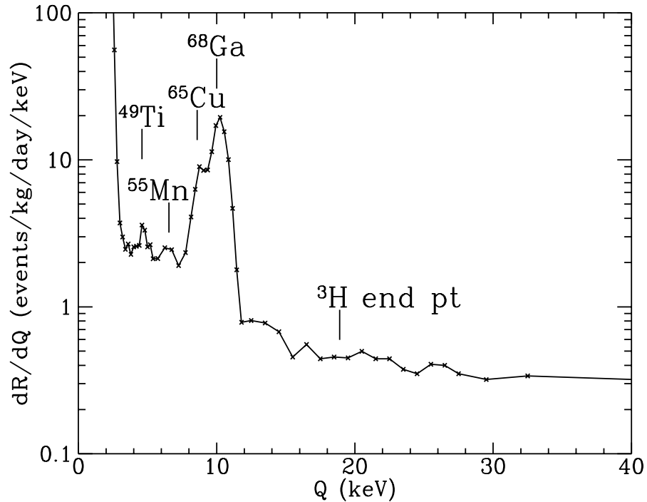
Figure 25. Measured gamma-ray background in an underground high-purity germanium ionization detector (data acquired by the UCB/UCSB/LBL experiment at Oroville [303][304]). Various gamma-ray lines are identified, as is the end point of the broad tritium spectrum. The rapid rise at low Q is the electronic noise. Compare with the potential WIMP signals shown in Fig. 23 and Fig. 24.
