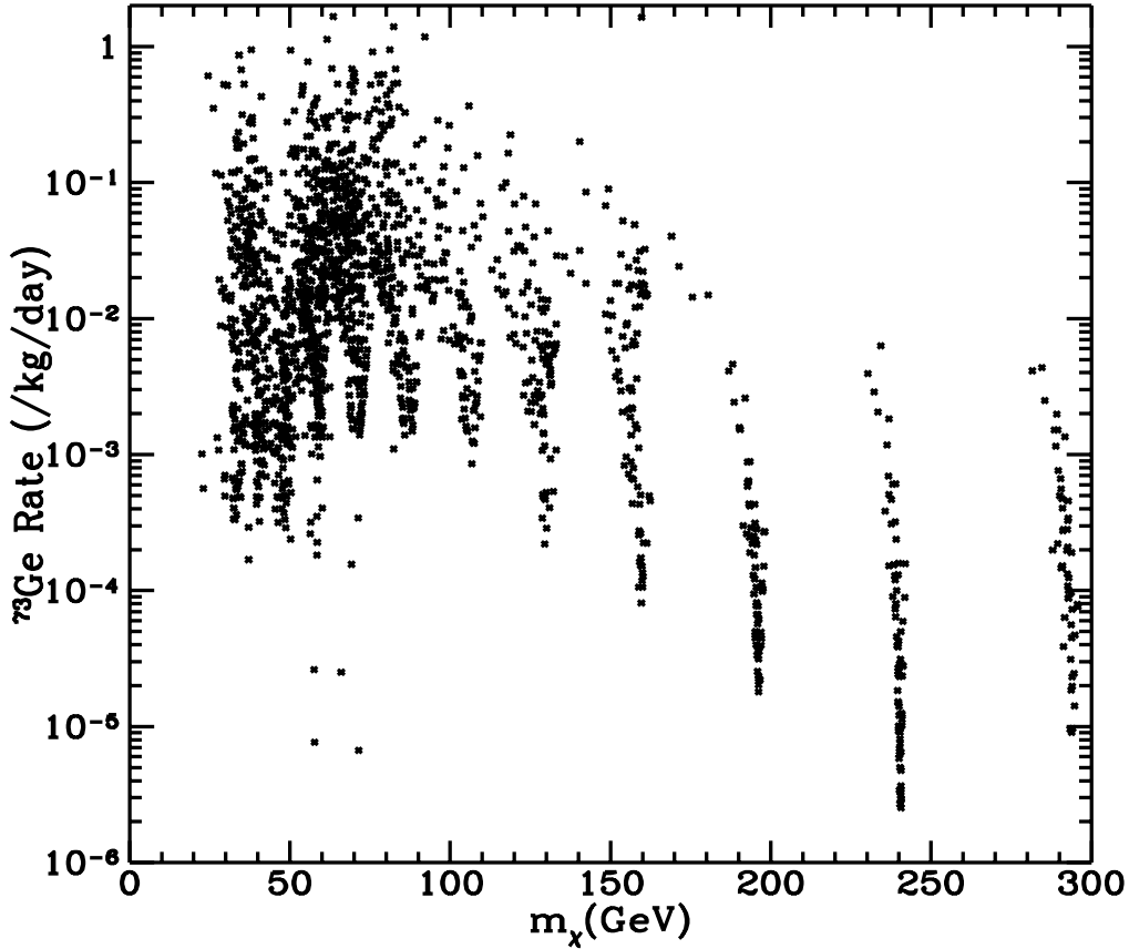
Figure 47. Predicted rate in a ^{73}\text{Ge} cryogenic detector vs neutralino mass for the allowed dark-matter models above. All constraints are implemented.
