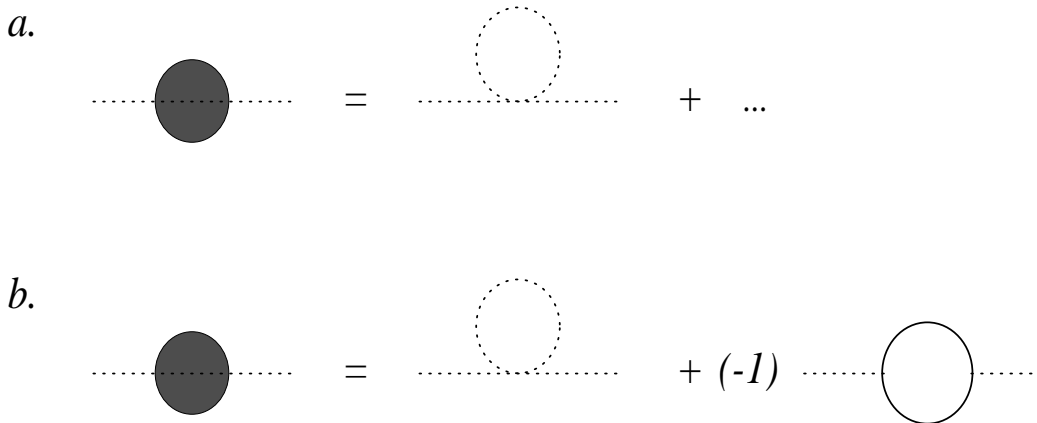
Figure 5. Radiative corrections to the mass of a scalar particle. The dotted curves are scalar propagators, and the solid curves are fermion propagators. (a) Diagrams with no supersymmetry, and (b) Diagrams with supersymmetry.
