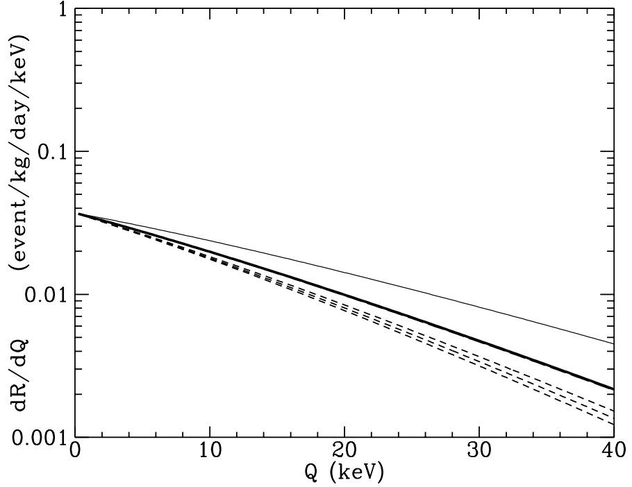
Figure 22. Theoretical differential event rate [Eq. (8.17)] vs. deposited energy for several different nuclear form factors. An arbitrary cross section of \sigma_0 = 4 \times 10^{-36} \text{ cm}^2 was chosen, with m_\chi = 40 \text{ GeV} and m_N = 68 \text{ GeV} , and standard values of the other parameters. The heavy solid line shows the best-estimate (i.e., the Woods-Saxon) form factor [Eq. (7.33)] for scalar interactions, while the long-dashed line (which falls on top of the heavy solid line) shows the exponential form factor [Eq. (7.31)]. The light solid line shows F(Q) = 1 (no form factor). The three spin form factors for germanium (Table 5) are shown as short-dashed lines.
