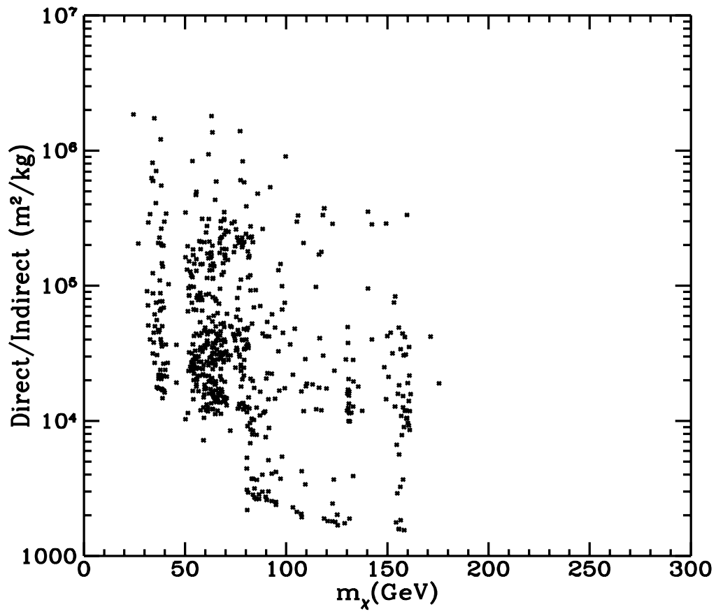
Figure 61. The ratio of direct to indirect rates is plotted for models with indirect rates between 10^{-4} \text{m}^{-2} \text{yr}^{-1} > \Gamma > 10^{-2} \text{m}^{-2} \text{yr}^{-1} .
