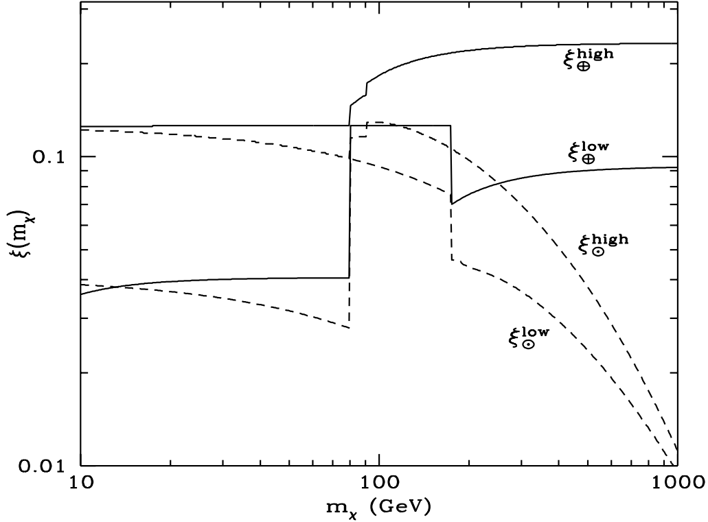
Figure 33. Upper and lower limiting values for the function \xi(m_\chi) for the Earth (solid curves) and Sun (dashed curves).
