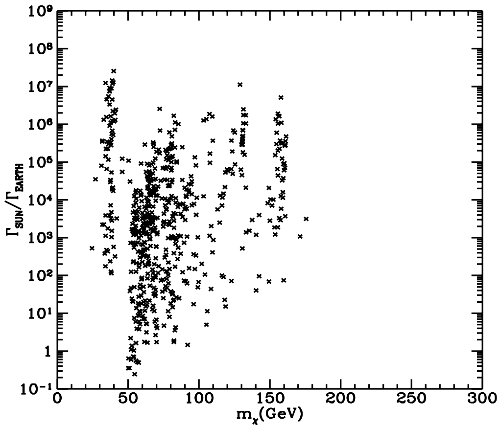
Figure 59. Ratio of indirect-detection rates for neutrinos from the Sun and Earth vs. the neutralino mass. Only models which predict rates between 10^{-2} \text{ m}^{-2} \text{ yr}^{-1} and 10^{-4} \text{ m}^{-2} \text{ yr}^{-1} are plotted.
