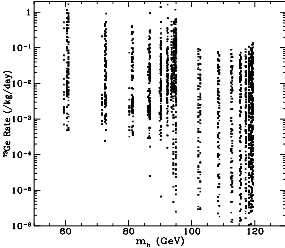
Figure 48. Predicted rate in a ^{73}\text{Ge} cryogenic detector vs lightest scalar Higgs mass for the allowed dark-matter models above. All constraints are implemented. The gaps are due to the incomplete parameter space sampling.
