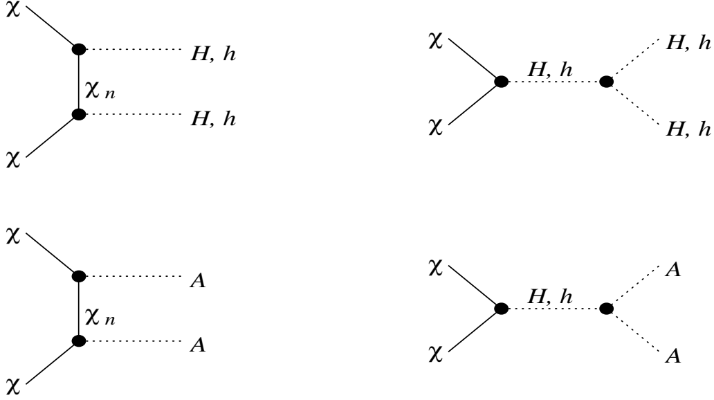
Figure 14. Diagrams for neutralino-annihilation to the H^0 H^0 , H^0 h^0 , h^0 h^0 , and A^0 A^0 final states.
