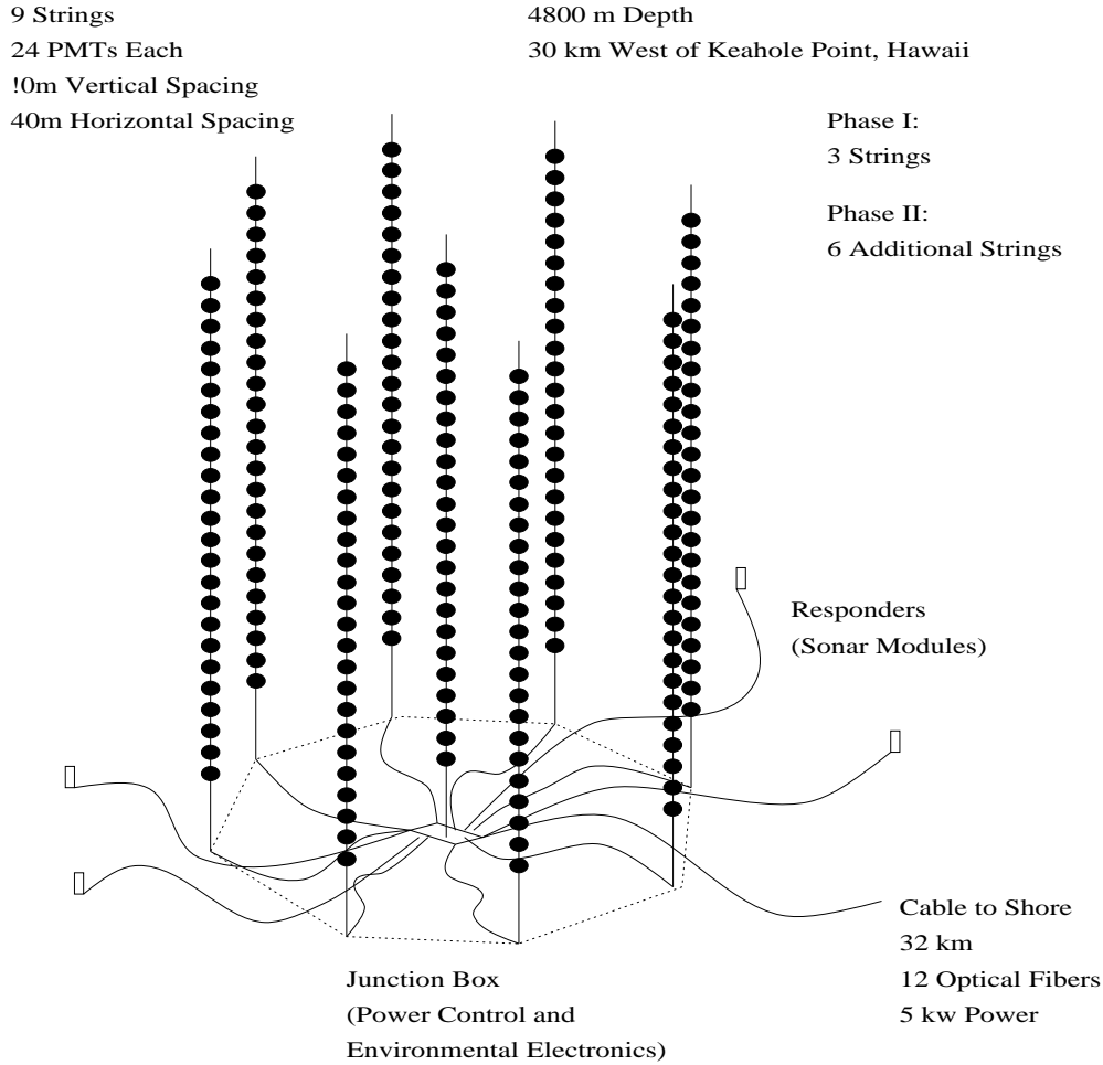
Figure 27. Diagram of the DUMAND neutrino detector [339].
