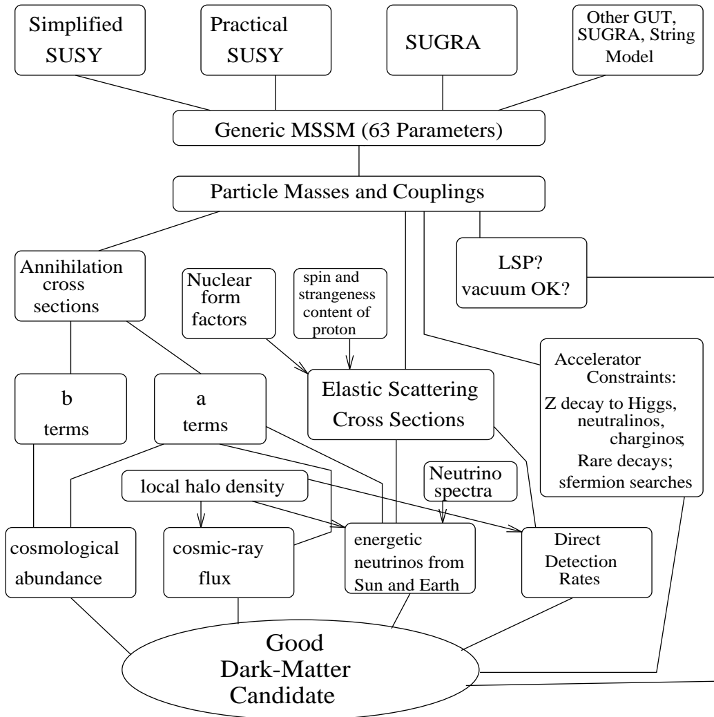
Figure 62. Diagrammatic summary of calculations needed in the study of supersymmetric dark matter.
