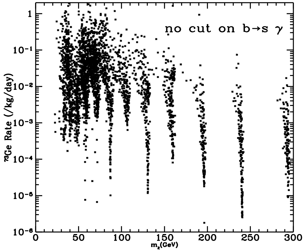
Figure 55. Same as Fig. 47 except that the constraint 10^{-4} < \text{Br}(b \rightarrow s\gamma) < 4.2 \times 10^{-4} has been relaxed.
