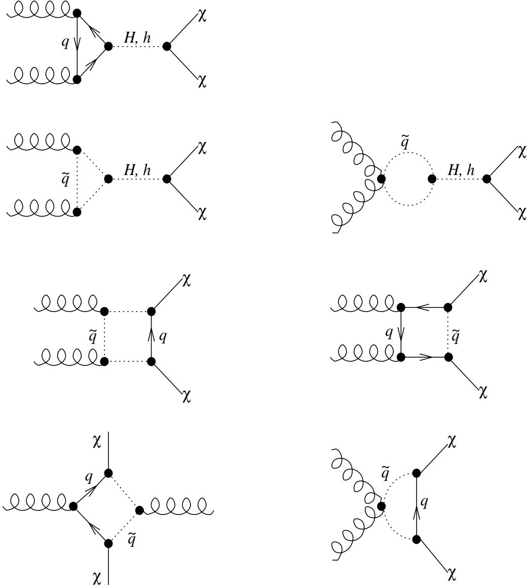
Figure 21. Feynman diagrams contributing to the gluonic interaction with neutralinos, which contributes to the scalar elastic-scattering amplitude for neutralinos from nuclei.
