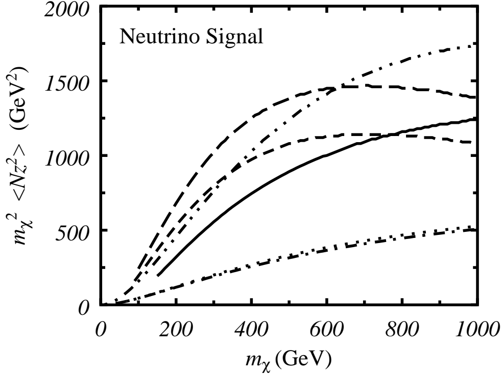
Figure 31. The second moment, m_\chi^2 \langle Nz^2 \rangle , of the neutrino energy distribution from injection of particles with energy equal to the WIMP mass m_\chi in the Sun. The solid curve is for t\bar{t} pairs, the upper (lower) dashed curve is for W^+W^- ( ZZ ) pairs, and the upper dot-dash curve is for \tau\bar{\tau} pairs. At the bottom are the b\bar{b} and c\bar{c} curves, and the b\bar{b} curve is slightly higher than the c\bar{c} curve.
