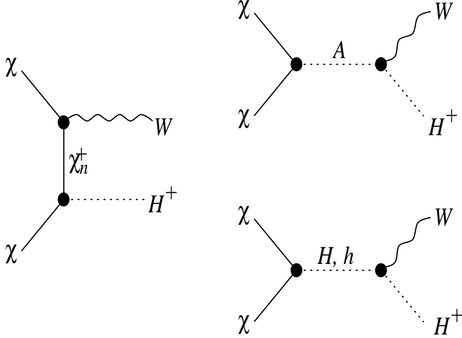
Figure 13. Diagrams for the process \chi\chi \rightarrow W^+H^- . The charge conjugate process is similar.
