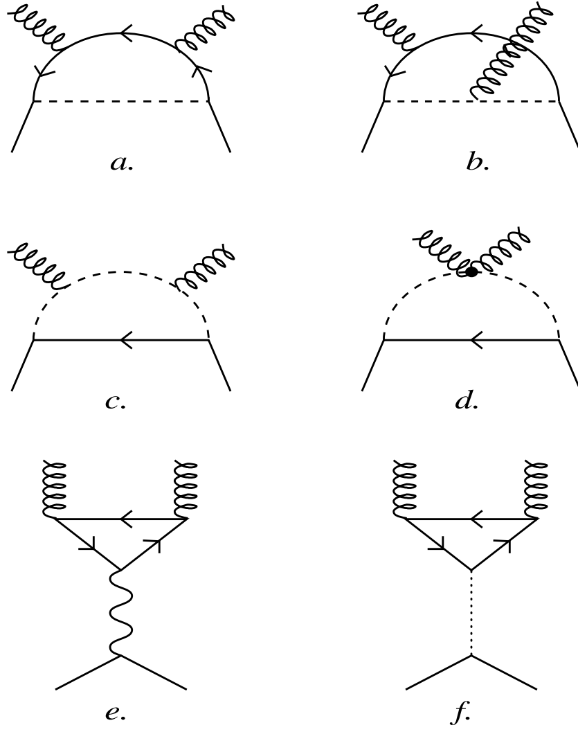
Figure 17. Diagrams contributing to neutralino annihilation into gluons: (a)-(d) Quark-squark loops and (e) and (f) the exchange of the Z^0 boson or the pseudoscalar Higgs boson A^0 . From Ref. [252].
