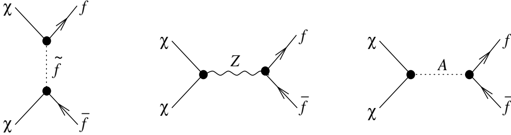
Figure 16. Diagrams contributing to neutralino annihilation into fermions.
