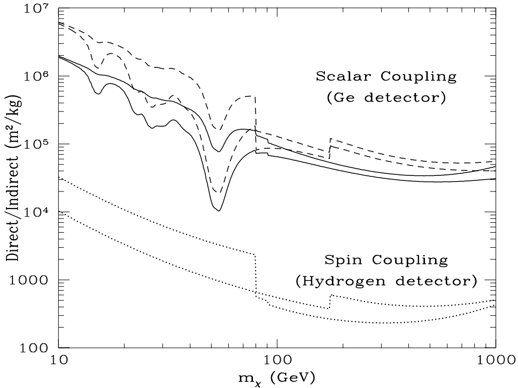
Figure 35. Direct vs indirect detection of scalar- and spin-coupled WIMPs. For scalar-coupled WIMPs, we plot the ratio of the rate for elastic scattering from Ge in a laboratory detector to the flux of upward muons induced by neutrinos from annihilation in the Sun and Earth as a function of WIMP mass. The solid (dashed) curves are the ratios for the upper (lower) limit for the neutrino fluxes. The upper (lower) pair of these curves are for models that give \Gamma = 10^{-4} ( 10^{-2} ) \text{m}^{-2} \text{yr}^{-1} , and the model dependent uncertainties are indicated by the range of values between the highest and lowest curves. For scalar-coupled WIMPs, the ratios for detectors with different composition can be obtained using the scalings plotted in Fig. 26. For WIMPs with axial-vector (i.e., spin) couplings to nuclei, we plot ratios of the rate for elastic scattering from hydrogen in a laboratory detector to the flux of upward muons induced by neutrinos from annihilation in the Sun. The upper (lower) dotted curve is the ratio for the upper (lower) limit to the neutrino fluxes for spin-coupled WIMPs, and the model-dependent uncertainty is indicated by the range of values between these curves. In both cases, we neglect detector thresholds and backgrounds and assume efficiencies of order unity. From [305].
