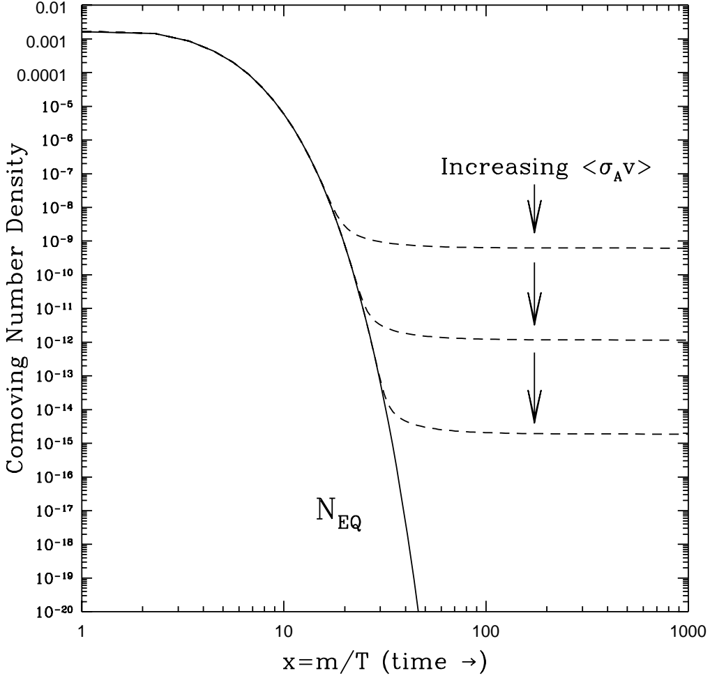
Figure 4. Comoving number density of a WIMP in the early Universe. The dashed curves are the actual abundance, and the solid curve is the equilibrium abundance. From [31].
