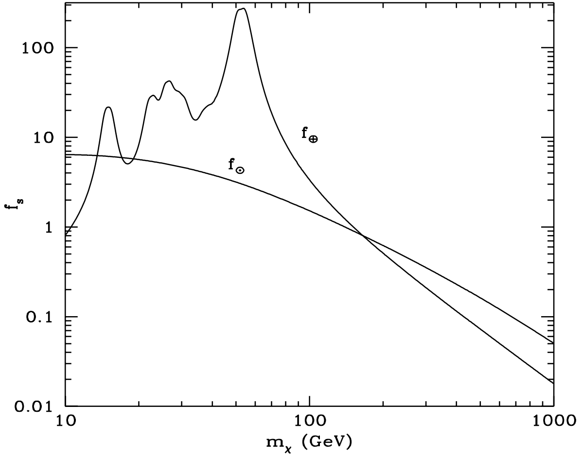
Figure 30. Plot of the neutralino-mass dependence of the scalar capture rate in the Sun, f_{\odot}(m_{\chi}) , and Earth, f_{\oplus}(m_{\chi}) as a function of neutralino mass.
