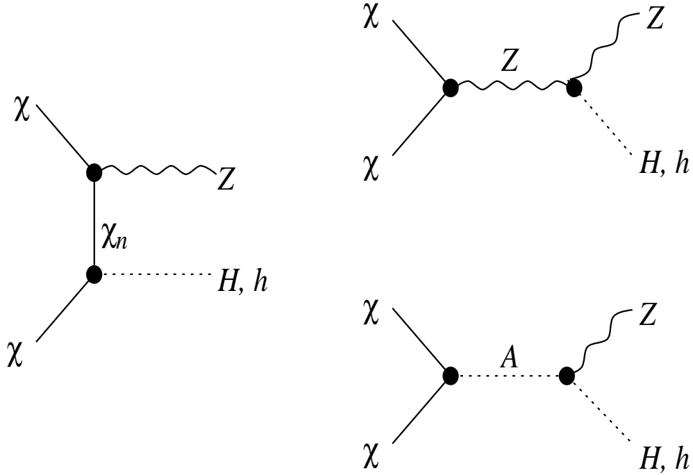
Figure 11. Diagrams for the processes \chi\chi \rightarrow Z^0 H^0 and \chi\chi \rightarrow Z^0 h^0 .
