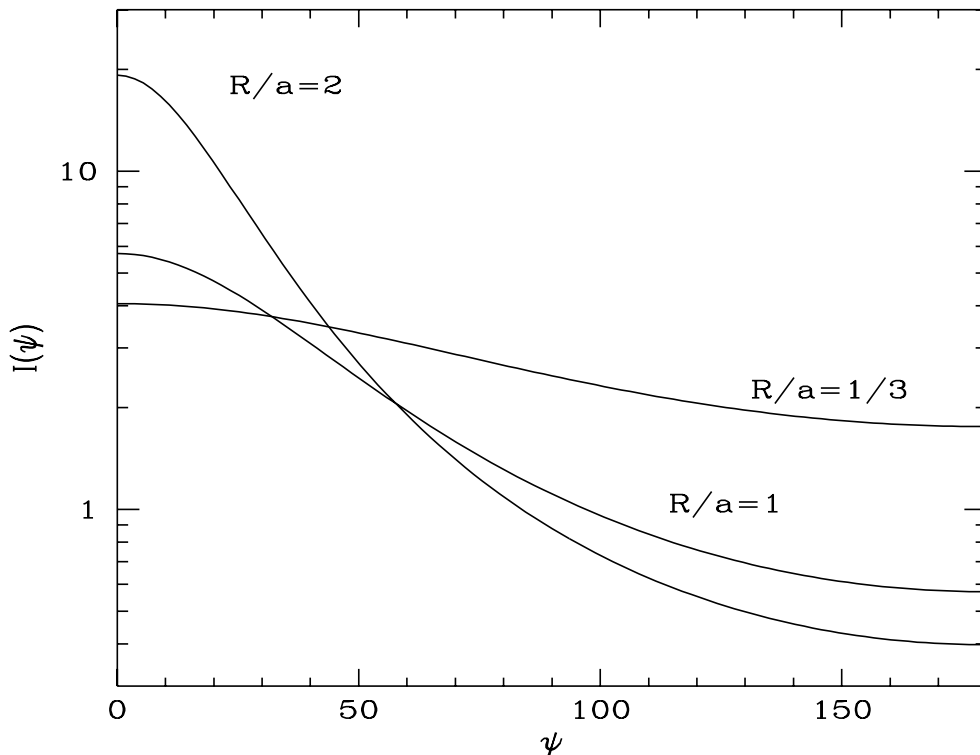
Figure 38. The intensity of a gamma-ray signal from WIMP annihilation in the halo as a function of the angle \psi between the line of sight and the Galactic center, for several values of R/a . From [378][379][380].
