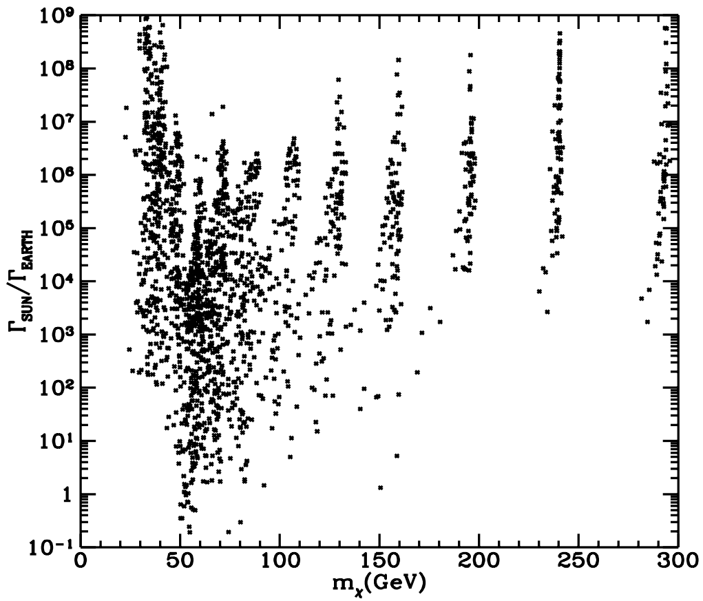
Figure 58. Ratio of indirect-detection rates for neutrinos from the Sun and Earth vs. the neutralino mass. All allowed models are plotted.
