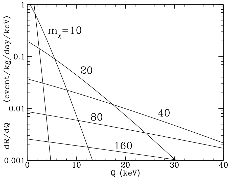
Figure 23. Theoretical differential event rate for WIMPs of various masses hitting a germanium target. WIMP masses are labeled in GeV. An arbitrary cross section of \sigma_0 = 4 \times 10^{-36} \text{ cm}^2 was chosen with standard values for the other parameters. Compare these curves with a typical experimental gamma-ray background shown in Fig. 25. Note the rate axis scale is 100 times smaller than in Fig. 25, and the cross section chosen is very high for neutralinos (see Section 11).
