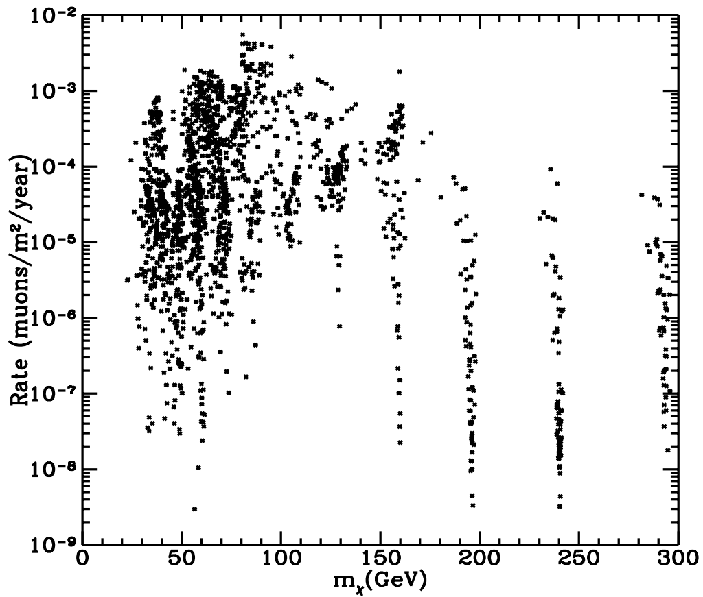
Figure 57. Indirect-detection rate vs neutralino mass. The sum of the rates for upward muons from both the Sun and Earth is shown. Currently planned experiments will be sensitive in the 10^{-2} \text{m}^{-2} \text{yr}^{-1} to 10^{-4} \text{m}^{-2} \text{yr}^{-1} range.
