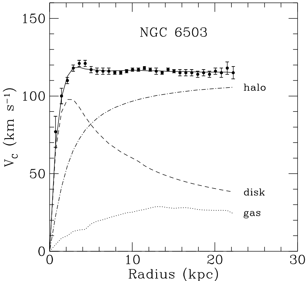
Figure 1. Rotation curve for the spiral galaxy NGC6503. The points are the measured circular rotation velocities as a function of distance from the center of the galaxy. The dashed and dotted curves are the contribution to the rotational velocity due to the observed disk and gas, respectively, and the dot-dash curve is the contribution from the dark halo. (From Ref. [36].)
