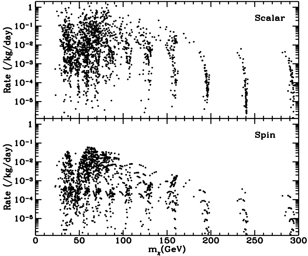
Figure 49. Predicted rate in a ^{73}\text{Ge} cryogenic detector vs. neutralino mass for the allowed dark-matter models above. Panel (a) shows only the scalar neutralino-nucleus interaction, while panel (b) shows only the spin interaction. All constraints are implemented.
