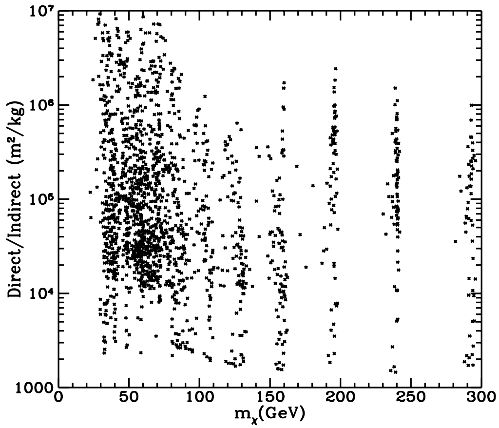
Figure 60. The ratio of direct to indirect rates is plotted for all allowed models.
