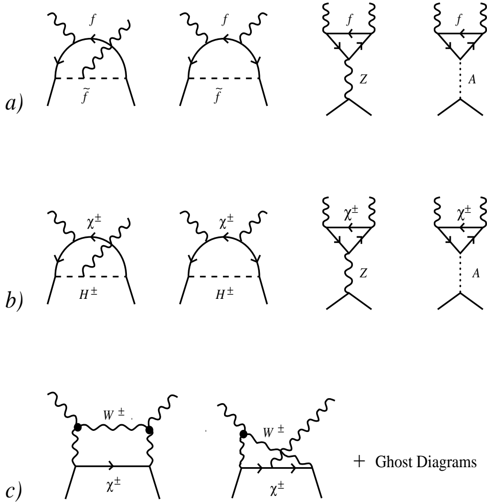
Figure 18. Diagrams contributing to neutralino annihilation into photons: (a) fermion-sfermion loops, (b) charged-Higgs-chargino loops, and (c) chargino- W -boson loops. From Ref. [266].
