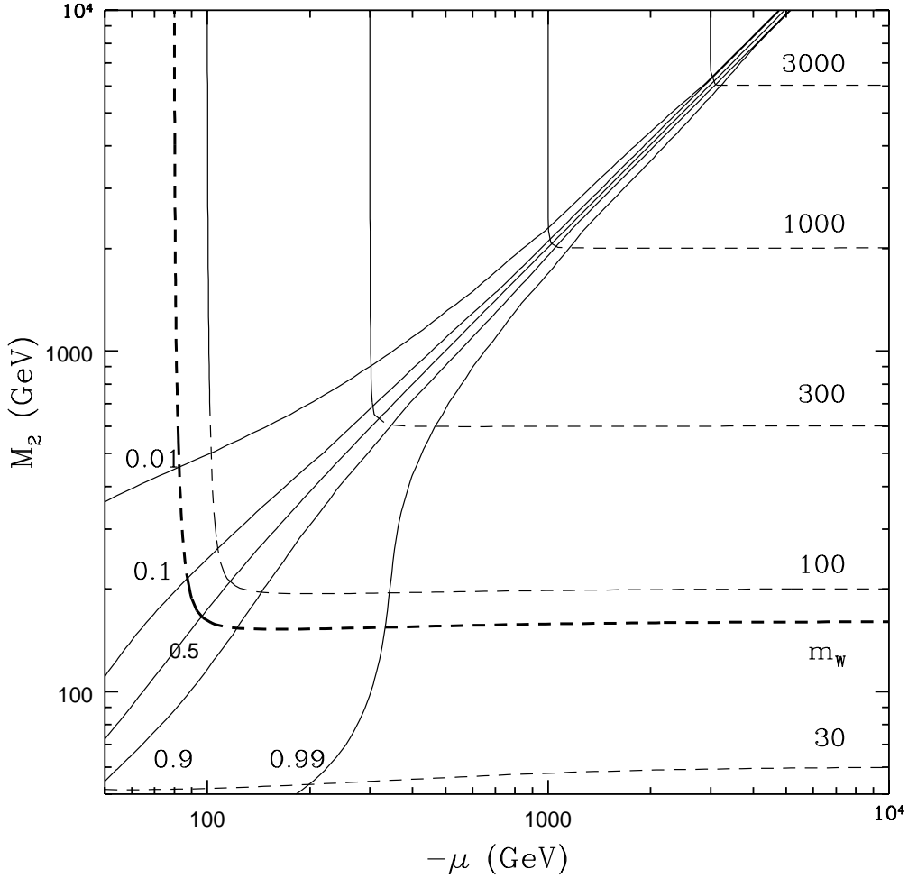
Figure 7. Same as Fig. 6, but for negative values of \mu .
