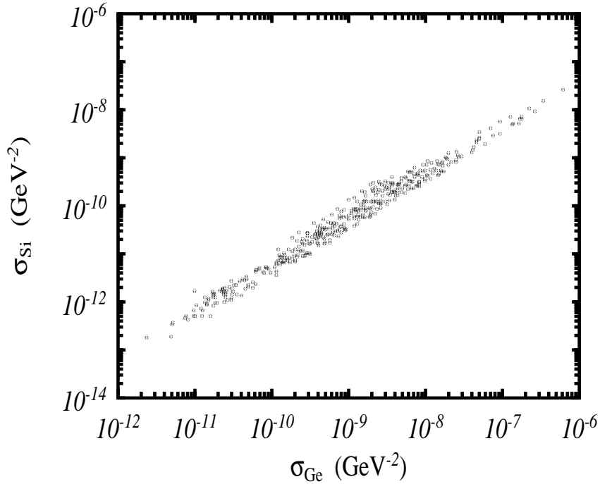
Figure 45. Illustration of the scaling between the ^{29}\text{Si} and ^{76}\text{Ge} elastic-scattering cross sections. The ratio is very nearly constant and approximately an order of magnitude, indicating the validity of the A^2 scaling of the cross section. The increased spread at lower values is due to the contamination from the spin-dependent cross section, which is noticeable only when the scalar cross section is small. The set of models plotted here is slightly different than those described in the text.
