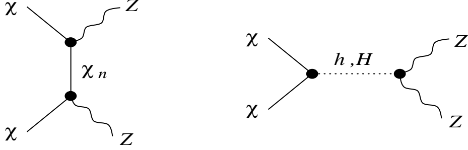
Figure 10. Diagrams contributing to neutralino annihilation to Z^0 Z^0 pairs.
