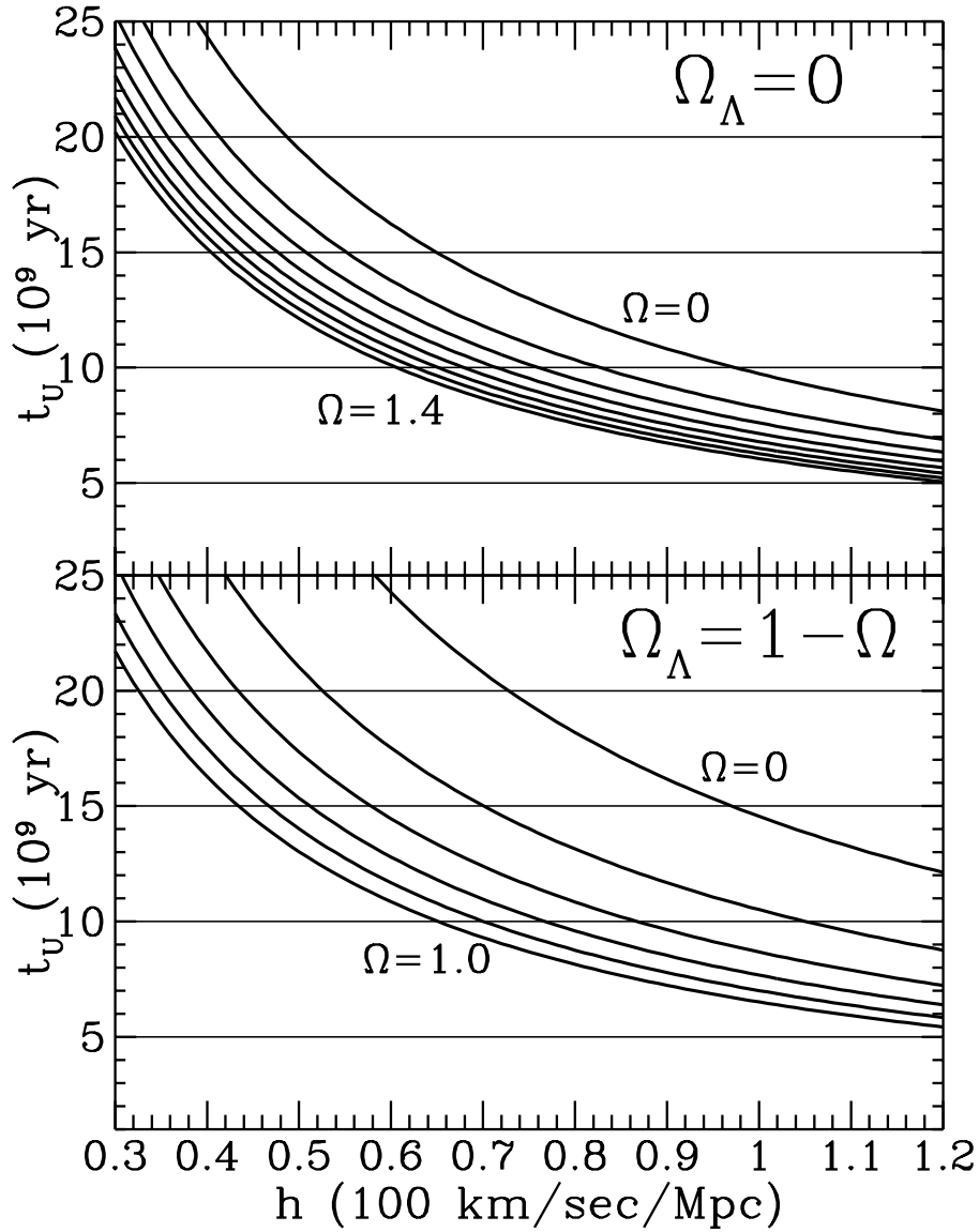
Figure 2. Age of the Universe for various values of h , the Hubble constant, and \Omega , the matter density. The top panel shows a Universe with no cosmological constant ( \Lambda = 0 ), while the bottom panel shows a flat Universe with a cosmological constant ( \Omega + \Omega_\Lambda = 1 ). In the top panel, the curves range from \Omega = 0 to \Omega = 1.4 in steps of 0.2, and in the bottom panel, \Omega ranges from 0 to 1 also in steps of 0.2.
