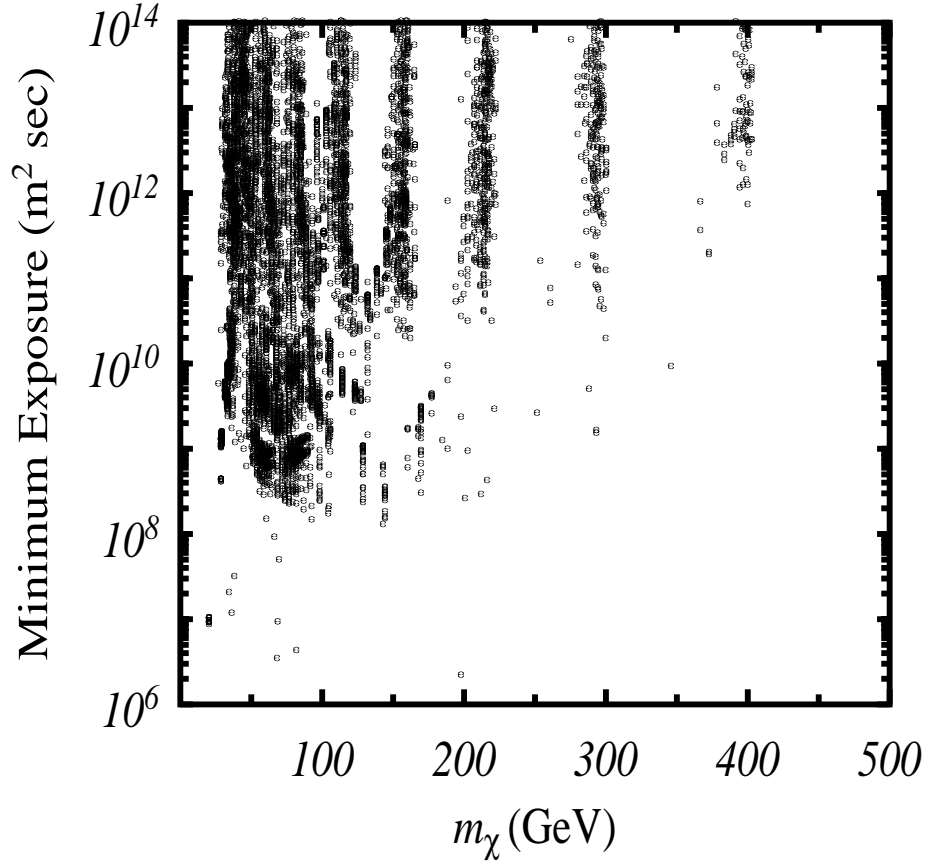
Figure 39. Minimum exposure required for a 3\sigma detection of gamma rays from neutralino annihilation in the Galactic center, versus mass of the neutralino, for the survey of supersymmetric parameter space discussed in the text.
