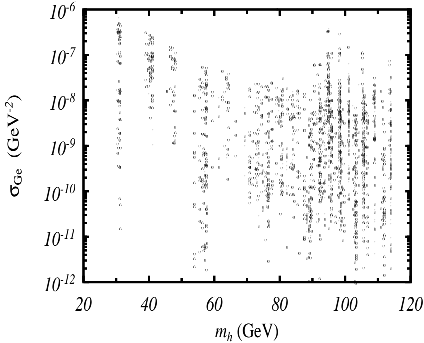
Figure 46. Dependence of the scalar ^{76}\text{Ge} cross section on the lighter Higgs-boson mass. For m_h \lesssim 70 GeV, the dependence is clear, indicating that Higgs-boson exchange is playing an important role in the process. The set of models plotted here is slightly different than those described in the text.
