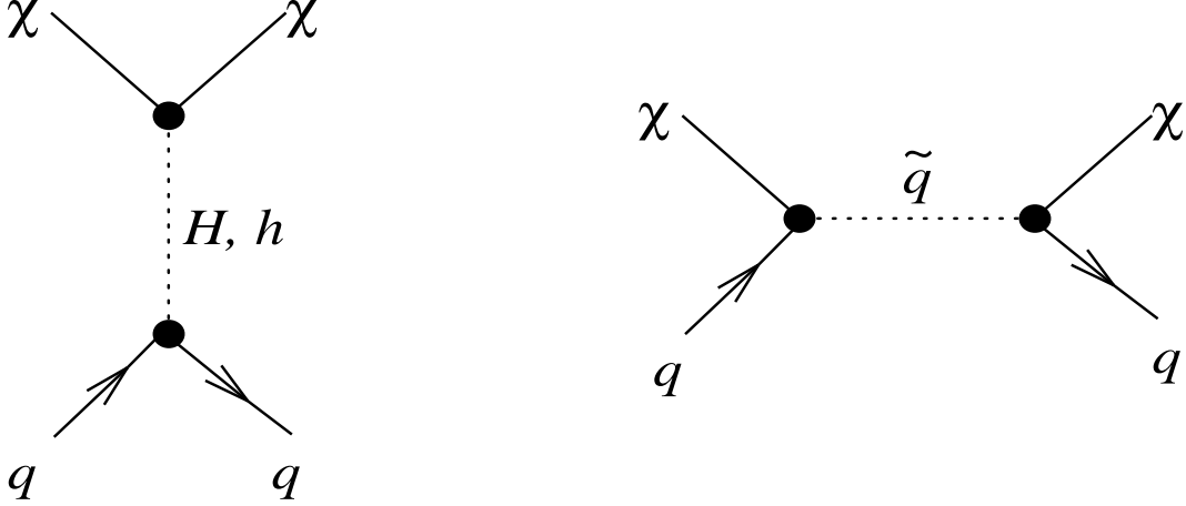
Figure 20. Feynman diagrams contributing to the scalar elastic-scattering amplitude of a neutralino from quarks.
