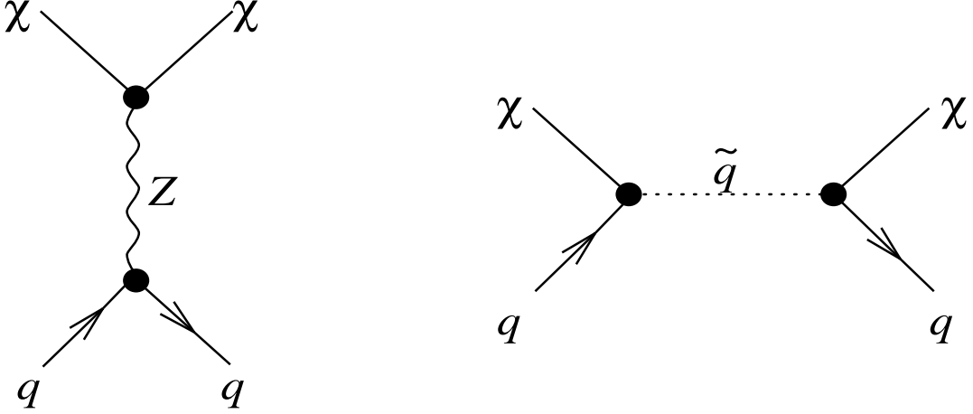
Figure 19. Feynman diagrams contributing to the spin-dependent elastic scattering of neutralinos from quarks.
