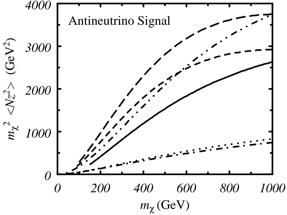
Figure 32. Same as Fig. 31, but for antineutrinos.
