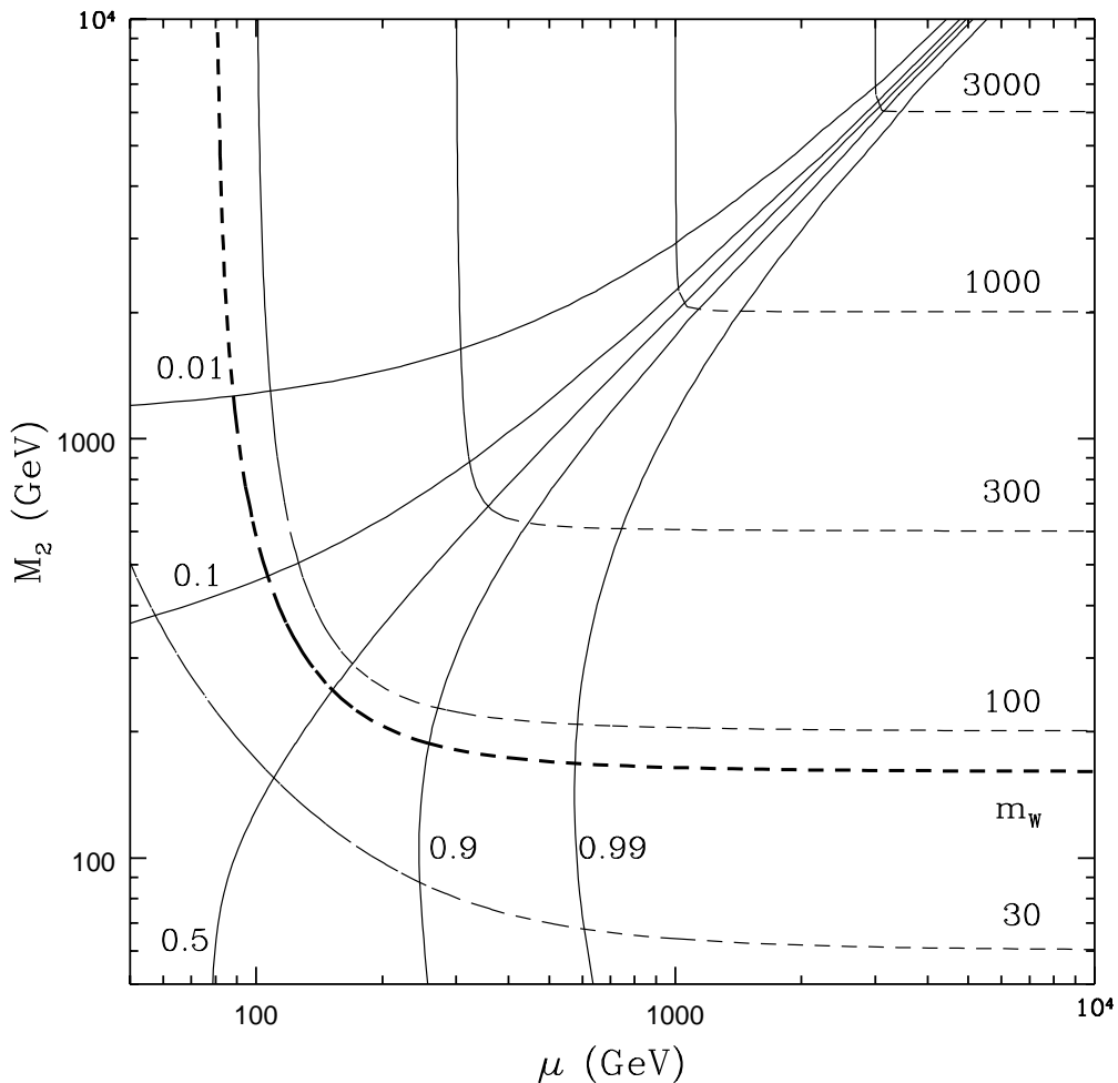
Figure 6. Contour plot of the neutralino mass and composition in the M_2 - \mu plane. The broken curves are contours of constant neutralino mass m_\chi (in GeV), and the solid curves are contours of constant gaugino fraction f_g . Here, \tan \beta = 2 and the GUT relation, M_1 = \frac{5}{3} \tan^2 \theta_W M_2 has been used. Only positive values of \mu are shown. From Ref. [134].
