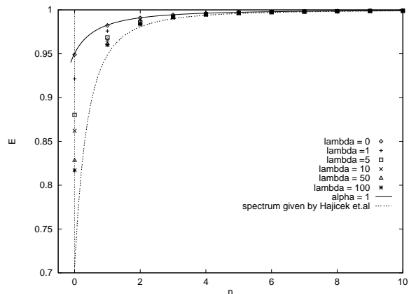
FIG. 4. The \lambda -dependence of the spectrum E(n) for m = 1.0000 . The time slicing parameter is chosen to be \lambda = 0.0000, 1.0000, 5.0000, 10.000, 50.000 and 100.00 . As \lambda increases, the spectrum of E approaches to (1.4) drawn by the dashed line.
