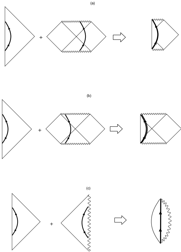
FIG. 1. Penrose diagrams of possible spacetimes constructed by the Minkowski-Schwarzschild junction with E < 1 . The trajectories of the dust shell in the Minkowski and Schwarzschild spacetimes are drawn. The two spacetimes are glued at the shell boundary. These figures show (a) a black hole spacetime for 1/2 < E < 1 (in which the junction condition requires that both R'_+ and R'_- are positive), (b) a wormhole spacetime for 0 < E < 1/2 (in which R'_+ < 0 and R'_- > 0 ), and (c) a negative mass spacetime (in which R'_+ < 0 and R'_- ) without any asymptotic flat region.
