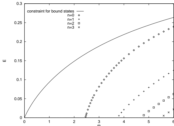
FIG. 3. The eigenvalues of E for the wave functions of wormhole formation in a static time slicing. The m -dependence of E is shown for the quantum numbers n = 0, 1, 2 and 3 . The solid line given by R_3 > \pi/\sqrt{-V_{\min}} means a rough upper boundary of the allowed range of E .
