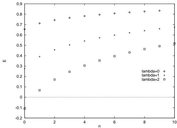
FIG. 5. The \lambda -dependence of the spectrum E(n) for m = 10.000 . The time slicing parameter is chosen to be \lambda = 0.0000, 1.0000 and 2.0000 . It is shown in this figure that the spectrum does not remain in the range 1 > E > 1/2 and even the negative mass states are allowed.
