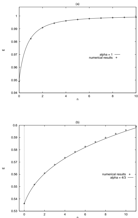
FIG. 2. The eigenvalues of E for the wave functions of black hole formation in a static time slicing. The validity of the approximate formula (4.12) checked by numerical calculations. The value of m is chosen to be (a) m = 1.0000 and (b) m = 100.00 . The spectrum given by (4.12) is drawn by solid lines which corresponds to (a) \alpha = 1 and (b) \alpha = 4/3 respectively.
