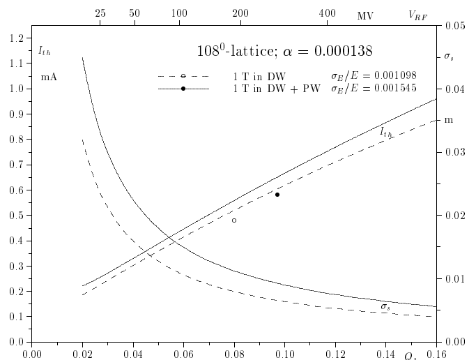
Figure 1. Calculated and measured TMCI thresholds vs. Q_s for two settings of damping and polarization wigglers DW and PW
