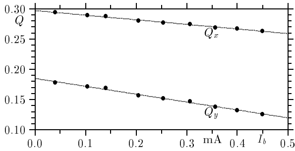
Figure 2. Measured tune change with bunch current
