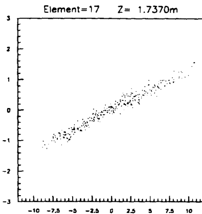
Fig. 3 Longitudinal phase space for 10 nC, before compression.
