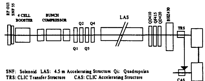
Fig. 1 CTF line in 1995
