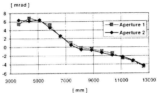
Fig. 3. Dipole field direction vs longitudinal position in both apertures at injection field level
