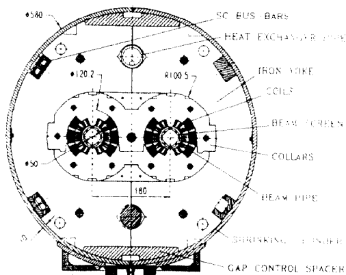
Fig. 1 Cross-section of the first full scale prototype (CERN-INFN 1)
