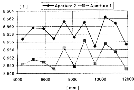
Fig. 4. Dipole field value vs longitudinal position in both apertures at 8.65 T
