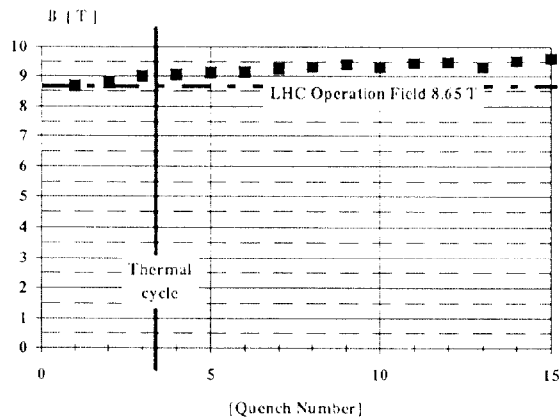
Fig. 2 Training curve at superfluid helium
