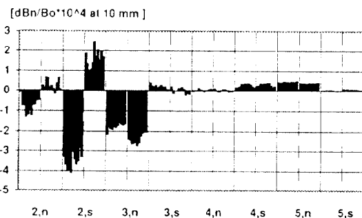
Fig. 4. Dipole field value vs longitudinal position in both apertures at 8.65 T
