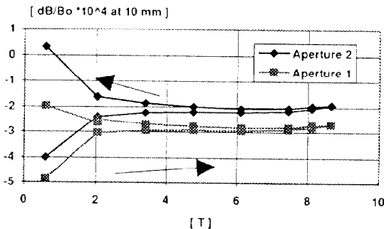
Fig. 6 Normal sextupole harmonic integrated over 0.75 m in both apertures as a function of field
