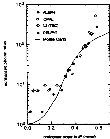
Figure 1: Normalised background rates vs. slope of the asymmetric orbit bump
