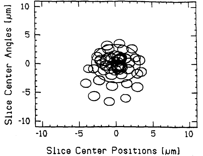
Figure 4. 'Small' emittance taken as reference.
