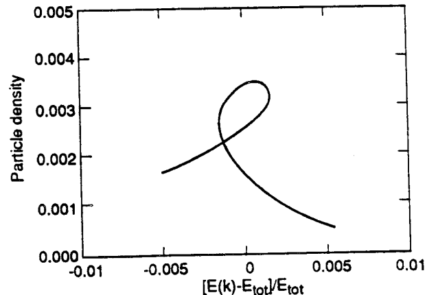
Figure 2. Energy deviation of slices of beam.
