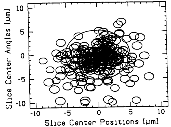
Figure 6. 'Large' emittance with 100 nm jitter on quadrupoles.
