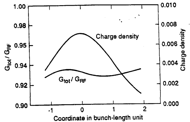
Figure 1. Relative accelerating voltage resulting from a truncated charge distribution.
