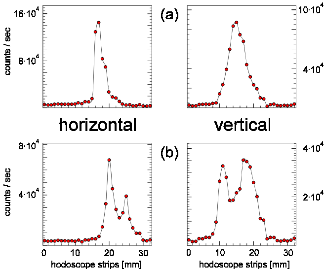
FIGURE 3: Beam profiles of the extracted beam as measured with the hodoscope of scintillation counters, (a) at the maximum extraction efficiency and (b) off-maximum.
