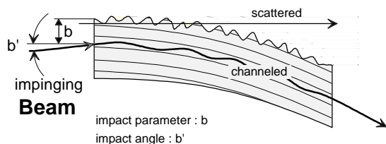
FIGURE 6 : Importance of the surface quality for first-pass channeling and extraction.
