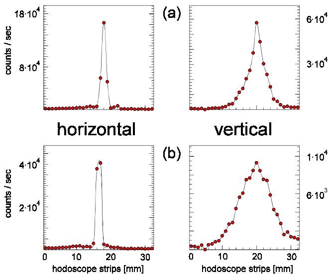
FIGURE 5 : Horizontal and vertical beam profiles measured with the hodoscope for the "U-shaped" crystal, cf. Fig. 3.
