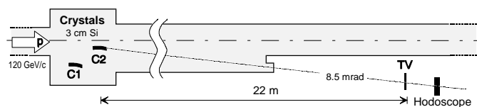
FIGURE 1 : Schematic view of the experimental apparatus used in the SPS extraction experiment with a bent crystal. C1 and C2 are two crystals mounted on goniometers. The detectors for the extracted beam are located 22 meters downstream of the crystals. For details, see text.
