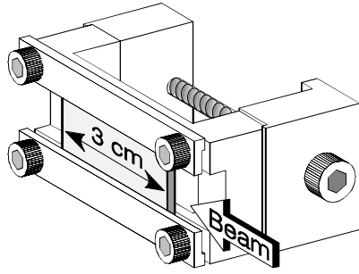
FIGURE 2: The silicon crystal bent on the "Serpukhov type" bending device. The bending is adjusted with a differential screw before mounting in the vacuum tank
