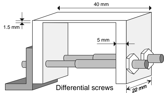
FIGURE 4: Schematic drawing of the new "U-shaped" silicon crystal, cut out of a block of silicon, including the "feet" needed to bend it. Bending is achieved with two differential screws.
