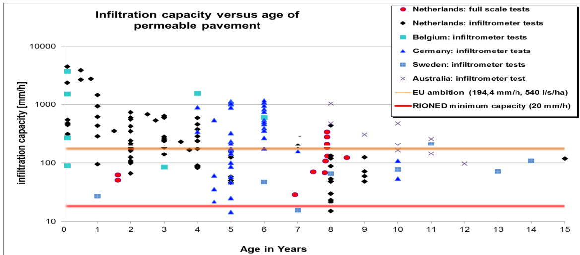
Figure 5 International permeable pavement infiltration capacity research results [Boogaard, 2015]
