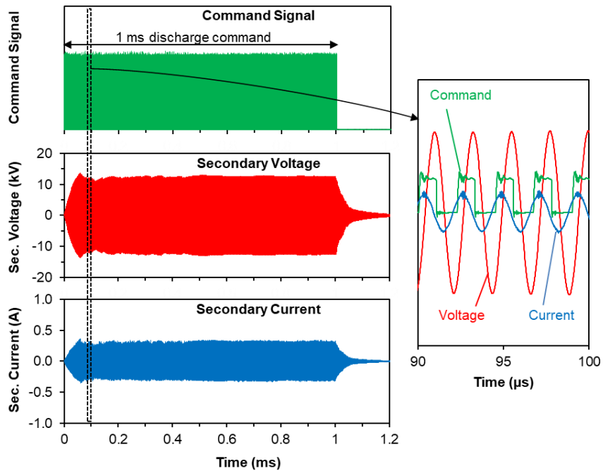
Figure 2- 3. The command signal, measured secondary voltage signal, and measured current signal during corona discharge.
