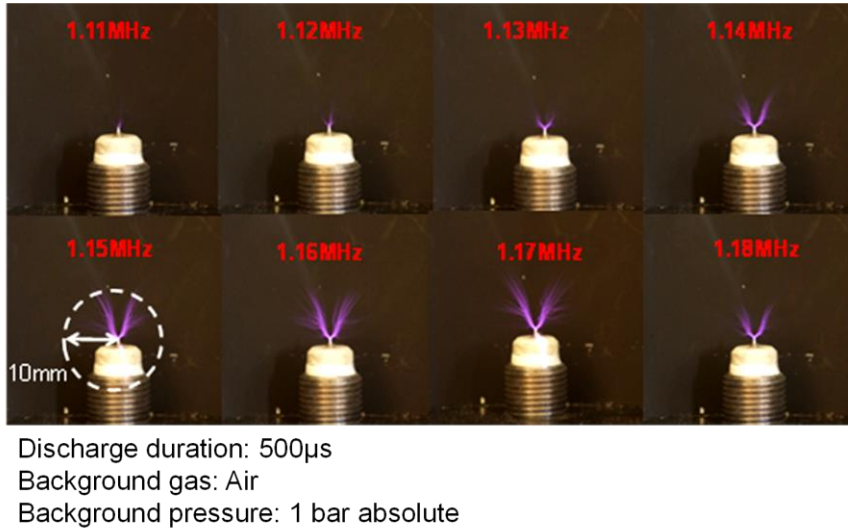
Figure 3- 5. The corona plasma length within the selected frequency range of the command signals.
