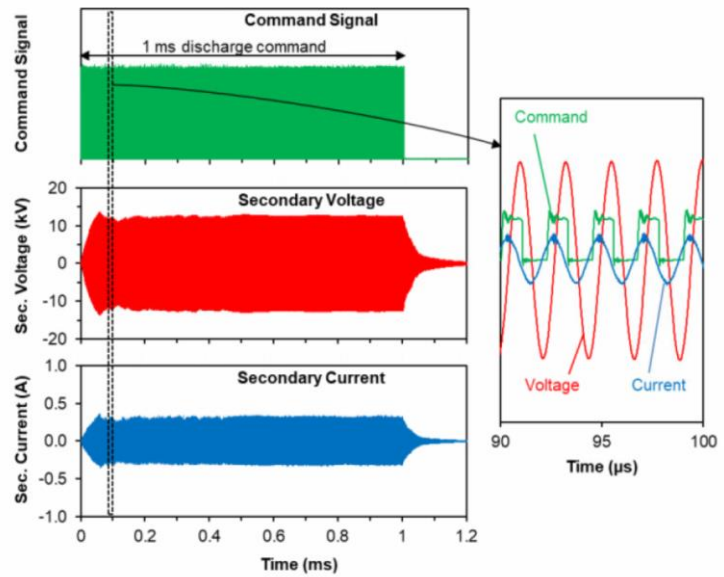
Figure 1- 4. Corona discharge.
