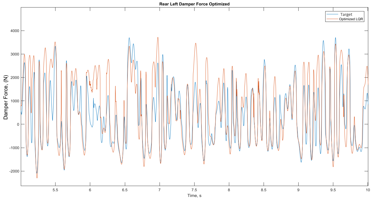
Figure 23: Rear left damper force time history curve of particle swarm optimized clipped optimal controller and supplier controller
