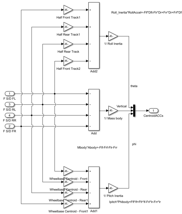
Figure 77: Vehicle body Equations of motion (48), (49), & (50) Simulink® model
