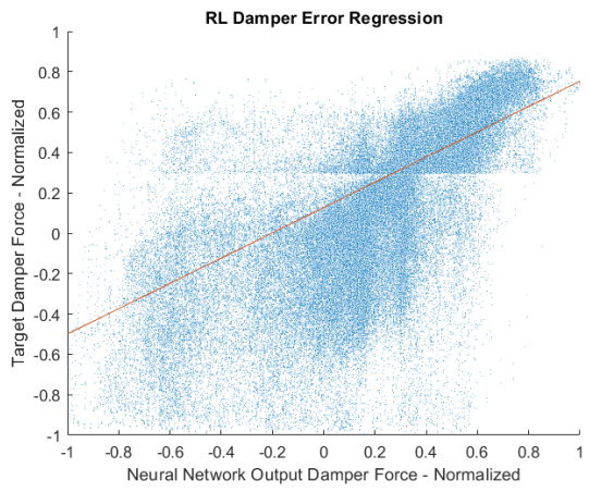
Figure 68: Linear regression plots between neural network controlled and supplier controlled dampers at each vehicle corner.
