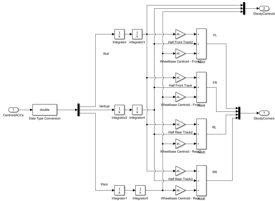
Figure 78: Centroid accelerations to corner displacement conversion Simulink® block
