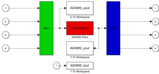
Figure 59: Block diagram within adams_sub block
