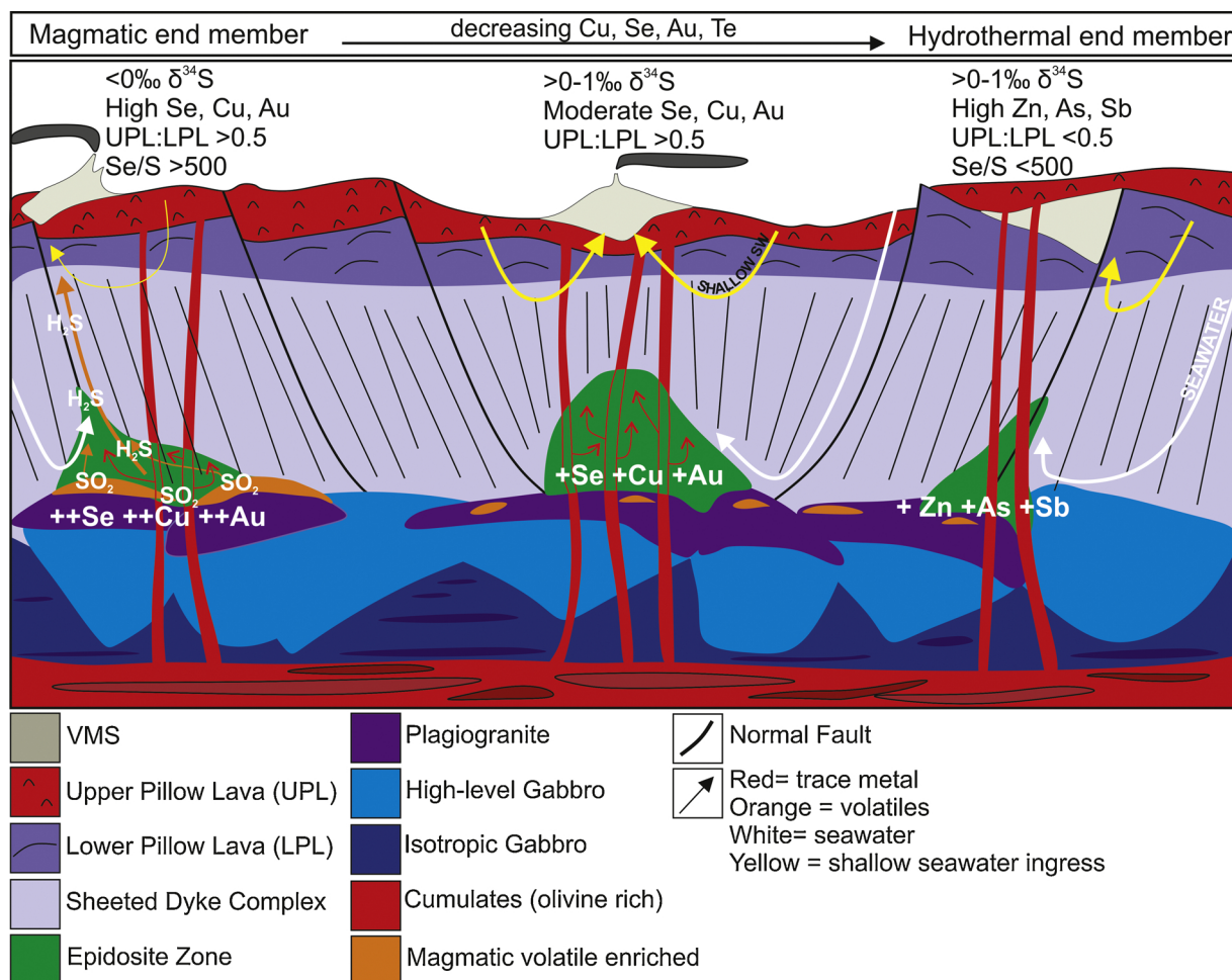
Fig. 13. Summary of VMS formation in the Troodos hydrothermal systems. Three scenarios explaining the transition from magmatic to hydrothermal end member VMS. (A) Both an UPL (Se, Cu, Au) source and magmatic volatile influx. VMS formed are enriched in Se, Cu, Au (and other magmatophile elements), exhibit a high UPL-LPL ratio and Se/S ratios >500 (Table 6A) and may exhibit negative \delta^{34}\text{S} values. The yellow arrow indicates minor shallow seawater circulation. (B) Same as scenario A but with no evidence of magmatic volatile influx, or volatile influx has been subsequently overprinted by a seawater signature. Selenium, Cu and Au are enriched and UPL-LPL ratio remains elevated but \delta^{34}\text{S} values <0\text{‰} are absent. The shallow circulation of seawater is variable and denoted by yellow arrows. (C) Metals are sourced from a LPL source with minimal/no volatile influx. VMS are relatively enriched in Zn, As and Sb and exhibit a low UPL-LPL ratio and low Se/S <500 . \delta^{34}\text{S} values are the same as B; at or above the Troodos magmatic mean (0–1‰). (For interpretation of the references to colour in this figure legend, the reader is referred to the web version of this article).
