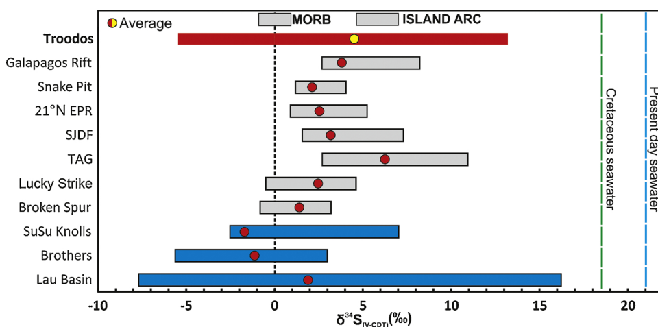
Fig. 10. Comparison of \delta^{34}\text{S} of VMS deposits in Troodos (red bar) with active seafloor hydrothermal systems (pyrite, marcasite, sphalerite and chalcopyrite). Troodos (This study (n = 180), Hannington et al., 1998; Keith et al., 2016a; Pedersen et al., 2017), Galapagos Rift (Knott et al., 1995), Snake Pit (Kase et al., 1990), 21°N East Pacific Rise (EPR) (Arnold and Sheppard, 1981; Woodruff and Shanks, 1988), Southern Juan de Fuca (SJDF) (Shanks and Seyfried, 1987), Trans-Atlantic Geotransverse Field (TAG) (Friedman, 1998; Gemmell and Sharpe, 1998; Herzig et al., 1998b), Lucky Strike (Rouxel et al., 2004), Broken Spur (Butler et al., 1998; Duckworth et al., 1995), SuSu Knolls (Yeats et al., 2014), Brothers (de Ronde et al., 2003d, 2005), Lau Basin (Herzig et al., 1998a). Red/yellow dots represent the average \delta^{34}\text{S} value. Grey box represents the \delta^{34}\text{S} composition of island arc lavas (Herzig et al., 1998a). Dashed lines: Black average MORB \delta^{34}\text{S} composition, blue modern day seawater, green Cretaceous seawater (Kampschulte and Strauss, 2004). (For interpretation of the references to colour in this figure legend, the reader is referred to the web version of this article).
