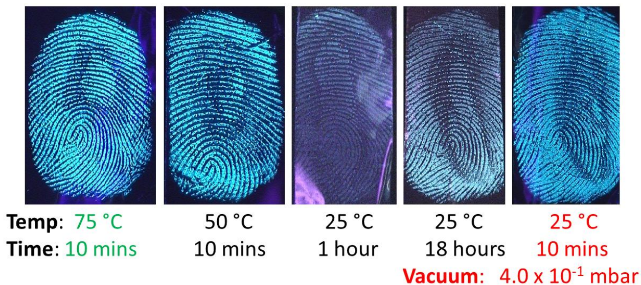
Figure 1. Optimisation of pyrene fuming conditions using fresh fingerprints on aluminium foil, and visualised with 313 nm UV radiation. The optimal fingerprint fuming treatment (highlighted in green) was exposure to pyrene fumed at 75 °C for 10 minutes. Heating at 25 °C was insufficient to deliver good visualisation, unless vacuum conditions were also applied (highlighted in red).
