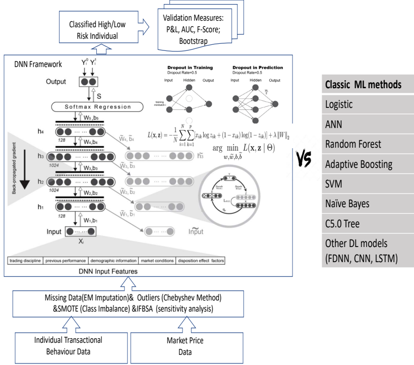
Figure 4: Topology of the DNN using sDA with 4 hidden layers with 128, 1024, 1024, 128 hidden units each. The output layer predicts class probabilities based on the output of the last dropout layer using the softmax function. DNN predictions are compared to ML benchmarks for assessing predictive performance.
