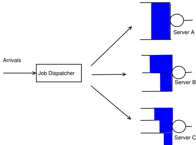
Figure 1.3: A multi-server PS model
