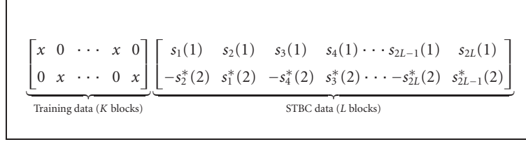
FIGURE 2: Complete frame for two transmit antennas and single receive antenna case.
