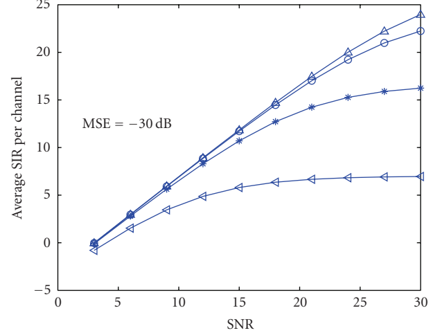
FIGURE 4: Plot of average SIR per channel versus SNR for MSE = -30 dB (graphs are plotted for \sigma_\omega^2 = 0, (2\pi/1000)^2, (2\pi)^2/10^5, (2\pi/100)^2 from uppermost to downmost, resp.).
