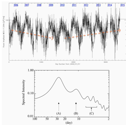
Figure 3. (top) Long-term intensity variation of Schumann resonance waves in the period of 2006-2015. (bottom) Periodogram of the long-term intensity variation of Schumann resonance waves.
