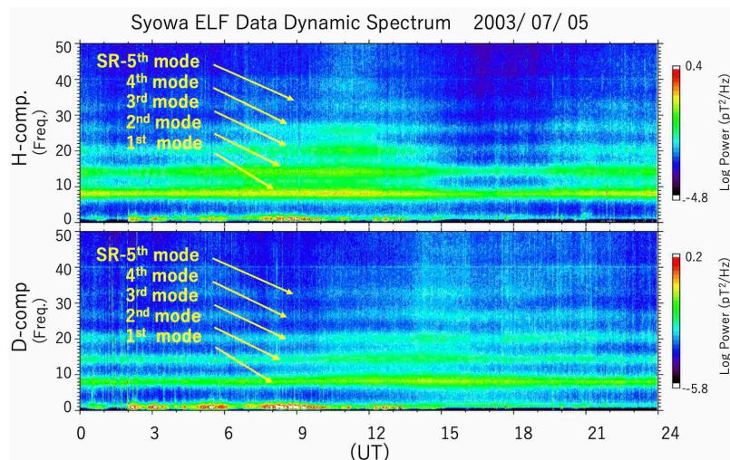
Figure 2. 1-day dynamic spectrum of the ELF waves measured at Syowa station. In the frequency range of 8-45 Hz, spectral peaks of Schumann resonance can be clearly seen.
