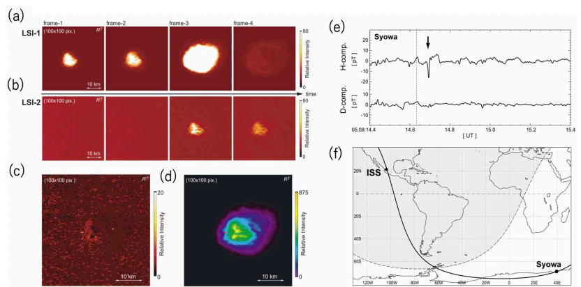
Figure 4. (a) Lightning and sprite images measured by the GIMS wideband camera (LSI-1) and narrowband camera (LSI-2). (c), (d) Results of the image subtraction between LSI-1 and LSI-2. Dot structures corresponding to sprite emissions can be confirmed in Figure 4(d). (e), (f) ELF waves excited by the sprite-producing lightning discharges.
