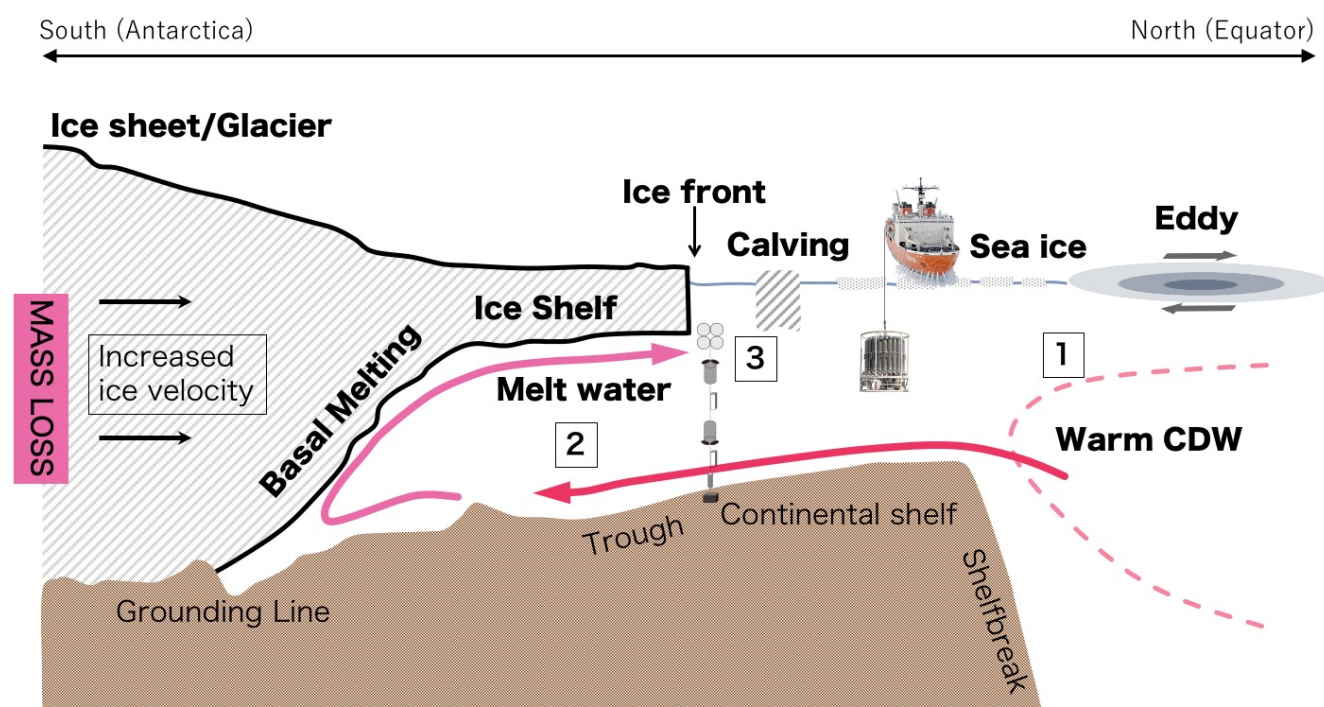
Figure 1. Conceptual diagram of ice sheet-ocean interaction which this proposal focuses on. Numbers 1 to 3 in the figure indicate areas and processes listed in this proposal.
