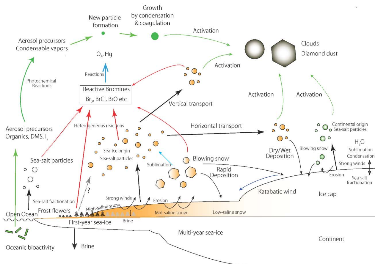
Fig.1 Schematics of atmospheric sea-salt and halogen cycles in polar regions. Dotted arrows indicate the speculated processes.
