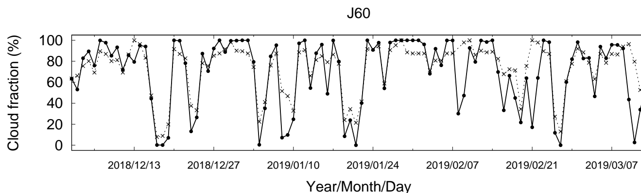
Figure 1: Temporal variation of daily-averaged cloud fractions during JARE 60 from 1 December 2018 to 13 March 2019. Solid and dashed lines correspond to the ceilometer and the visual observations, respectively.
