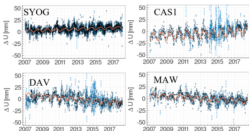
Figure 1. The time series of observed vertical displacement of each IGS station in East Antarctica; Syowa, Mawson, Davis, and Casey, estimated by PPP.
