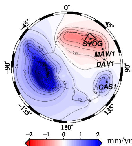
Figure 2. Spatial distribution of the estimated vertical elastic deformation rate due to recent snow mass change. The snow mass change is estimated from GRACE.
