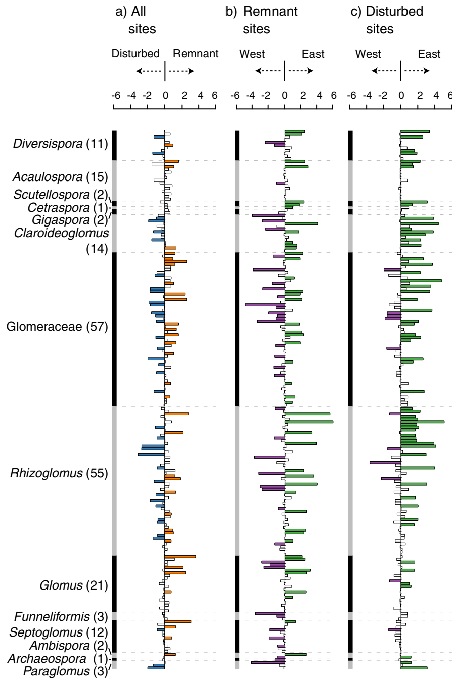
FIG. 3. Differential abundance (on log 2 scale) for each of the 199 OTUs (bars) between (a) remnant (orange) or disturbed (blue) site histories for all sites and between the western (purple) or the eastern (green) side of the precipitation gradient for (b) only remnant sites and (c) only disturbed sites. Filled bars denote OTUs with a significant difference in abundance between the two groups being compared. The order of bars is the same for all panels, and is sorted by the phylogenetic relationships of each OTU's taxonomic attribution (genus level except the family Glomeraceae) as determined from Appendix S1: Fig. S1, with the number of OTUs represented in each taxon in parentheses. OTUs from different taxonomic groups are denoted by alternating black and gray vertical bands on the left side of each panel, and by dashed horizontal lines.
