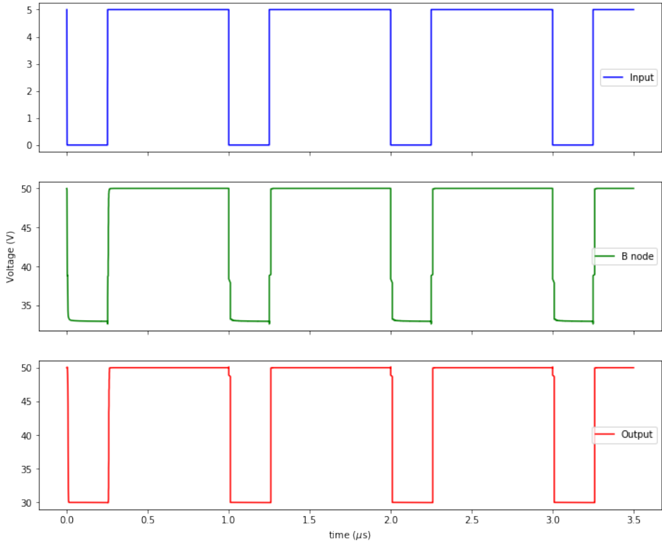
Figure 4.16: Simulated results of the proposed Level Shifter
