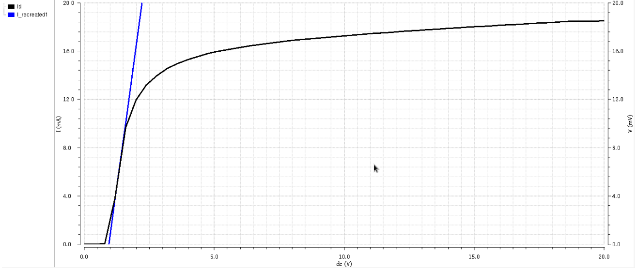
Figure 7.5: measure I_D (black) and recreated I_D (blue) with only K parameter for NMOS50M
