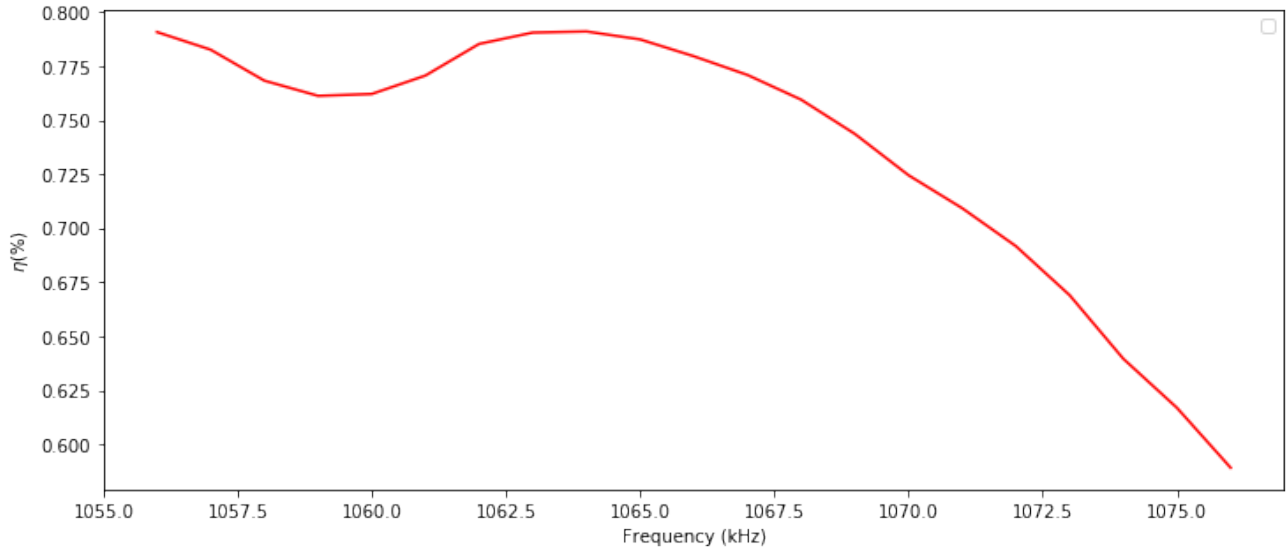
Figure 4.26: \eta vs. frequency when the power supply is connected to 20 V
