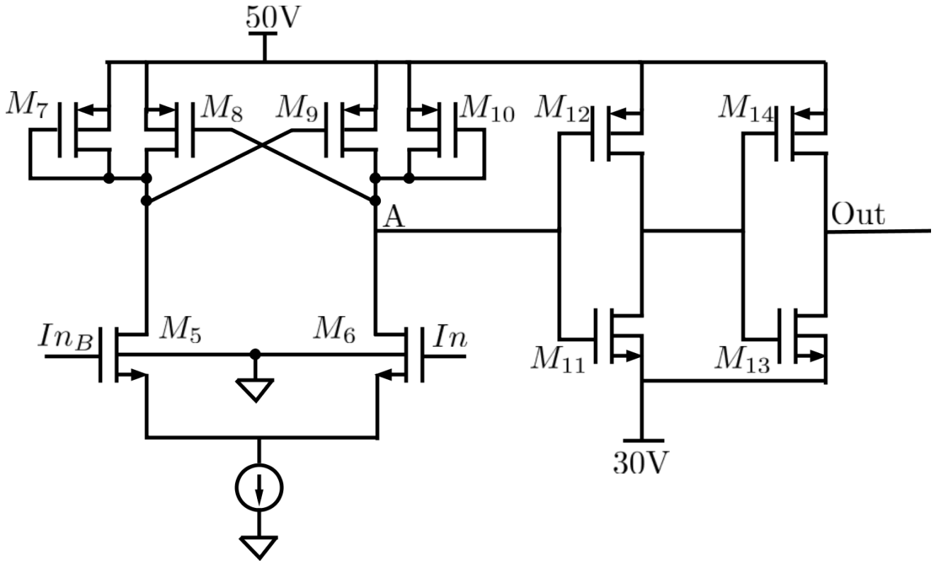
Figure 4.13: Level Shifter used in [3] and [4]
