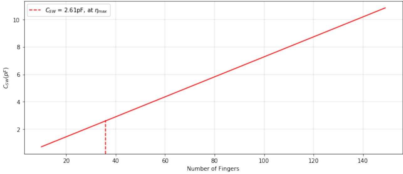
Figure 4.21: Switch capacitance vs number of fingers for transducer array used in section 3.3
