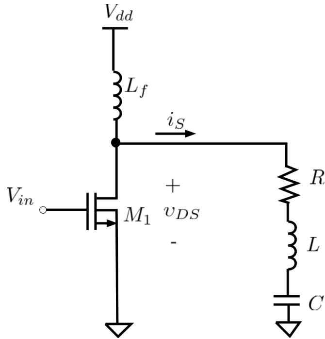
Figure 2.13: Schematic of class E amplifier [14]
