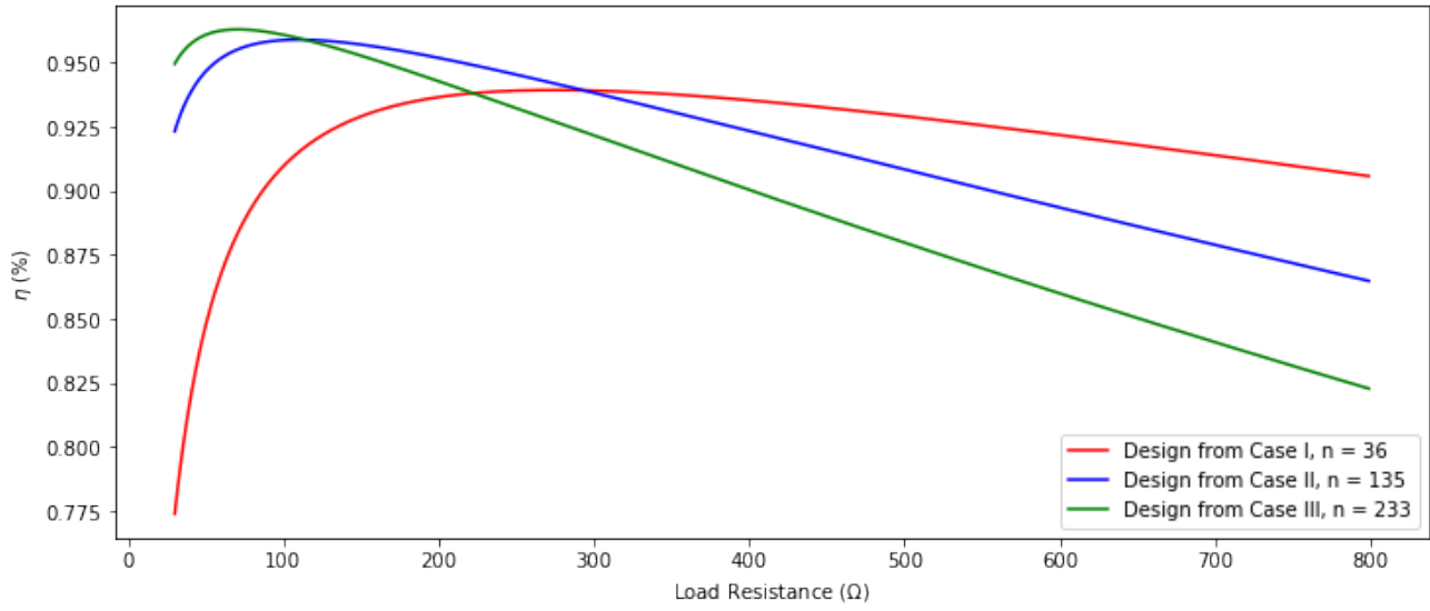
Figure 4.24: Power efficiency vs load resistance
