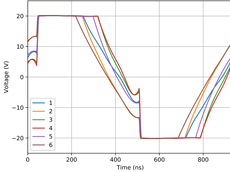
Figure 3.7: Sim 3 Output voltages
