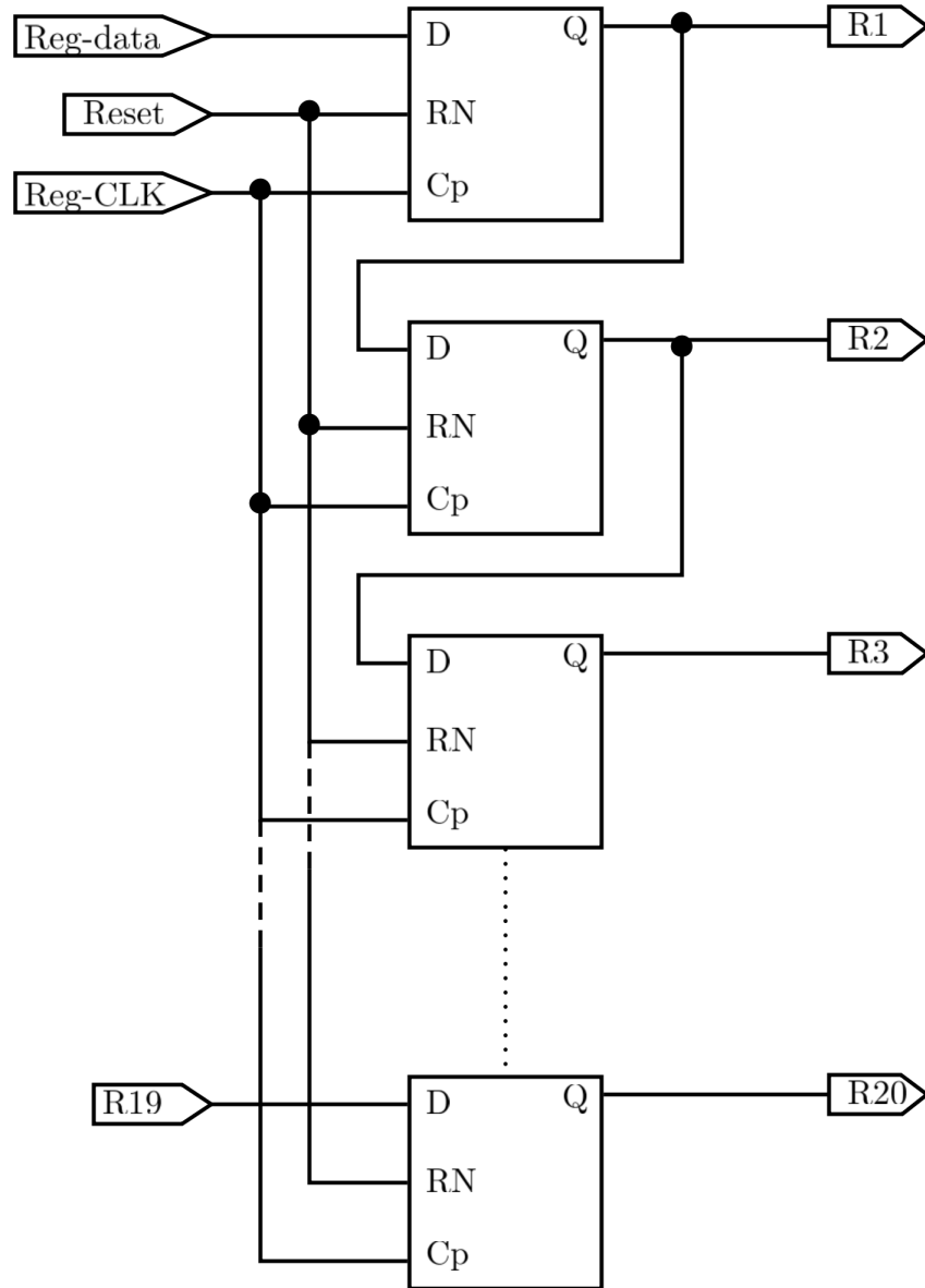
Figure 4.4: Schematic of the 20-bits Register
