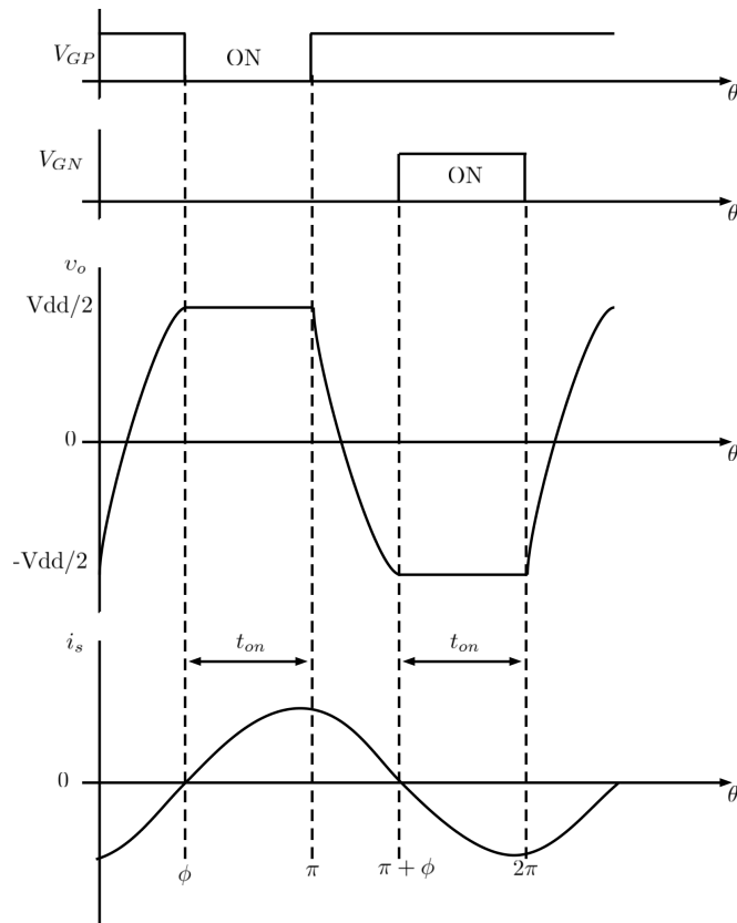
Figure 2.17: Class DE waveform
