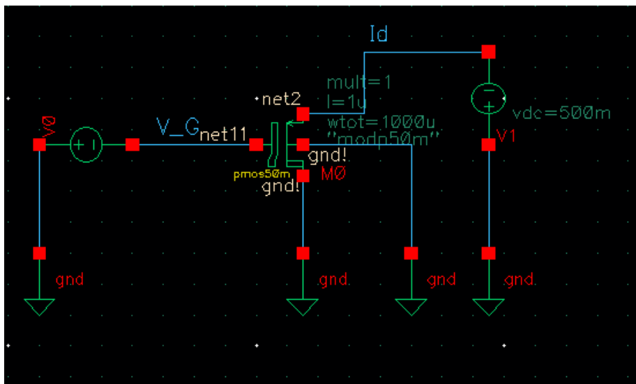
Figure 7.7: Circuit setup to extract parameters for PMOS50M
