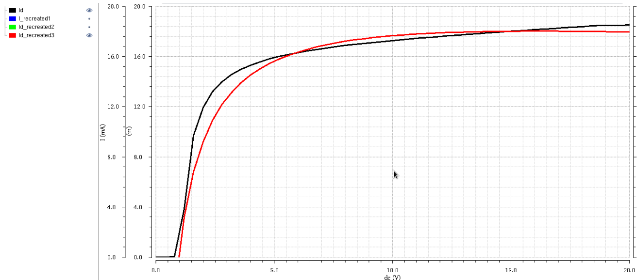
Figure 7.6: Recreated I_D using the extracted parameters (red) and the measure I_D (black)
