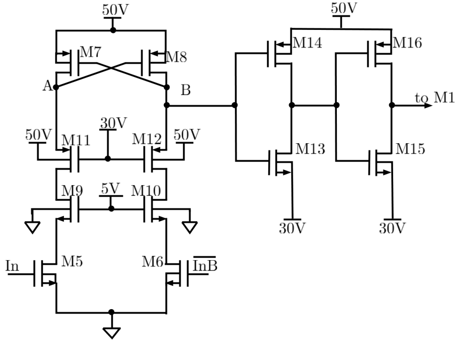
Figure 4.14: Schematic diagram for the 30-50 V level shifter
