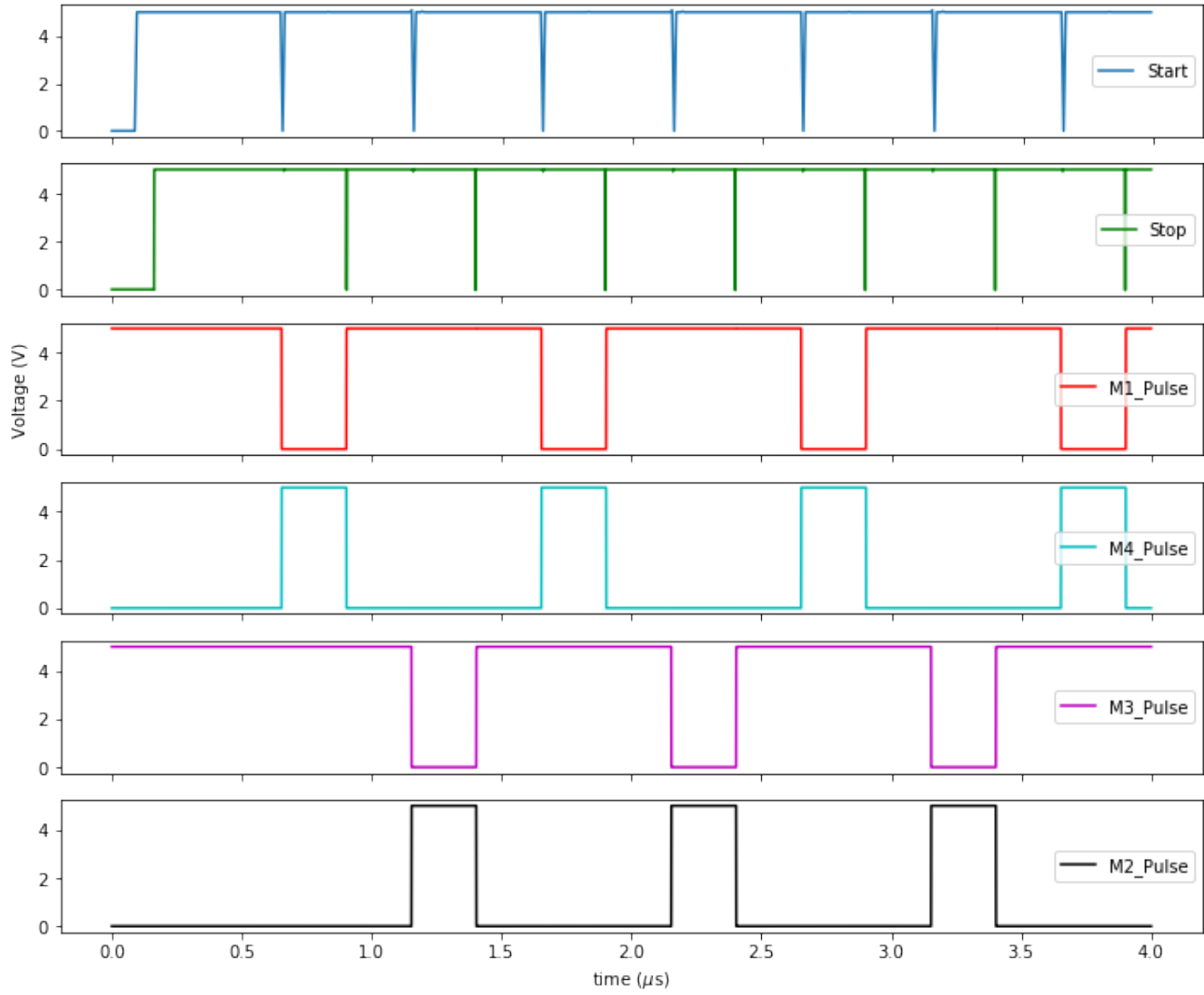
Figure 4.11: Outputs of the Pulse Train Generator
