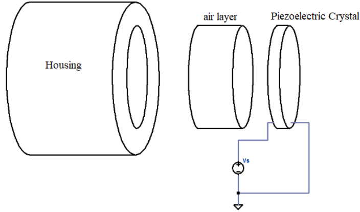
Figure 2.1: Exploded view of a transducer [3]
