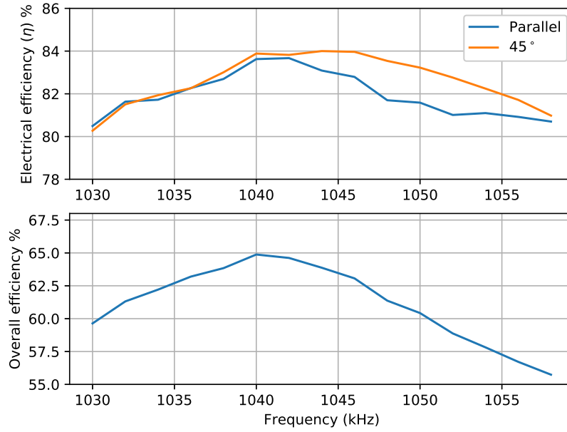
Figure 3.13: Array electrical efficiency ( \eta ) and overall combined electrical-acoustic efficiency vs. frequency.
