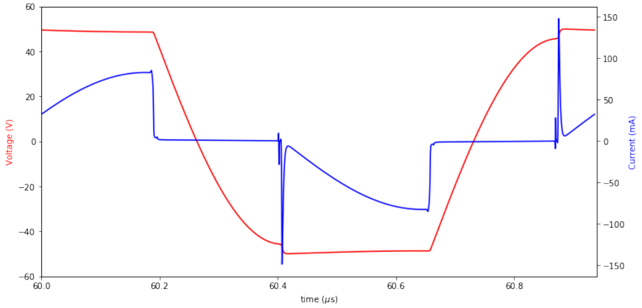
Figure 6.12: Output Voltage and Current of transducer 6
