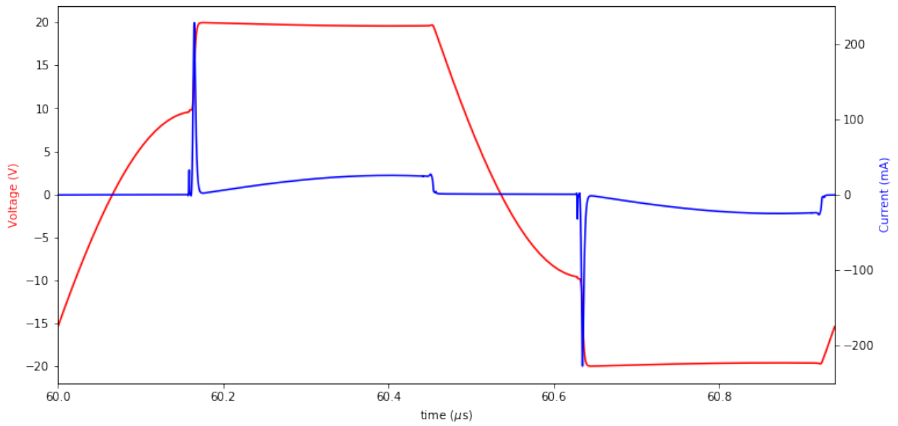
Figure 6.4: Output Voltage and Current of transducer 4
