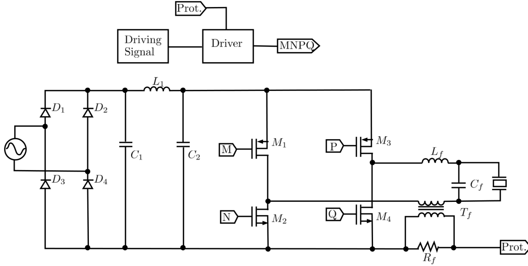
Figure 2.8: Schematic of class D Amplifier proposed by Agbossou [15]
