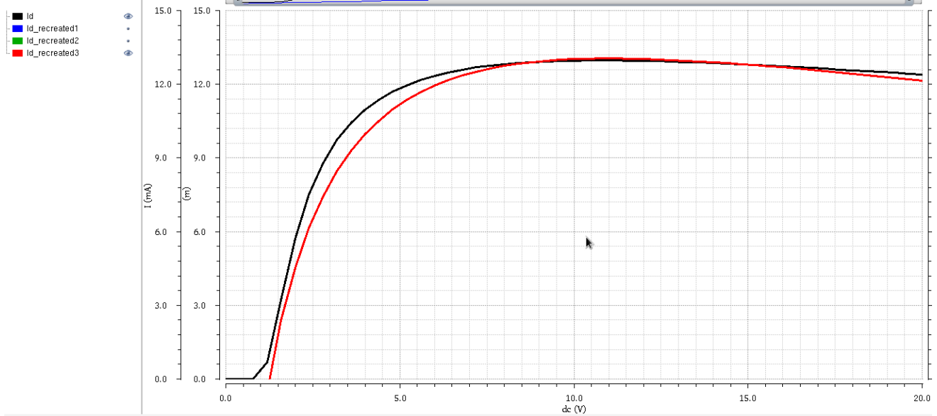
Figure 7.8: Recreated I_D for PMOS using the extracted parameters (red) and the measure I_D (black)
