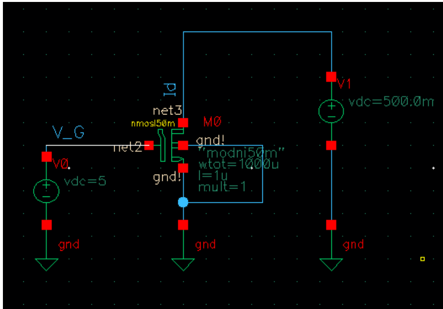
Figure 7.4: Circuit setup to extract parameters for NMOS50M
