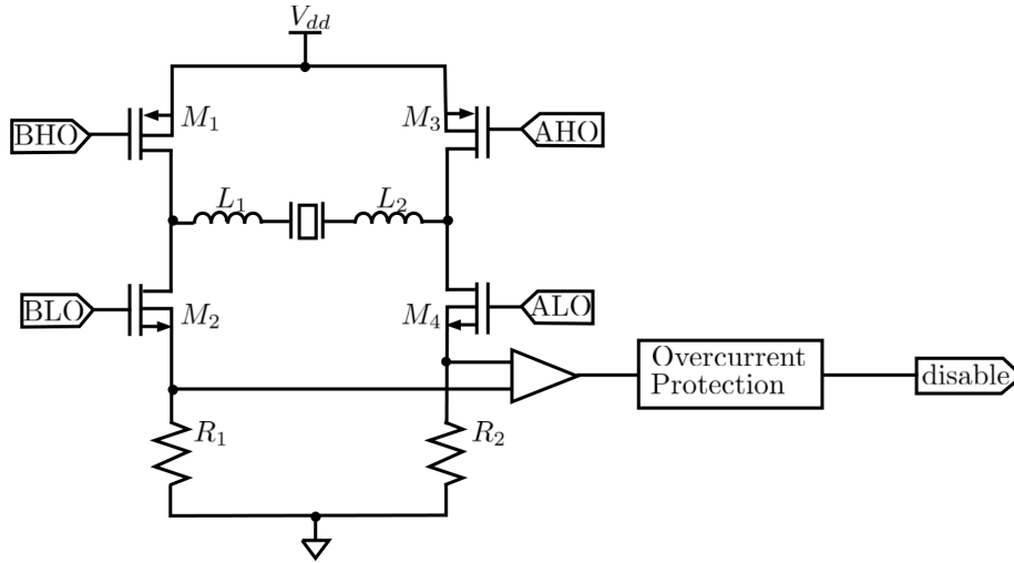
Figure 2.9: Schematic of a class D amplifier proposed by Yang and Xu [16]
