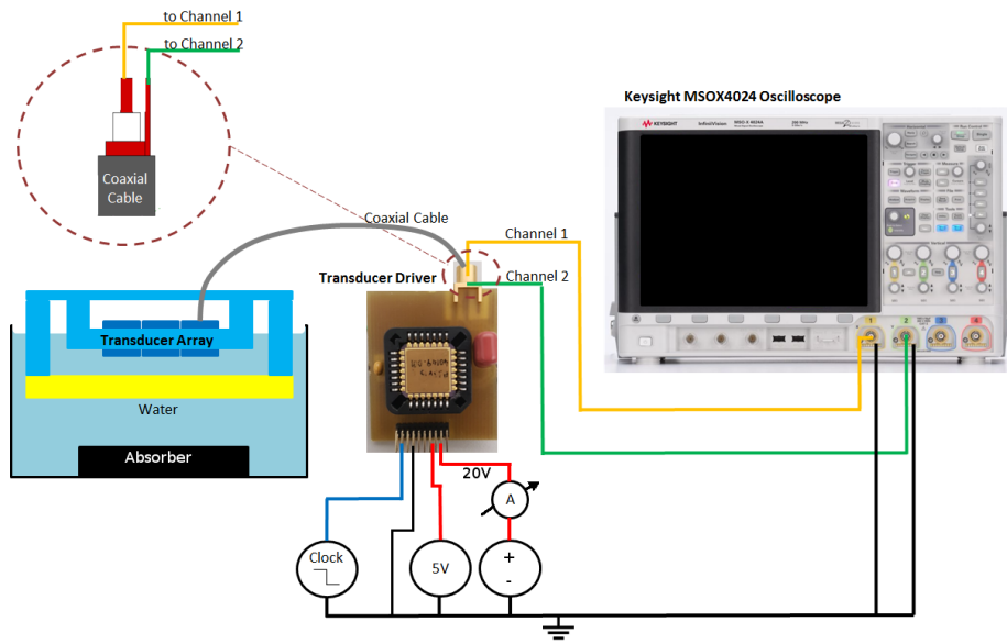
Figure 3.8: Experimental Setup
