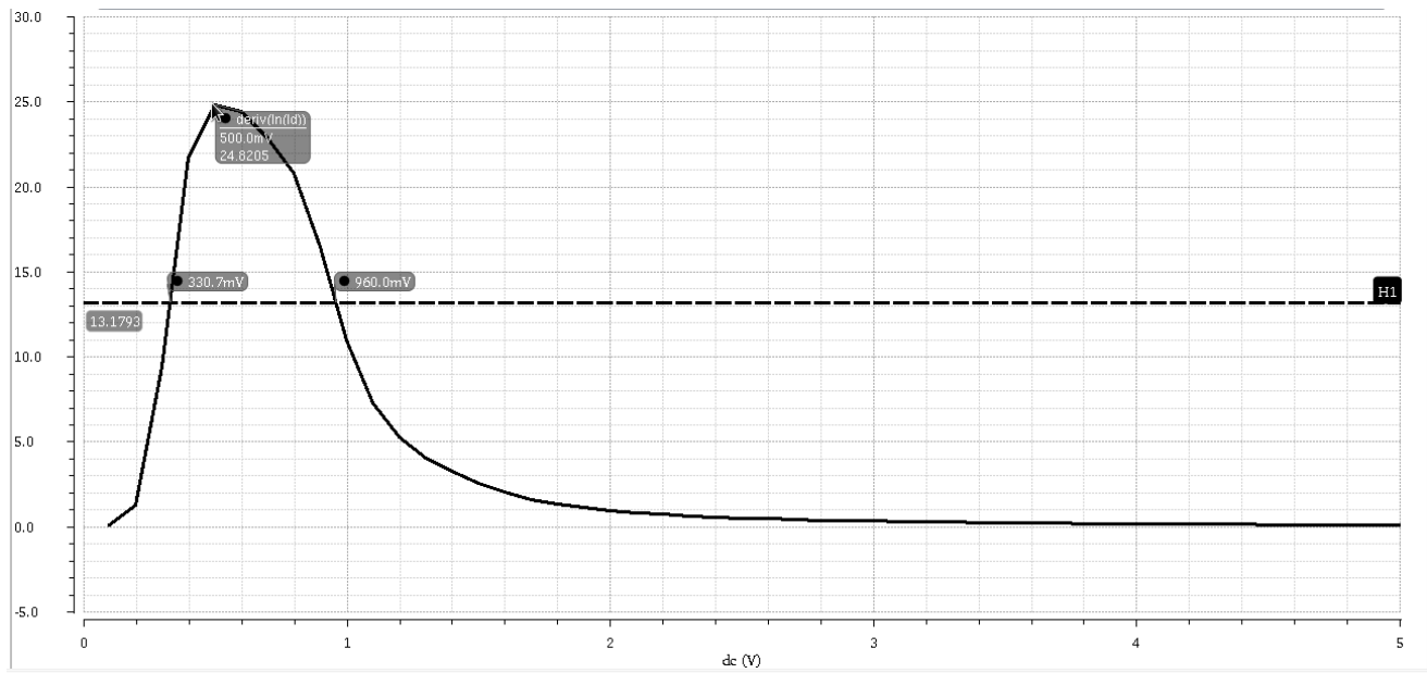
Figure 7.3: Obtaining V_t for NMOS50M
