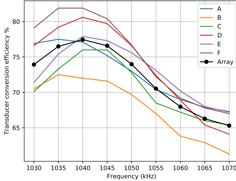
Figure 3.11: Transducer conversion efficiency as a function of frequency.
