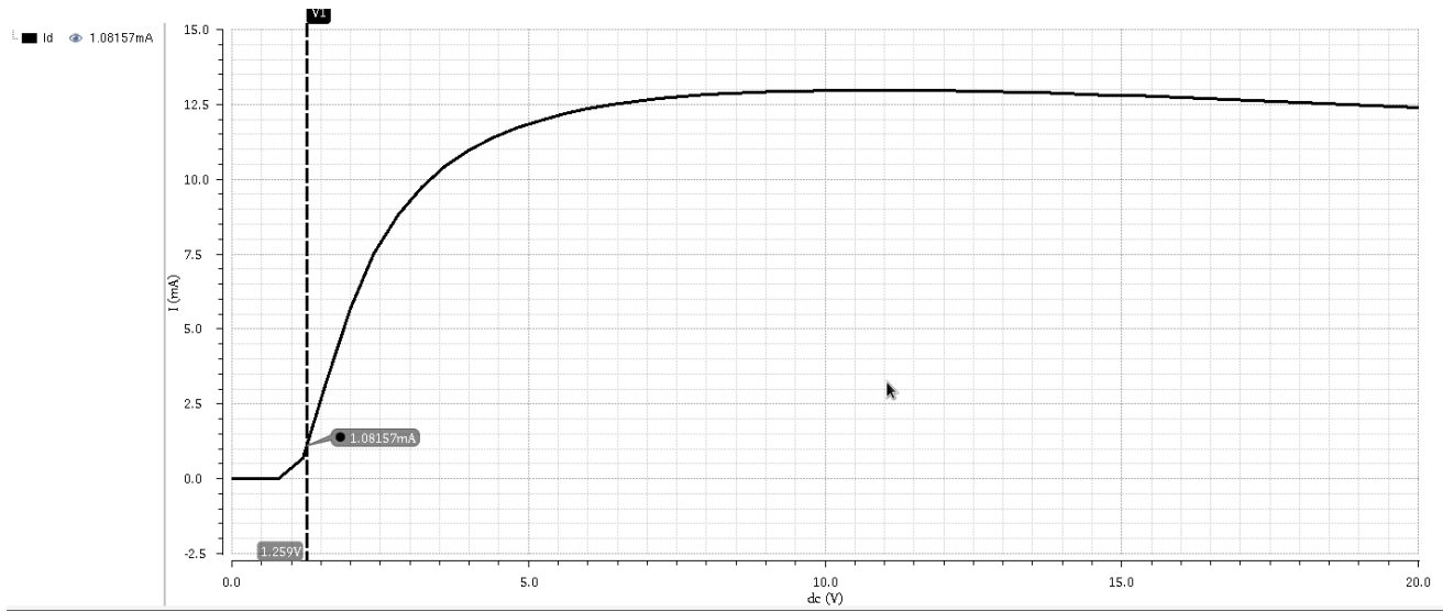
Figure 7.2: I_D vs V_{GB} for NMOS50M
