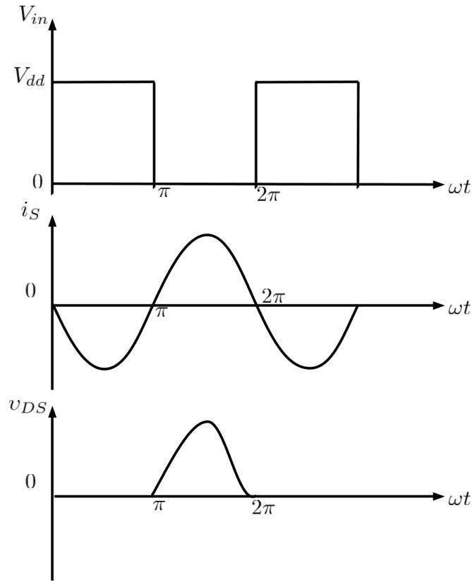
Figure 2.14: Waveforms of class E amplifier [14]
