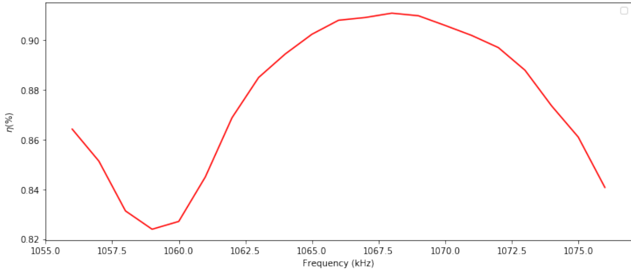
Figure 4.29: \eta vs. frequency when using 50 V voltage supply
