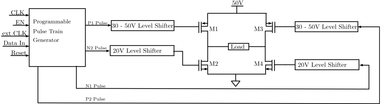
Figure 4.1: Proposed transducer driver
