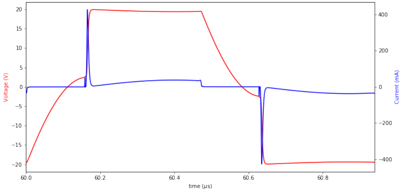
Figure 6.5: Output Voltage and Current of transducer 5
