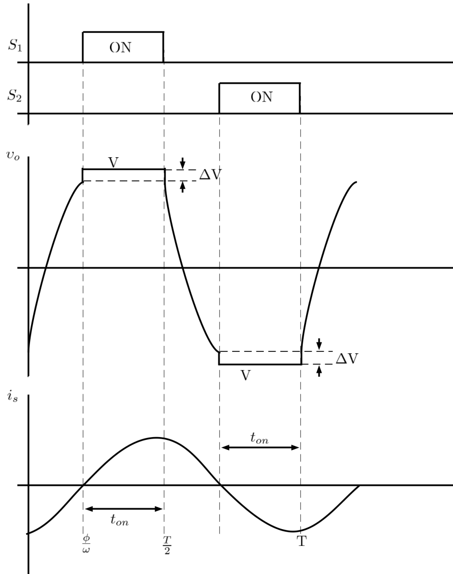
Figure 3.2: Class DE output waveform outside optimum condition
