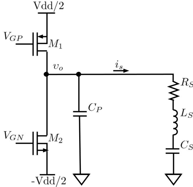
Figure 2.16: Class DE simplified circuit
