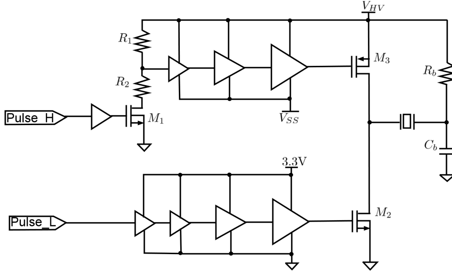
Figure 2.12: Proposed Amplifier from O. Farhanieh [20]
