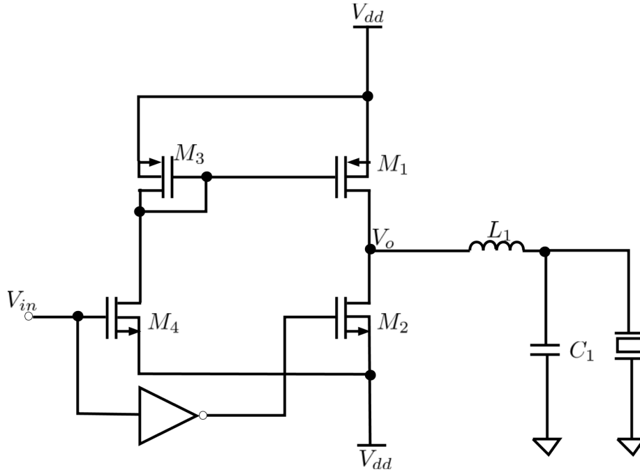
Figure 2.11: Schematic of LIPUS amplifier proposed in [22]
