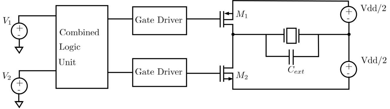
Figure 2.18: Overall system of Wai's design [3]
