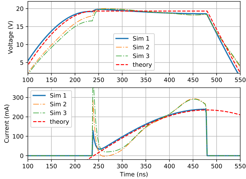
Figure 3.15: Output voltage and current waveforms for Transducer D.
