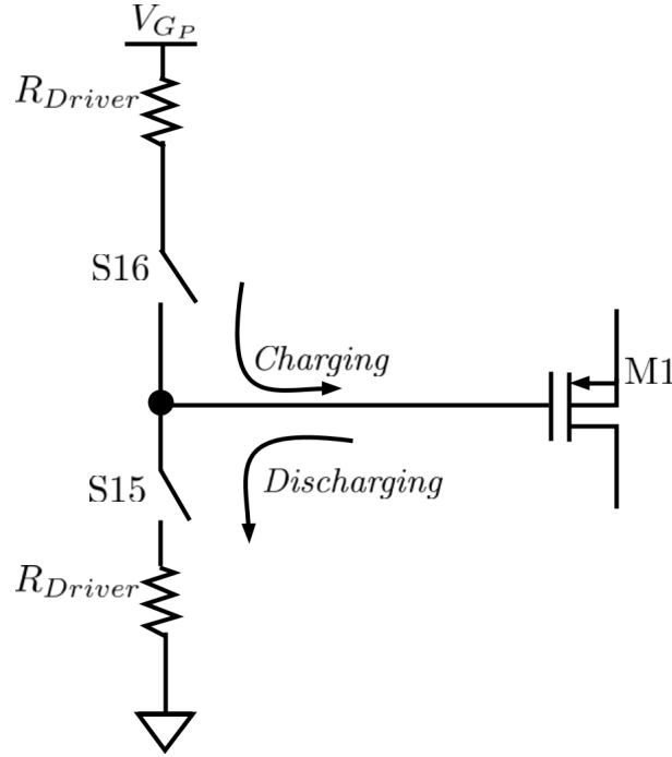
Figure 4.15: Simplified Gate Driving circuit
