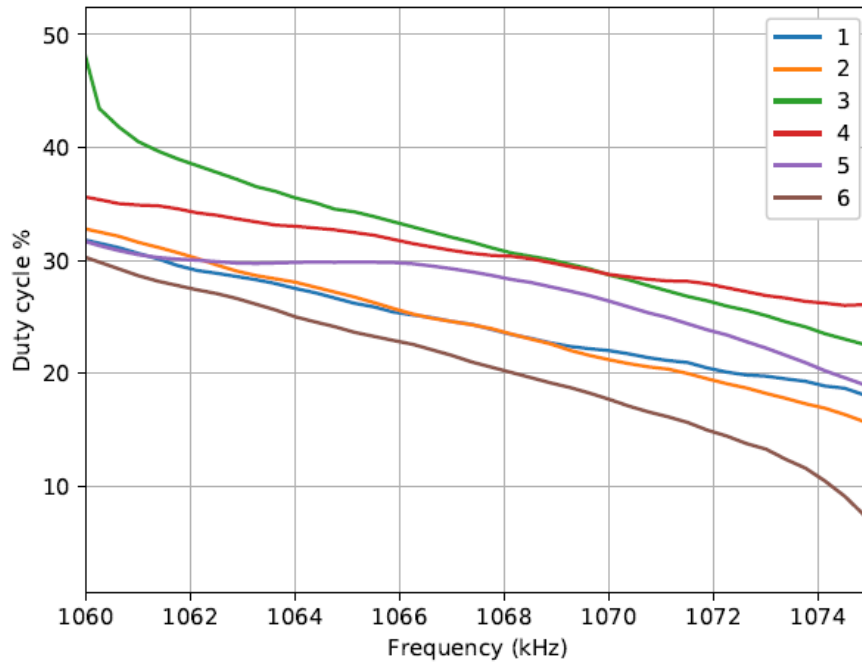
Figure 3.4: Optimum duty cycle vs frequency for the transducer array
