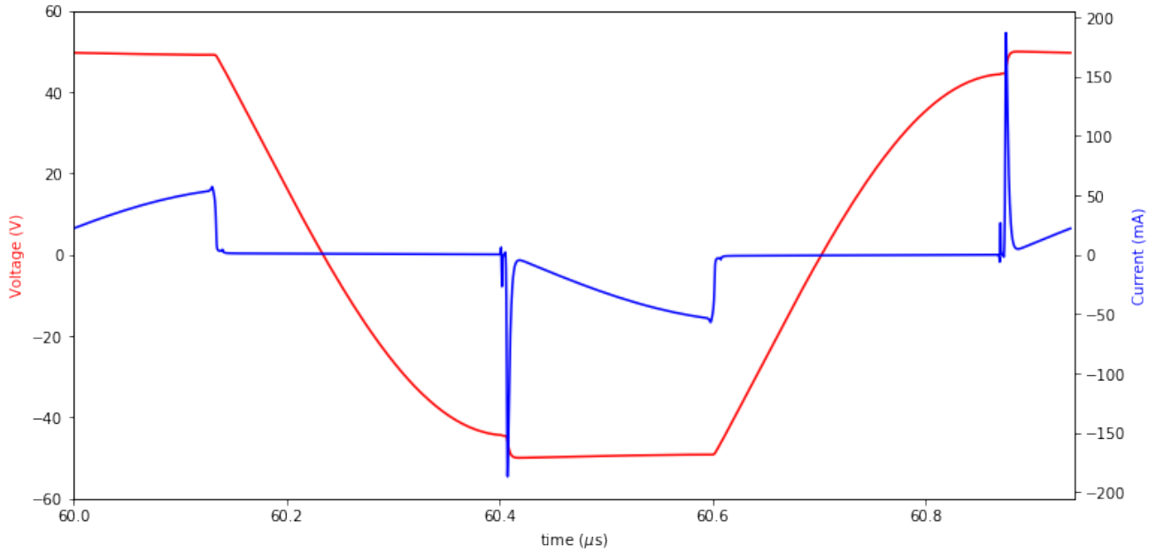
Figure 6.8: Output Voltage and Current of transducer 2
