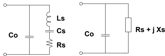
Figure 2.2: Piezoelectric transducer simplified equivalent circuit.
