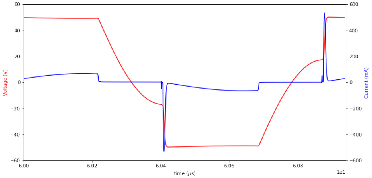
Figure 6.9: Output Voltage and Current of transducer 3
