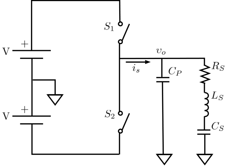
Figure 3.1: Simplified class DE circuit
