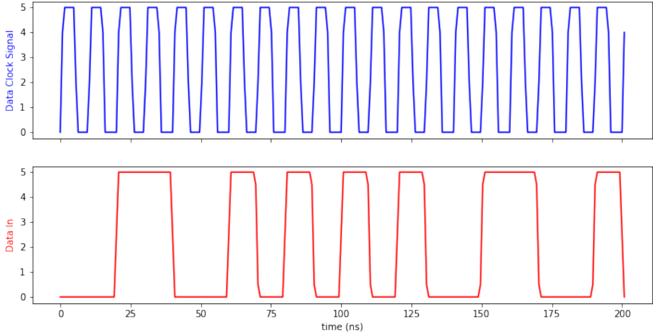
Figure 4.10: Simulation results for programming the DLU system
