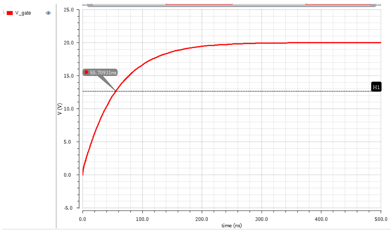
Figure 8.2: Gate capacitance charging curve
