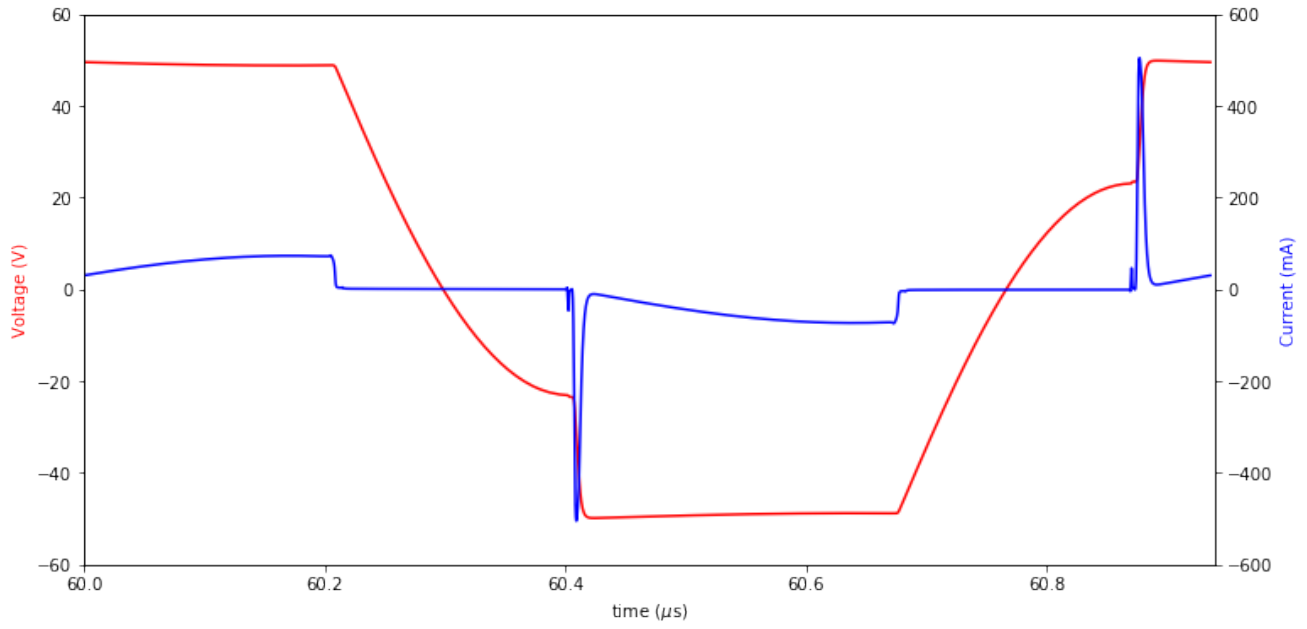
Figure 6.7: Output Voltage and Current of transducer 1
