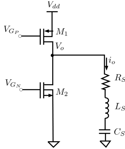
Figure 2.5: Schematic of class D amplifier[14]
