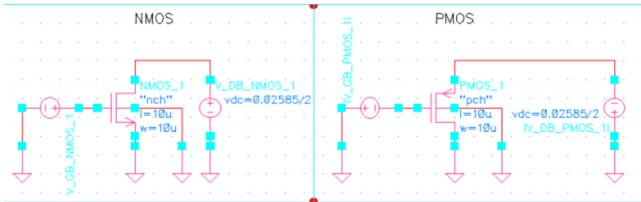
Figure 7.1: I_{SQ} and V_t extraction circuit
