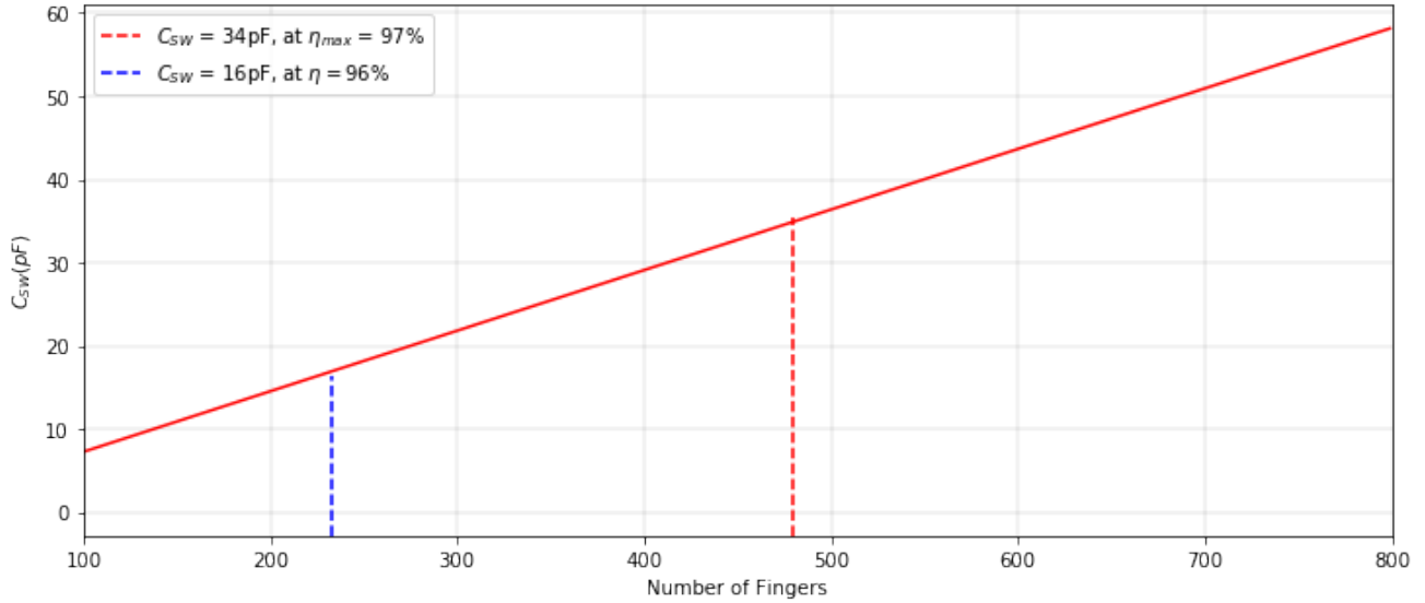
Figure 4.23: Switch capacitance vs number of fingers for transducer array used in section 3.4
