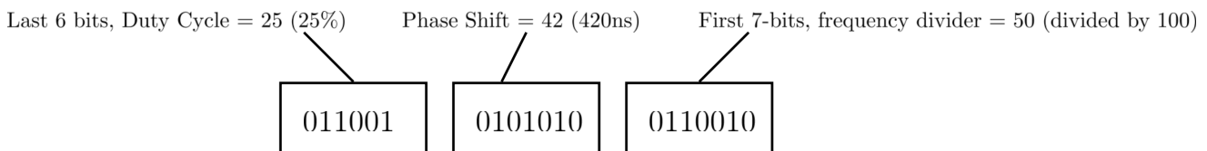
Figure 4.9: Data In Configuration
