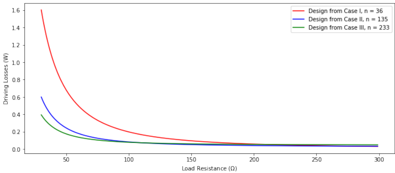
Figure 4.25: Power losses from all 3 cases
