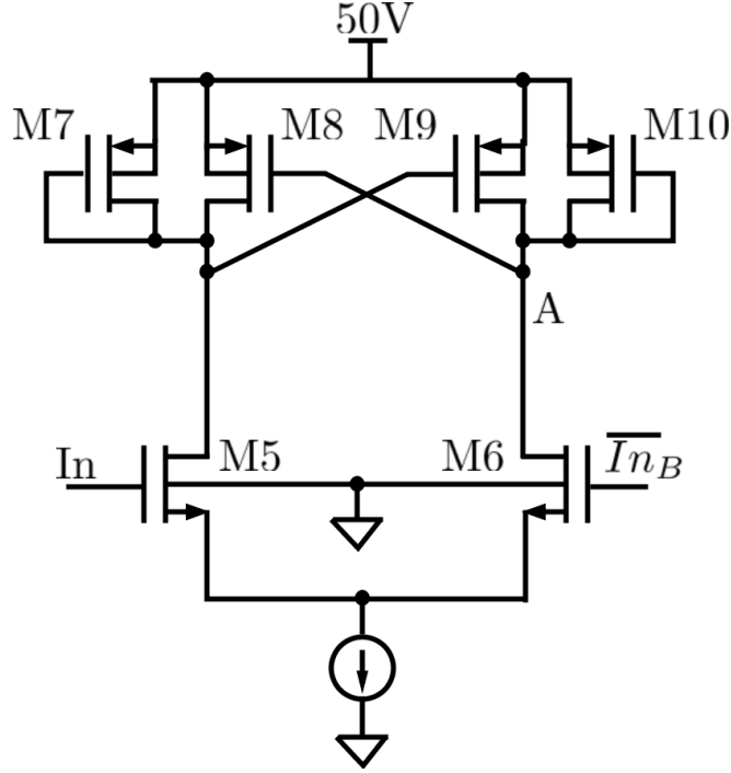
Figure 4.12: Schematic of a conventional level shifter
