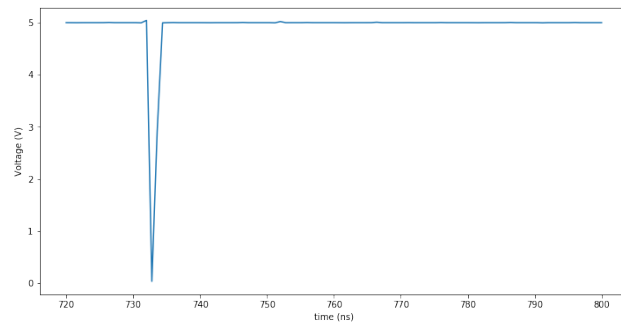
Figure 4.8: Zoomed view of RN pulse
