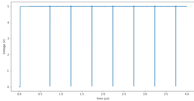
Figure 4.7: RN pulse for frequency divider
