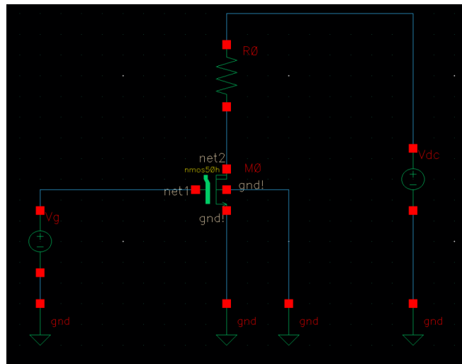
Figure 7.9: Simulation setup to extract the actual MOSFET on-resistance
