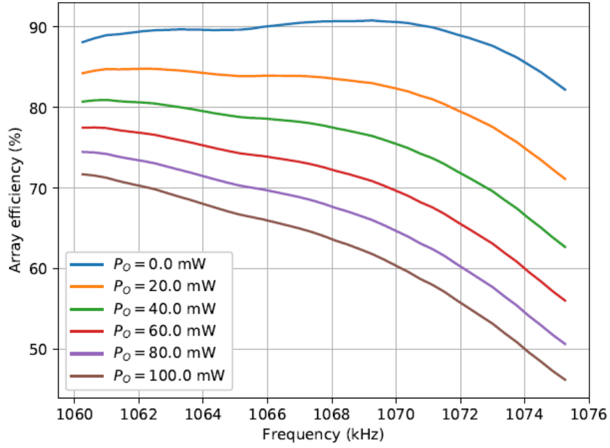
Figure 3.5: Power efficiency vs frequency for the transducer array with different driving power losses
