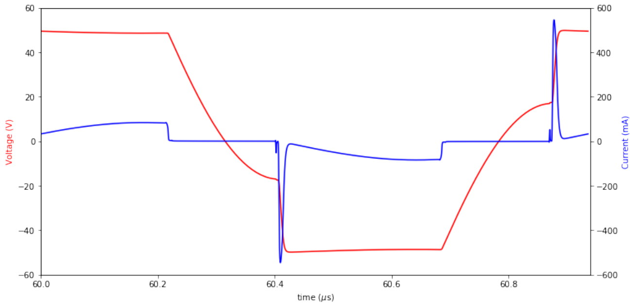
Figure 6.11: Output Voltage and Current of transducer 5
