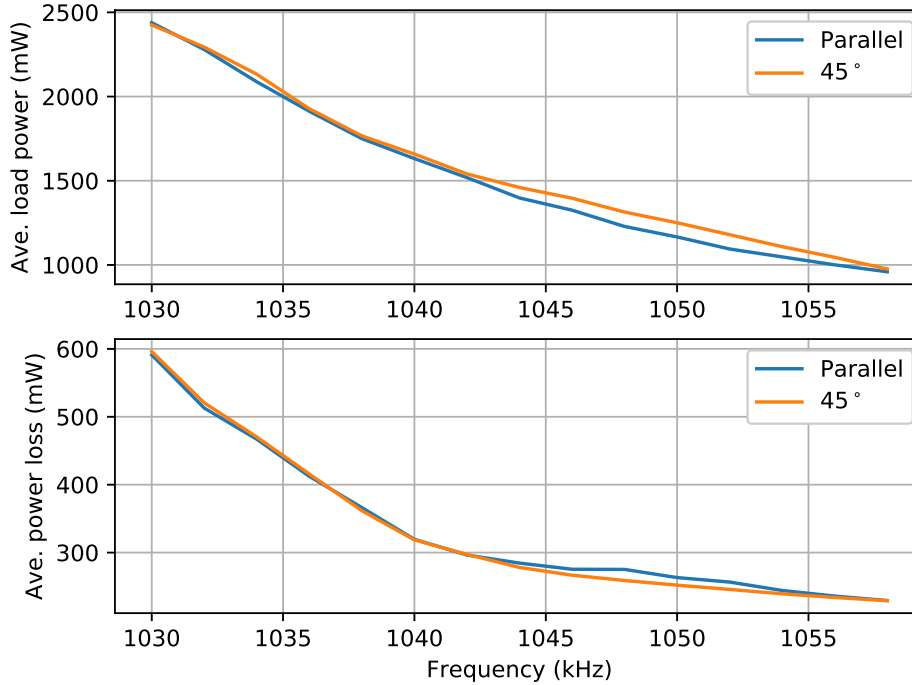
Figure 3.12: Electrical load power and losses vs. frequency
