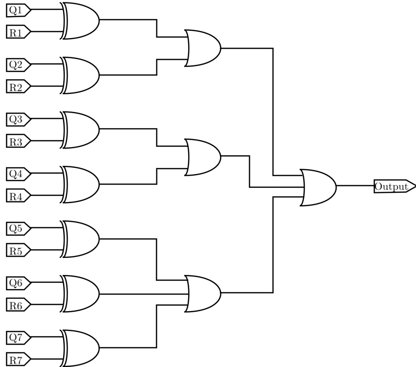
Figure 4.5: Schematic of the 7-bits Comparator
