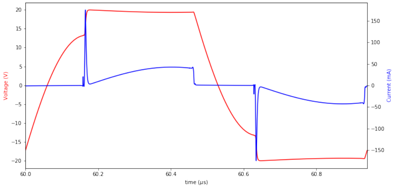
Figure 6.6: Output Voltage and Current of transducer 6
