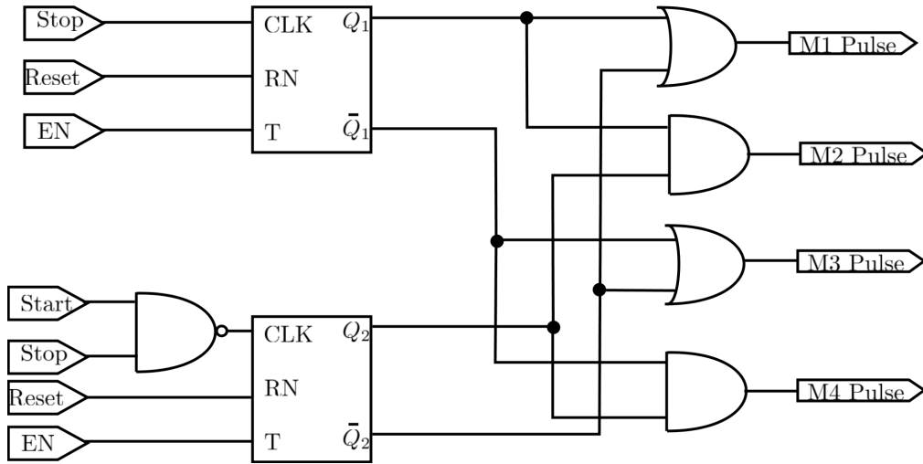
Figure 4.6: Schematic of the Output Block
