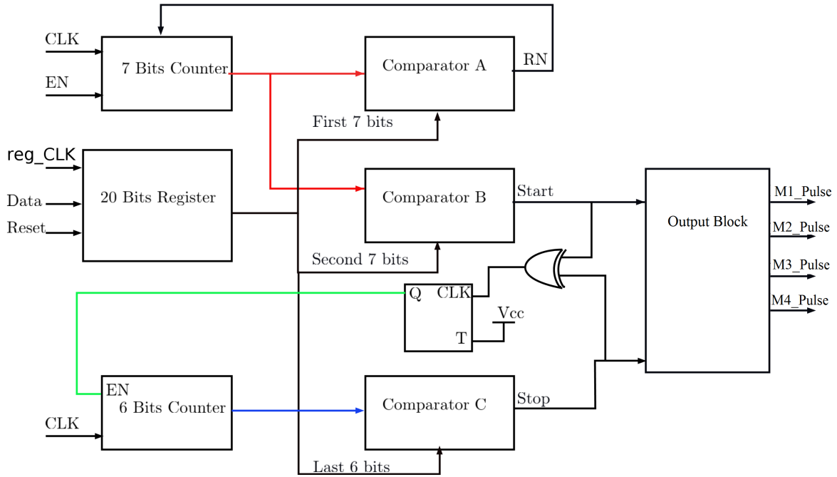
Figure 4.2: Block Diagram of the proposed Pulse Train Generator
