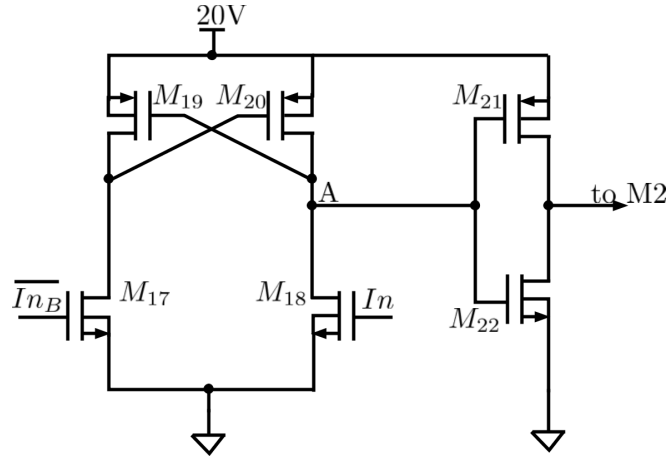
Figure 4.18: 20V Level Shifter design
