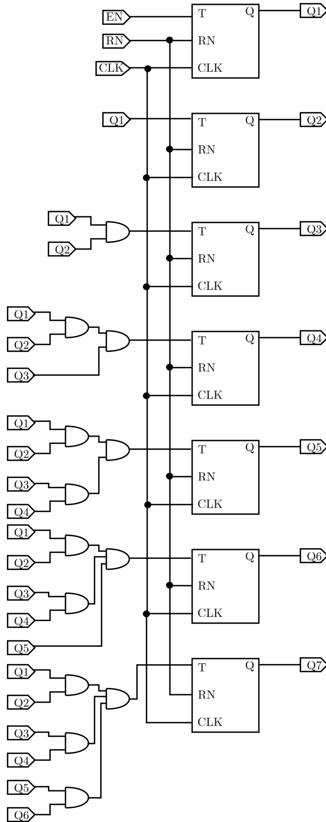
Figure 4.3: Schematic of the 7-bits counter
