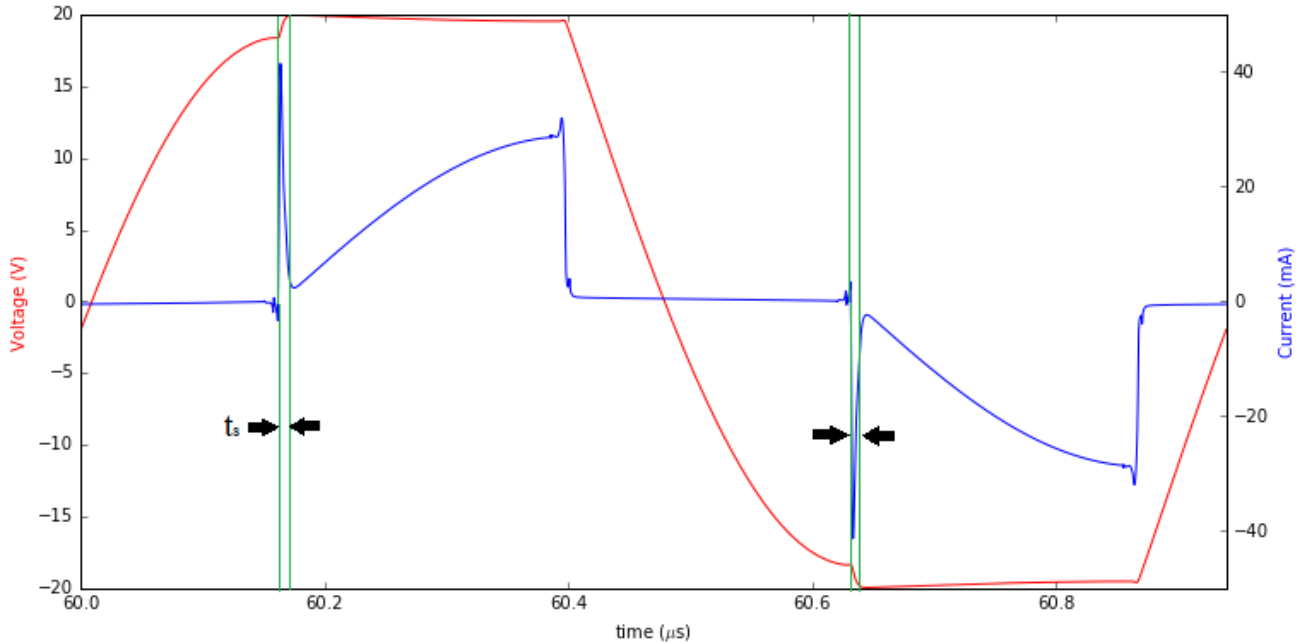
Figure 4.28: Extracting switching loss from simulation, red line is v_o , and blue line is i_s
