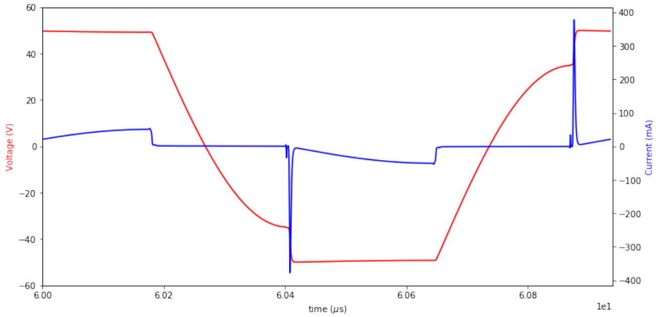
Figure 6.10: Output Voltage and Current of transducer 4
