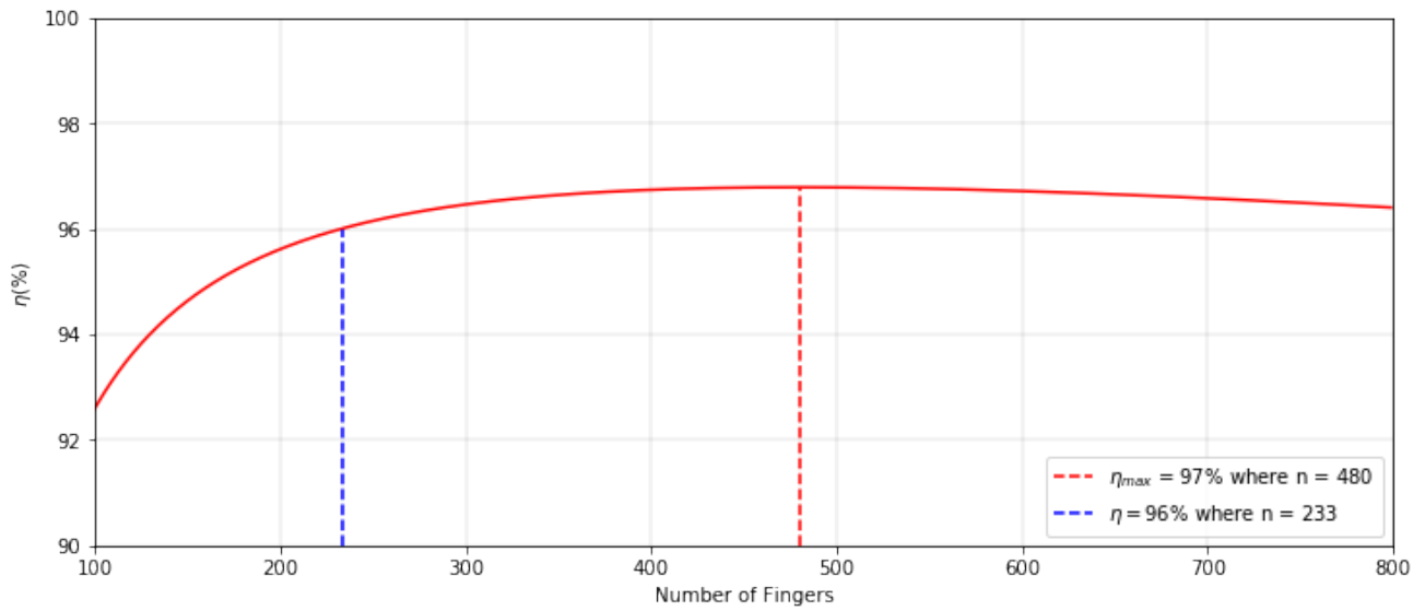
Figure 4.22: Power efficiency vs number of fingers for transducer array used in section 3.3
