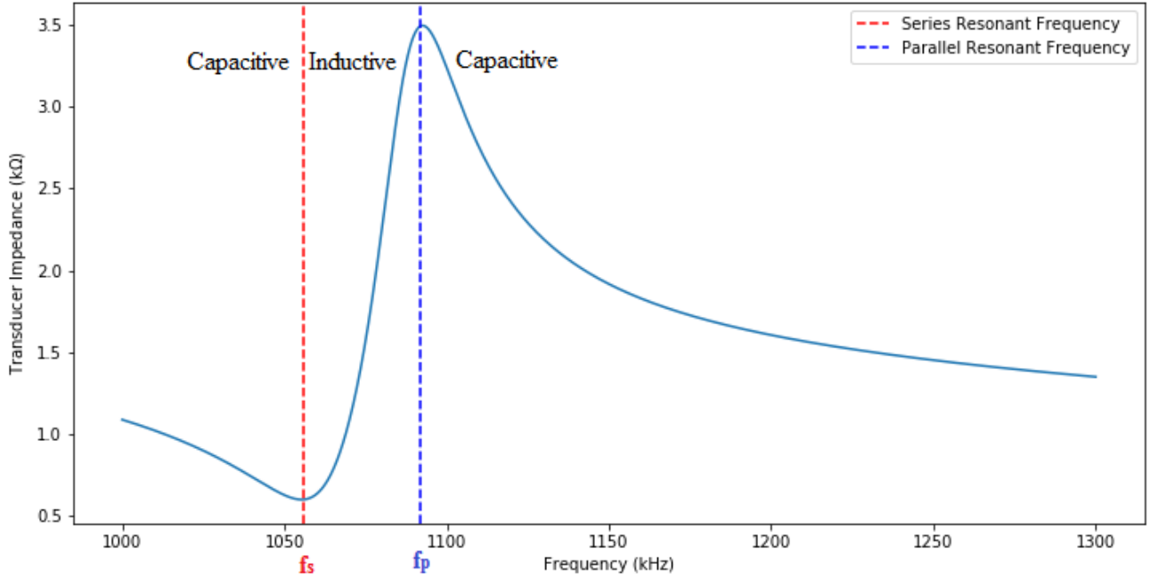
Figure 2.4: Magnitude of the Transducer Impedance vs Operating Frequency. f_s is the series resonant frequency, where as f_p is the parallel resonant frequency [15]
