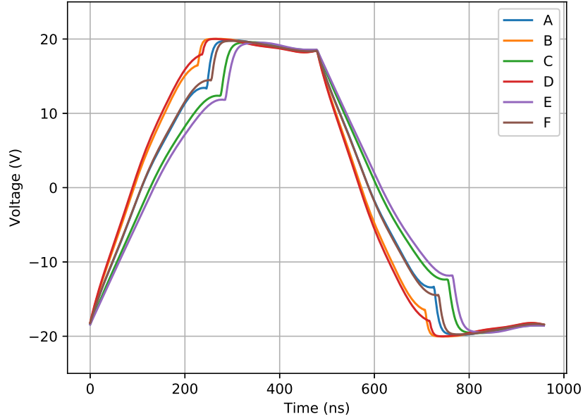
Figure 3.14: Output voltage for all transducers using the accurate transducer model (Sim 2).
