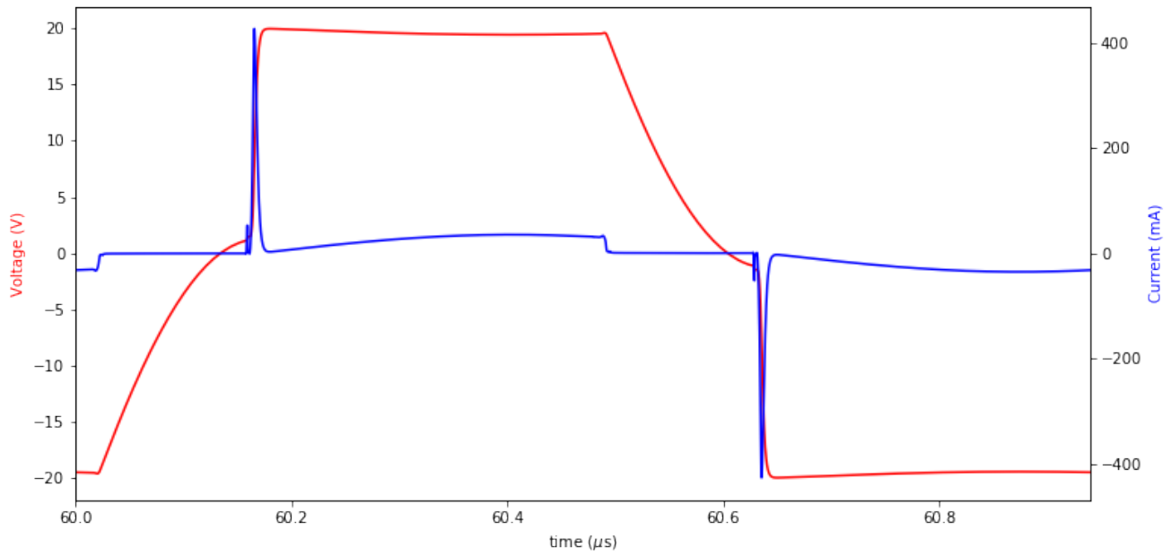
Figure 6.1: Output Voltage and Current of transducer 1
