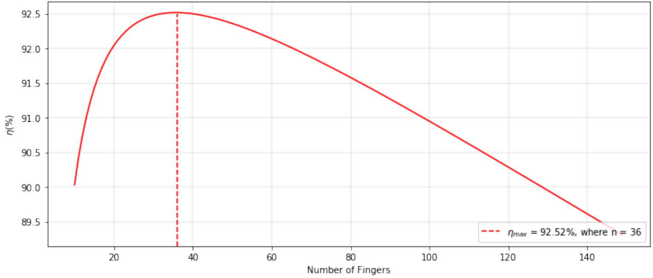
Figure 4.20: Power efficiency vs number of fingers for transducer array used in section 3.3
