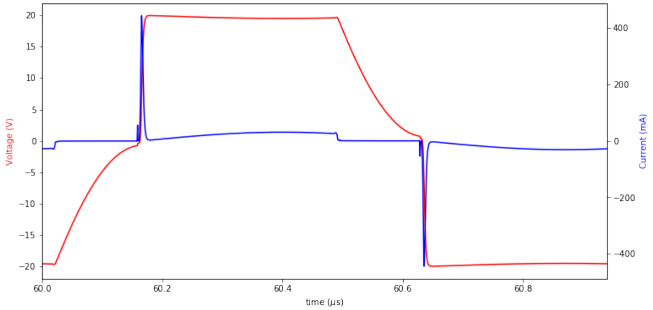
Figure 6.3: Output Voltage and Current of transducer 3
