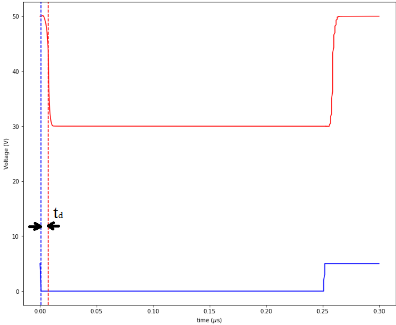
Figure 4.17: Close up view of the level shifter output waveform
