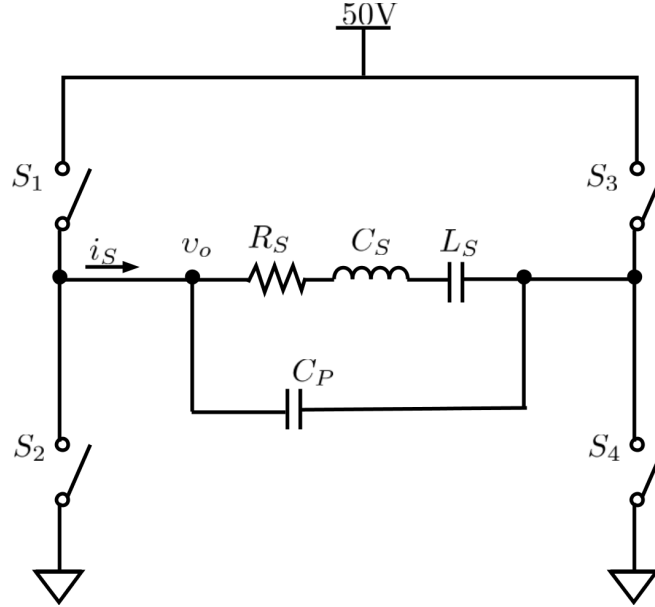
Figure 4.19: Simplified class DE amplifier in full bridge configuration
