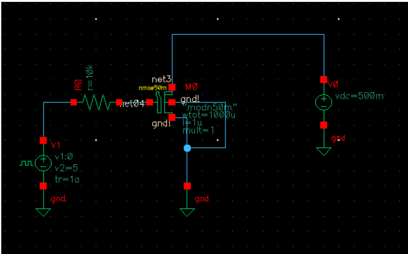
Figure 8.1: Circuit setup to find the gate capacitance
