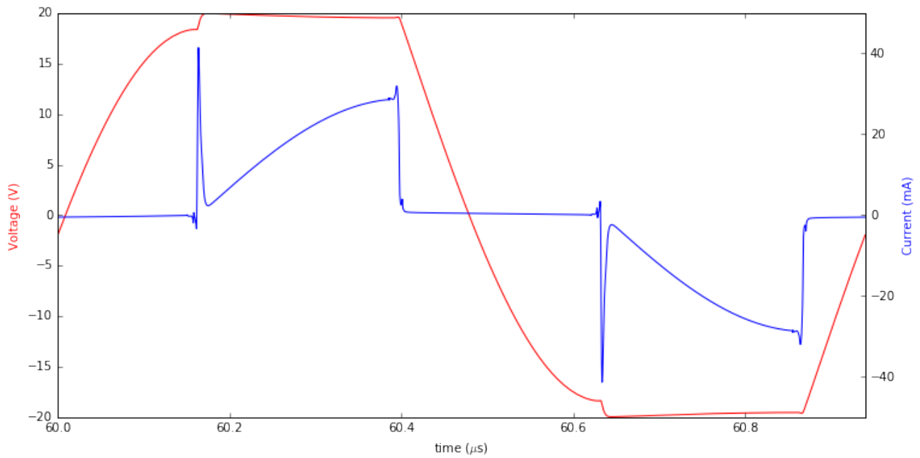
Figure 6.2: Output Voltage and Current of transducer 2
