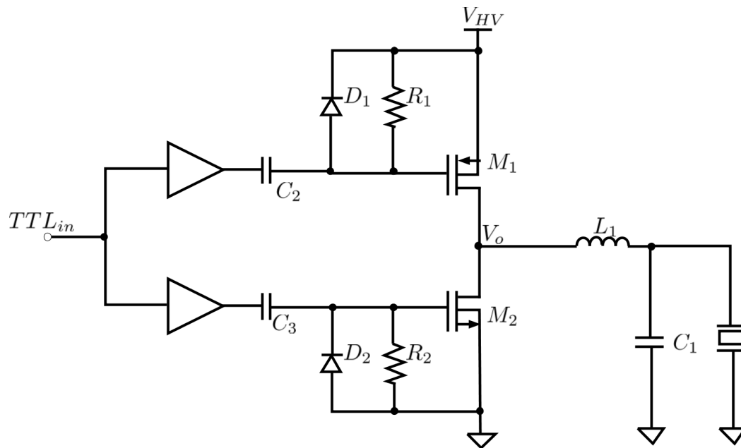
Figure 2.7: Schematic of the transducer driver proposed by Hall and Cain
