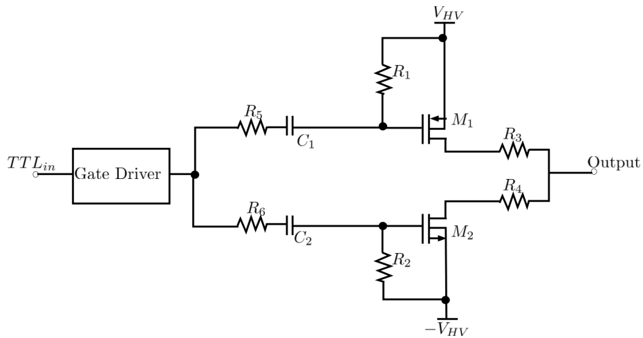
Figure 2.10: Schematic of the switched-mode amplifier proposed by Lewis and Olbricht [21]
