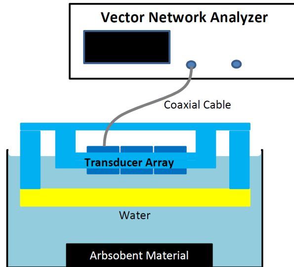
Figure 2.3: Measuring the impedance of the transducers
