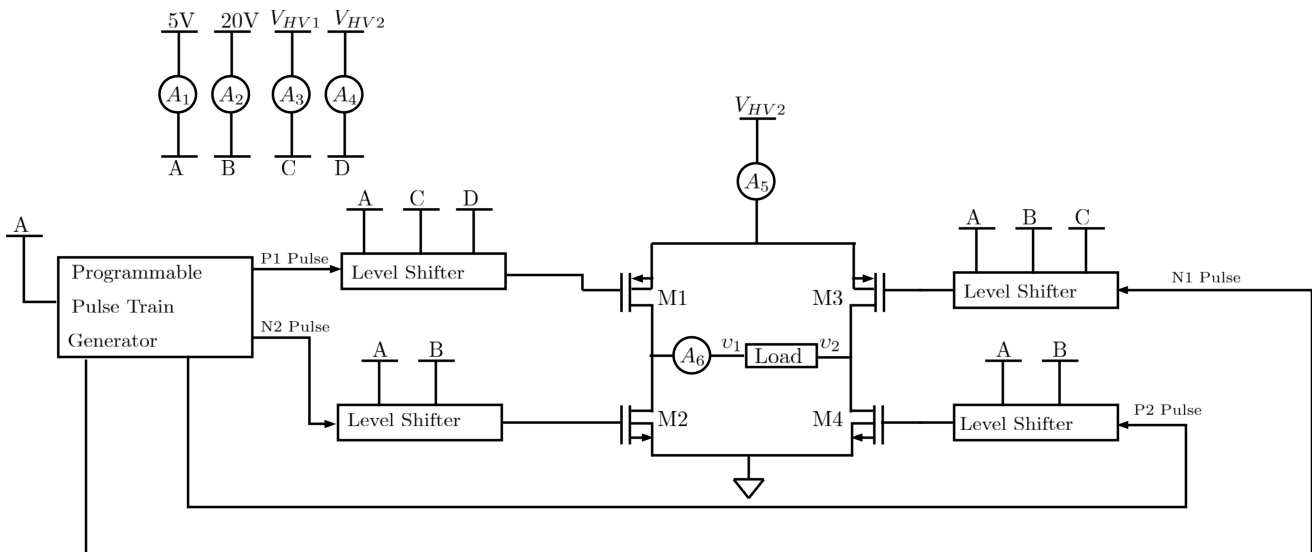
Figure 4.27: Simulation setup
