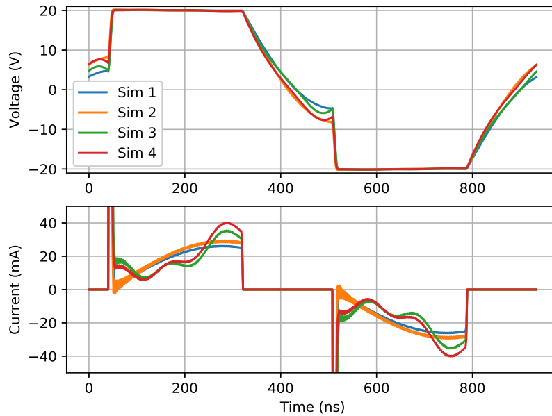
Figure 3.6: Trans 3 output voltage and current
