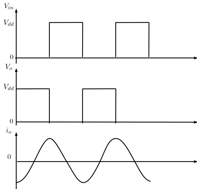
Figure 2.6: Waveforms of class D amplifier [14]
