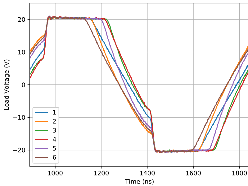
Figure 3.9: Experimental output voltage for all transducers.
