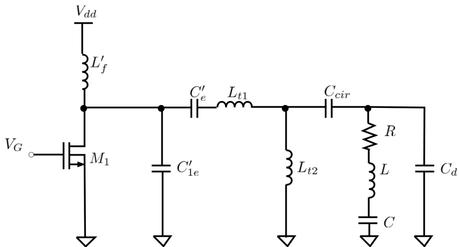
Figure 2.15: Yuan's class E Amplifier Design [10]
