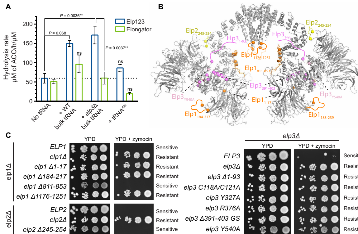
Fig. 5. Functional validation of Elp123. (A) Mean acetyl-CoA (ACO) hydrolysis rate of endogenous ScElp123 (blue) and recombinant Elongator (green) in the presence of different tRNAs. Statistical significance was determined by ordinary two-way analysis of variance (ANOVA; \alpha = 0.05 ) followed by Tukey's honestly significant difference test applied to the entire dataset. ns, not significantly different from the protein samples without tRNA (horizontal dotted line); **P < 0.01 ; mean \pm SEM; n = 3 ; in the case of elp3Δ bulk tRNA, n = 6 . (B) Structural overview of all mutations, truncations, and deletions tested in yeast. (C) Phenotypic analyses of various yeast strains carrying variations in Elp1, Elp2, and Elp3 using zymocin resistance assays.
